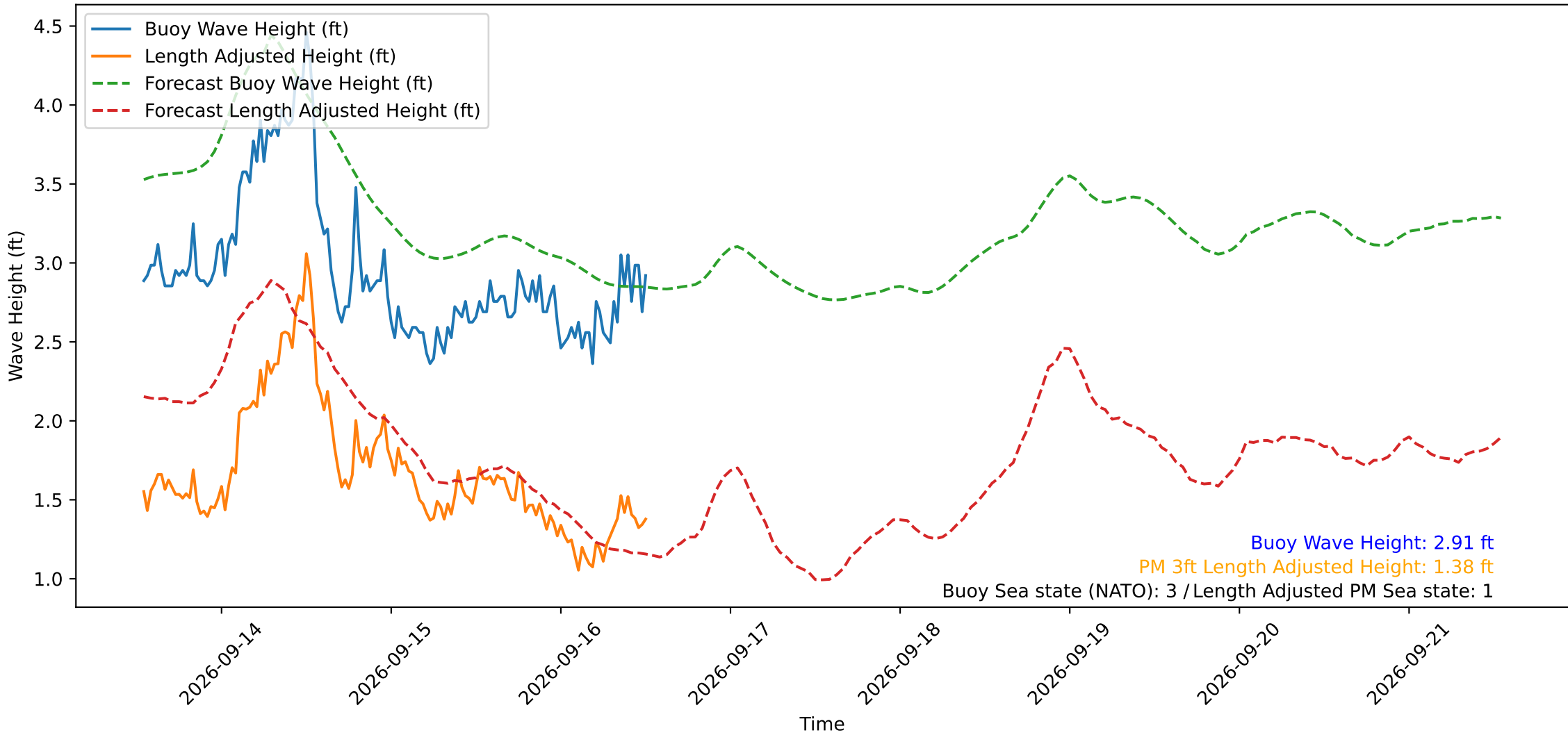
Wave Heights over Time for Oceanside Harbor at 2026-09-16 13:00:29
