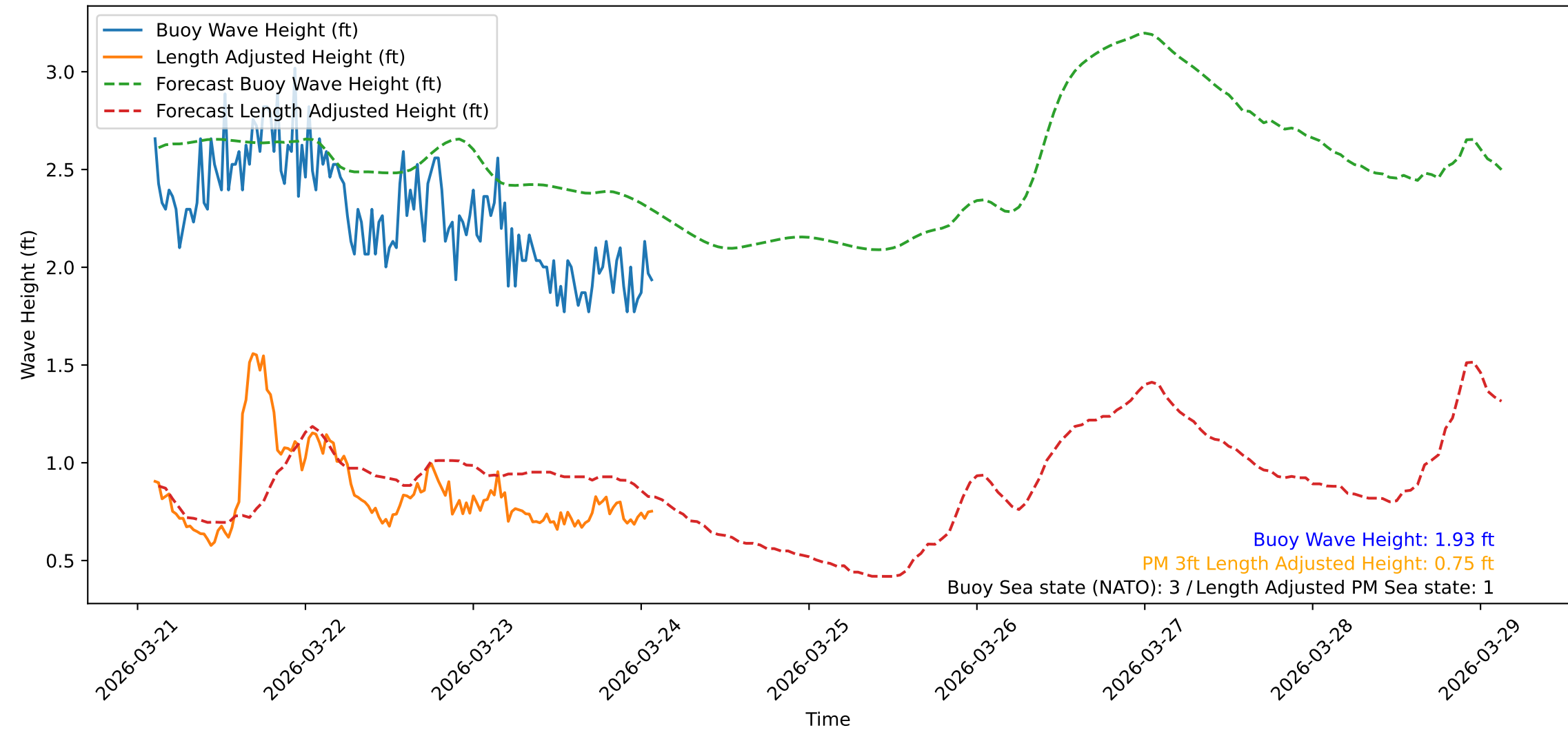
Wave Heights over Time for Oceanside Harbor at 2026-03-24 02:30:31
