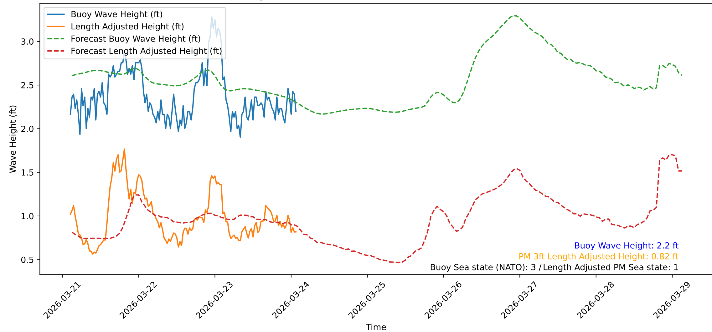
Wave Heights over Time for Green Beach at 2026-03-24 02:31:10
