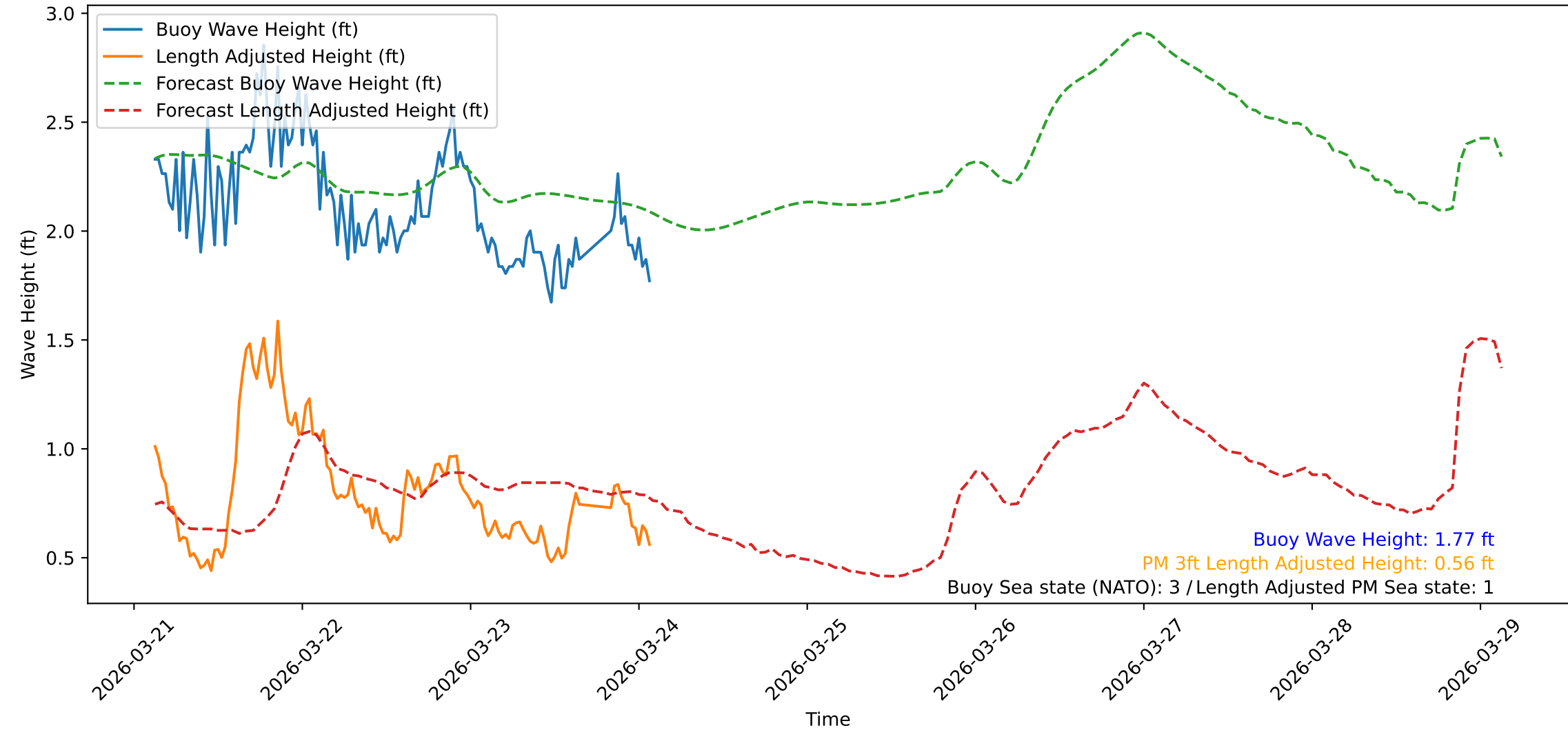
Wave Heights over Time for Red Beach at 2026-03-24 02:30:47
