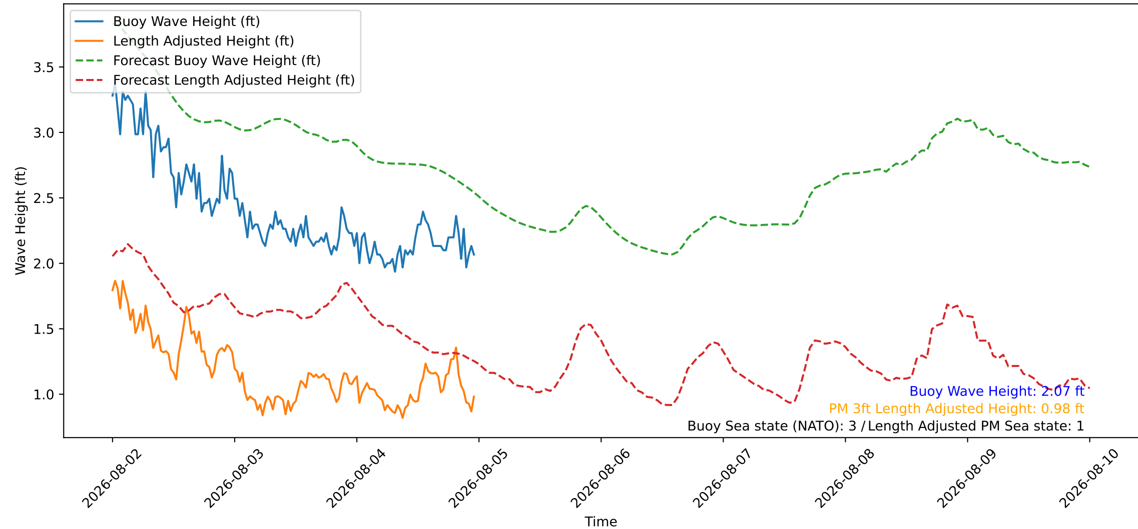
Wave Heights over Time for Green Beach at 2026-08-05 00:01:08
