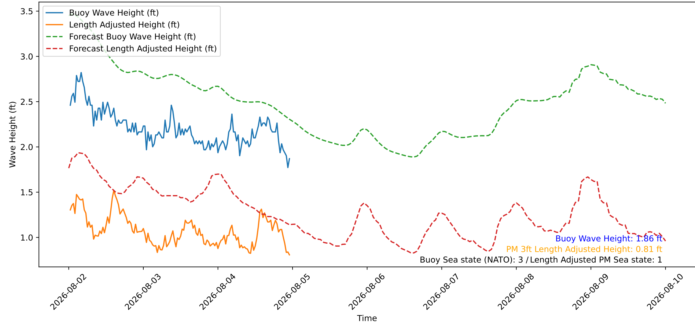
Wave Heights over Time for Red Beach at 2026-08-05 00:00:46
