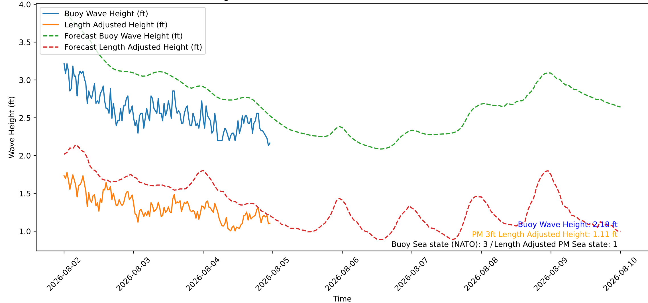
Wave Heights over Time for Oceanside Harbor at 2026-08-05 00:00:27
