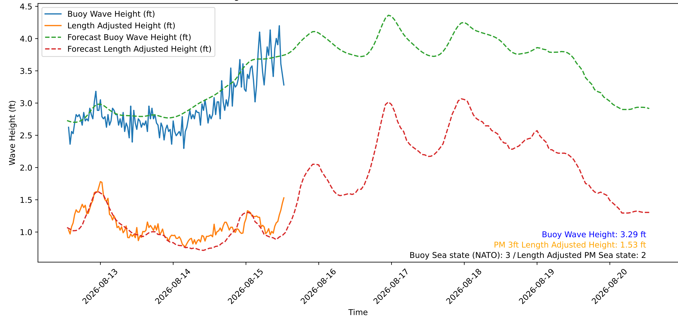
Wave Heights over Time for Oceanside Harbor at 2026-08-15 13:20:26
