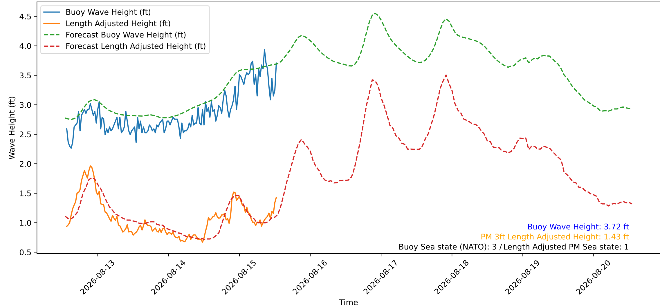
Wave Heights over Time for Green Beach at 2026-08-15 13:21:09
