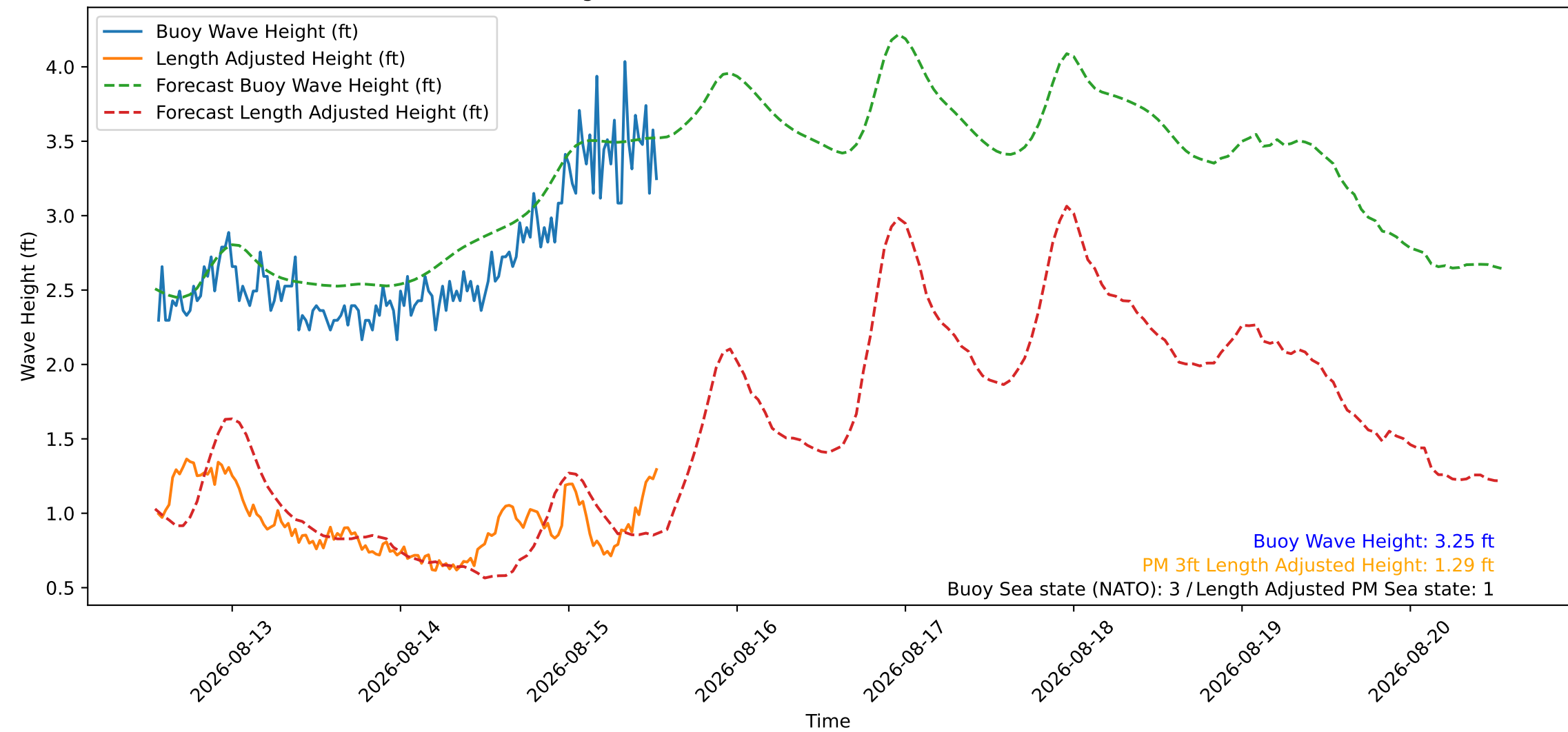
Wave Heights over Time for Red Beach at 2026-08-15 13:20:47
