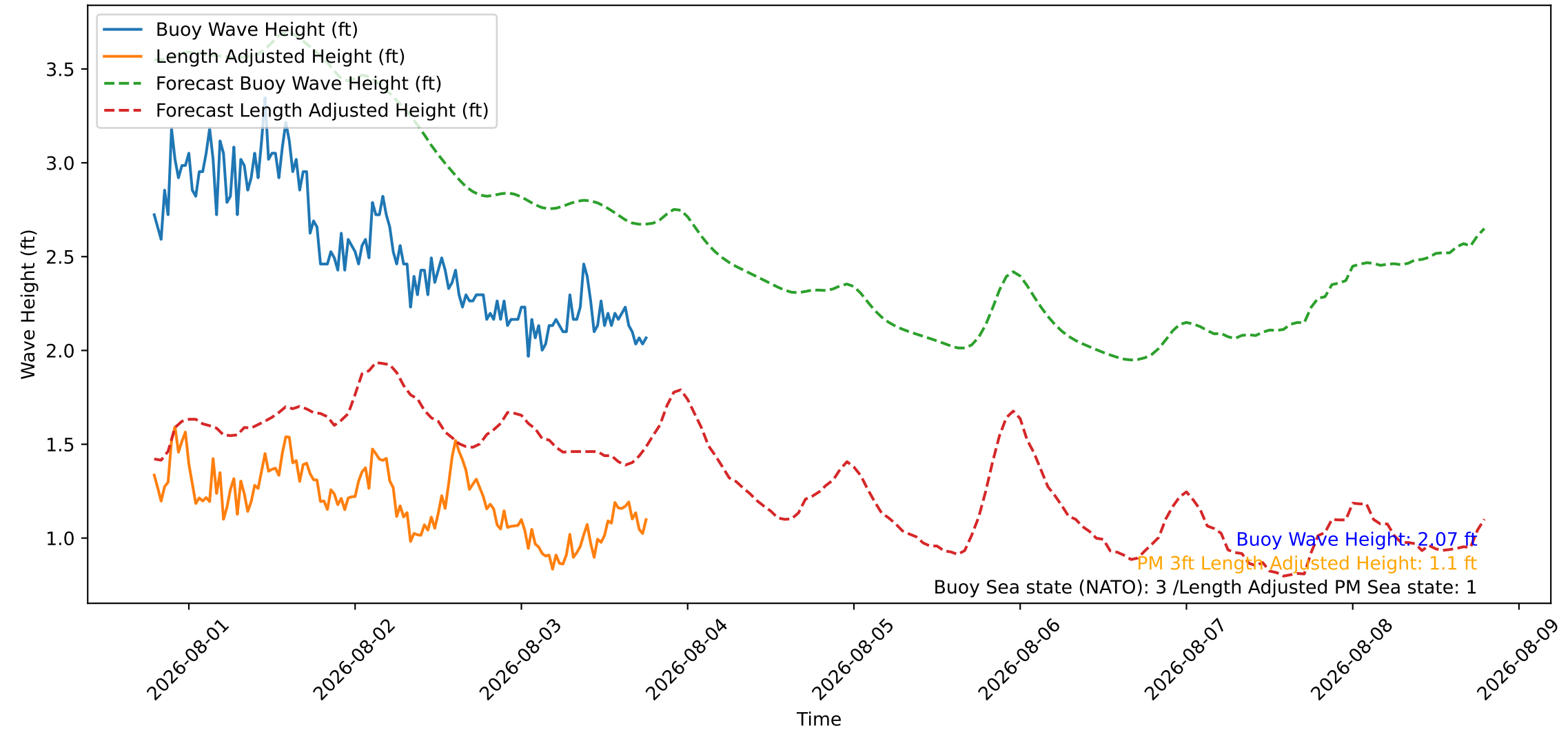
Wave Heights over Time for Red Beach at 2026-08-03 18:50:47
