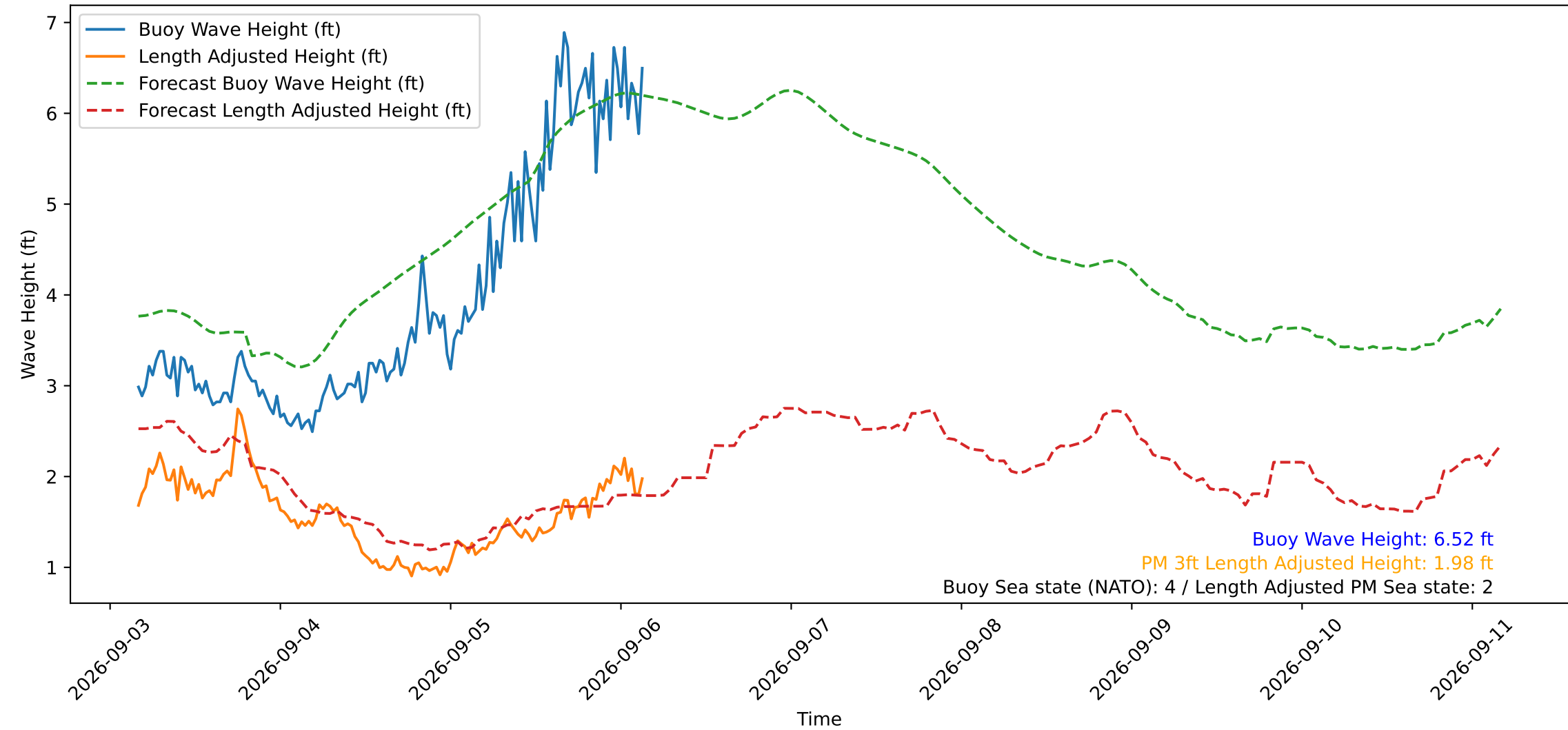
Wave Heights over Time for Green Beach at 2026-09-06 03:41:12
