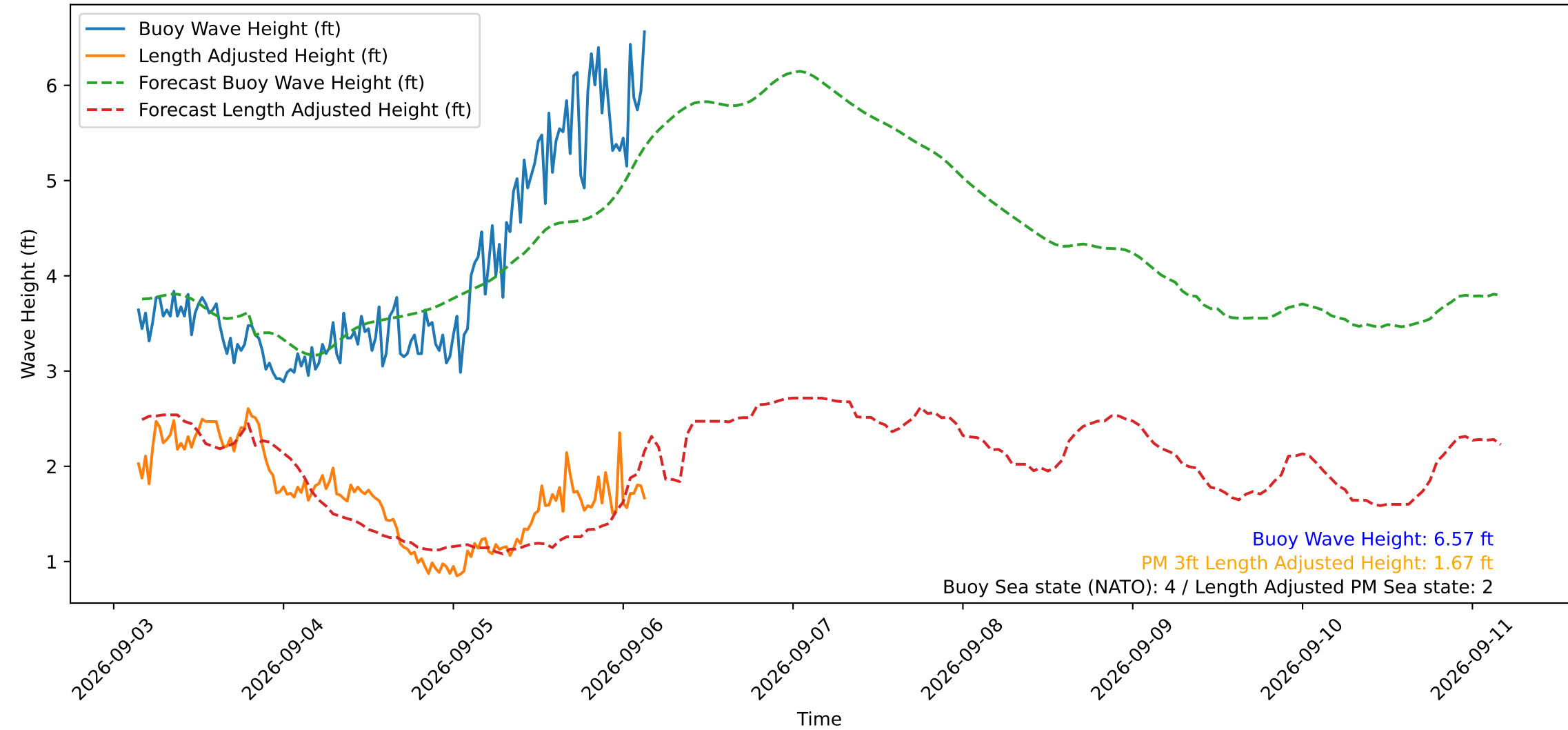
Wave Heights over Time for Oceanside Harbor at 2026-09-06 03:40:29
