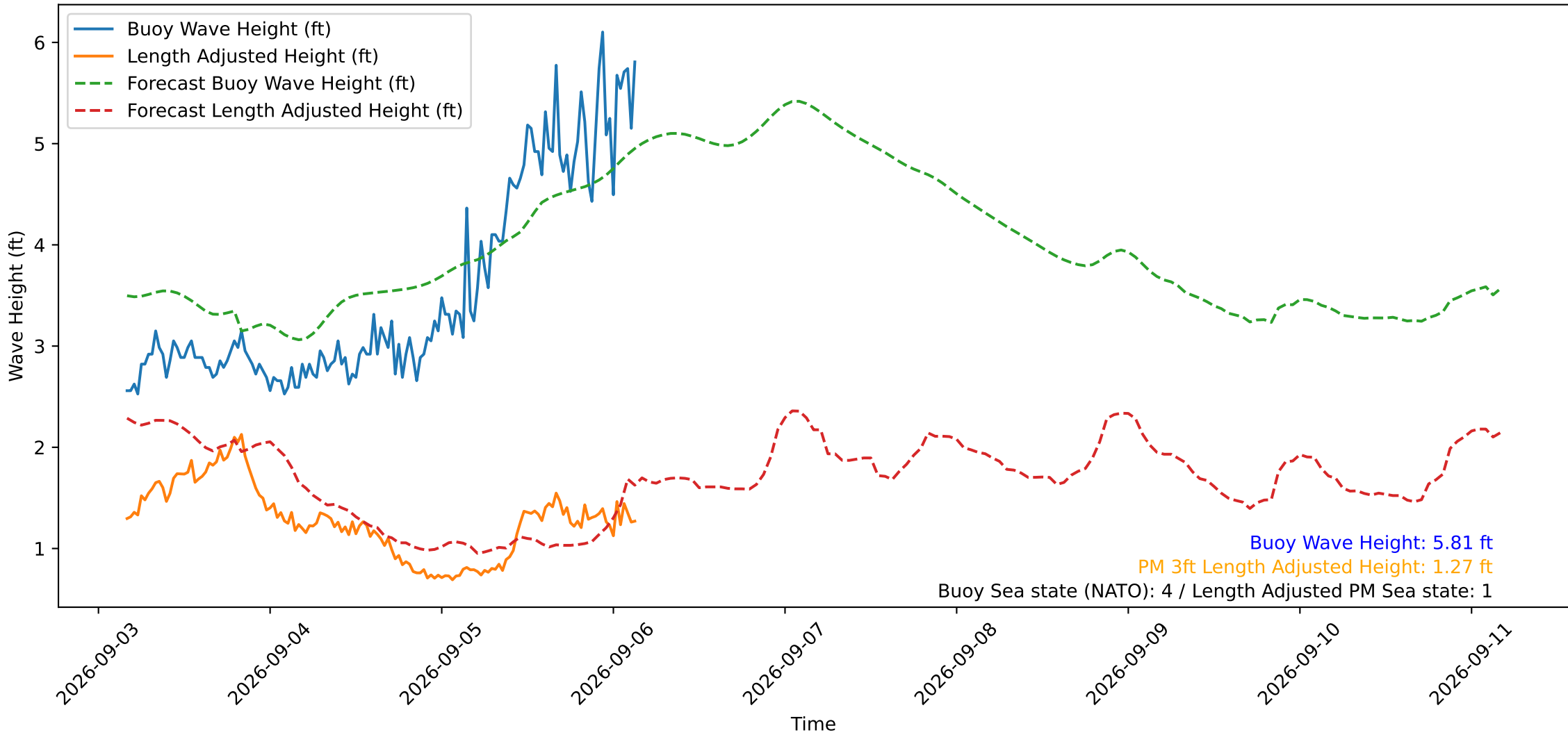
Wave Heights over Time for Red Beach at 2026-09-06 03:40:49
