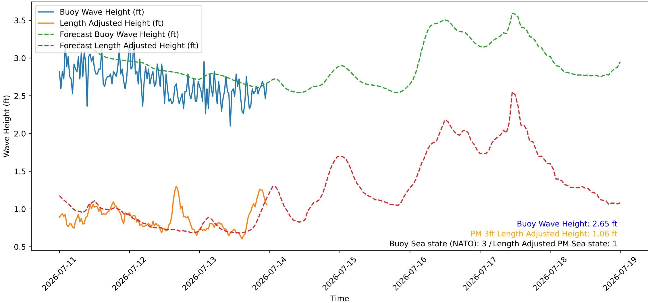
Wave Heights over Time for Oceanside Harbor at 2026-07-13 23:50:26
