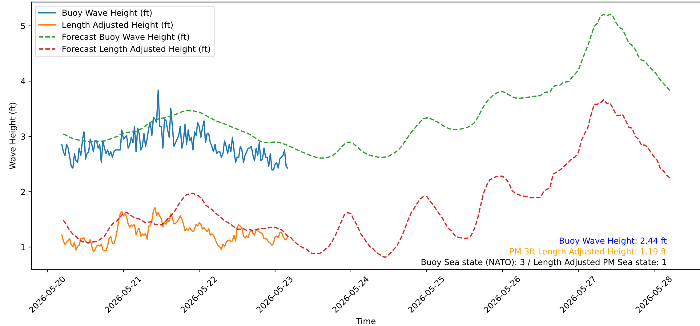
Wave Heights over Time for Oceanside Harbor at 2026-05-23 04:40:32
