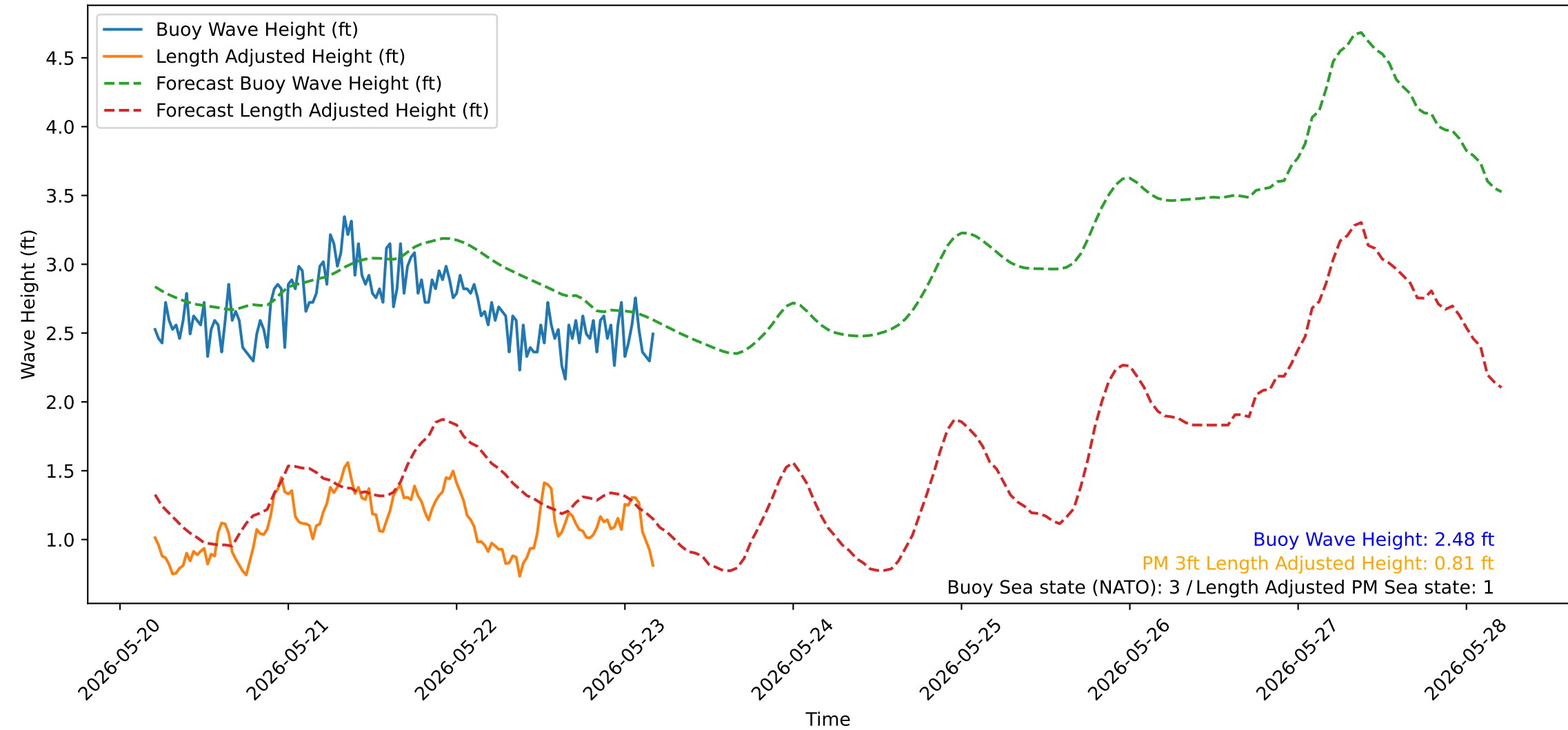
Wave Heights over Time for Red Beach at 2026-05-23 04:40:52
