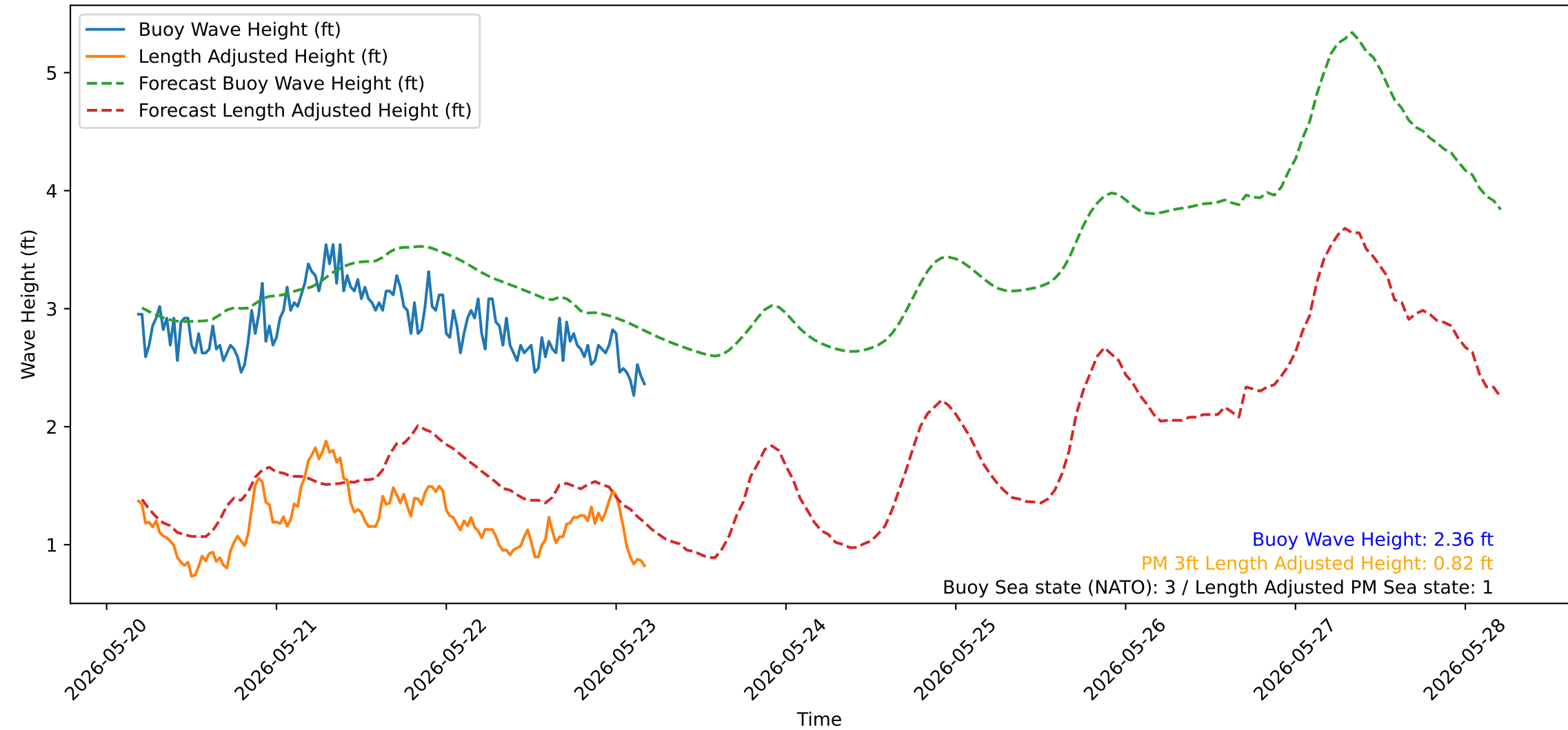
Wave Heights over Time for Green Beach at 2026-05-23 04:41:15
