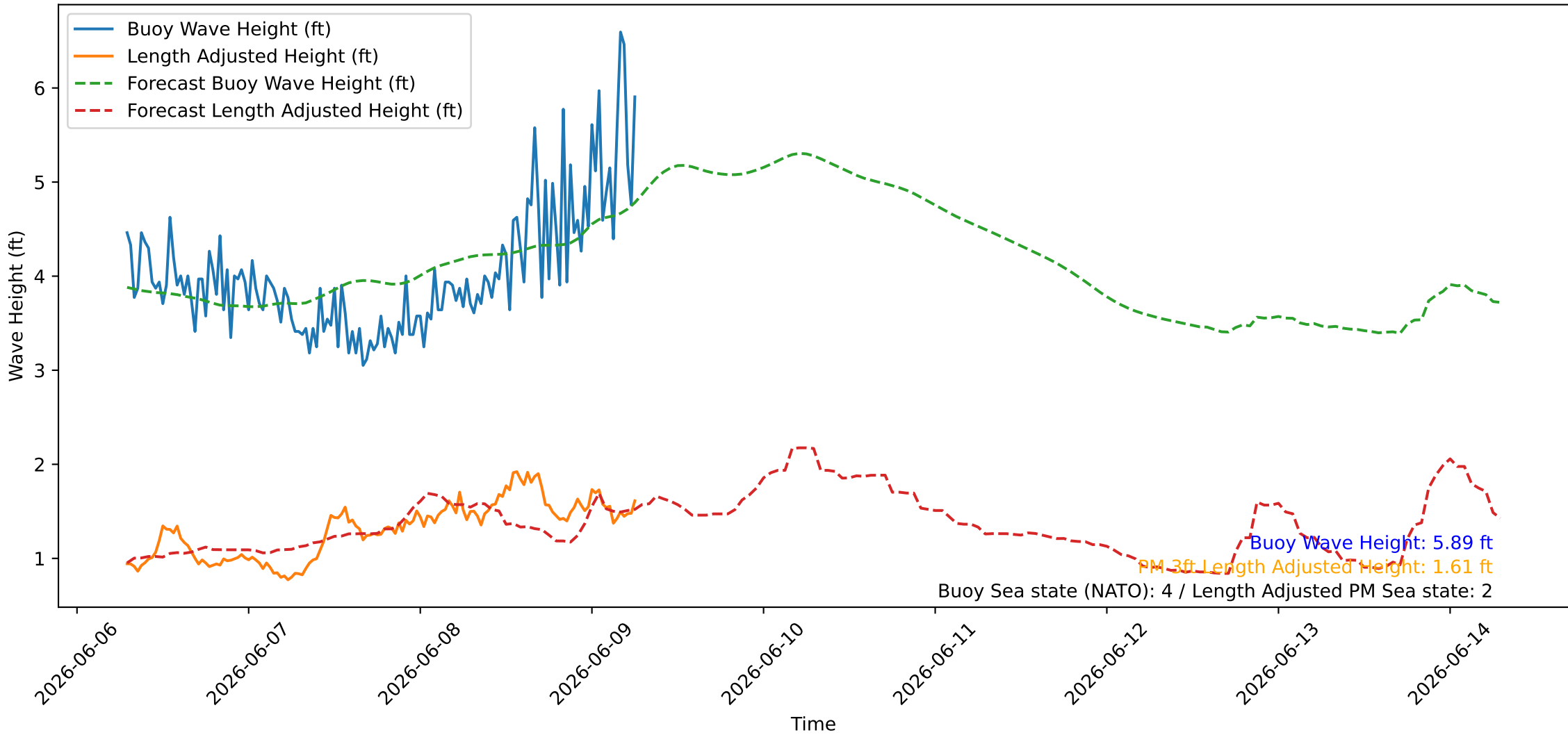
Wave Heights over Time for Red Beach at 2026-06-09 06:50:47
