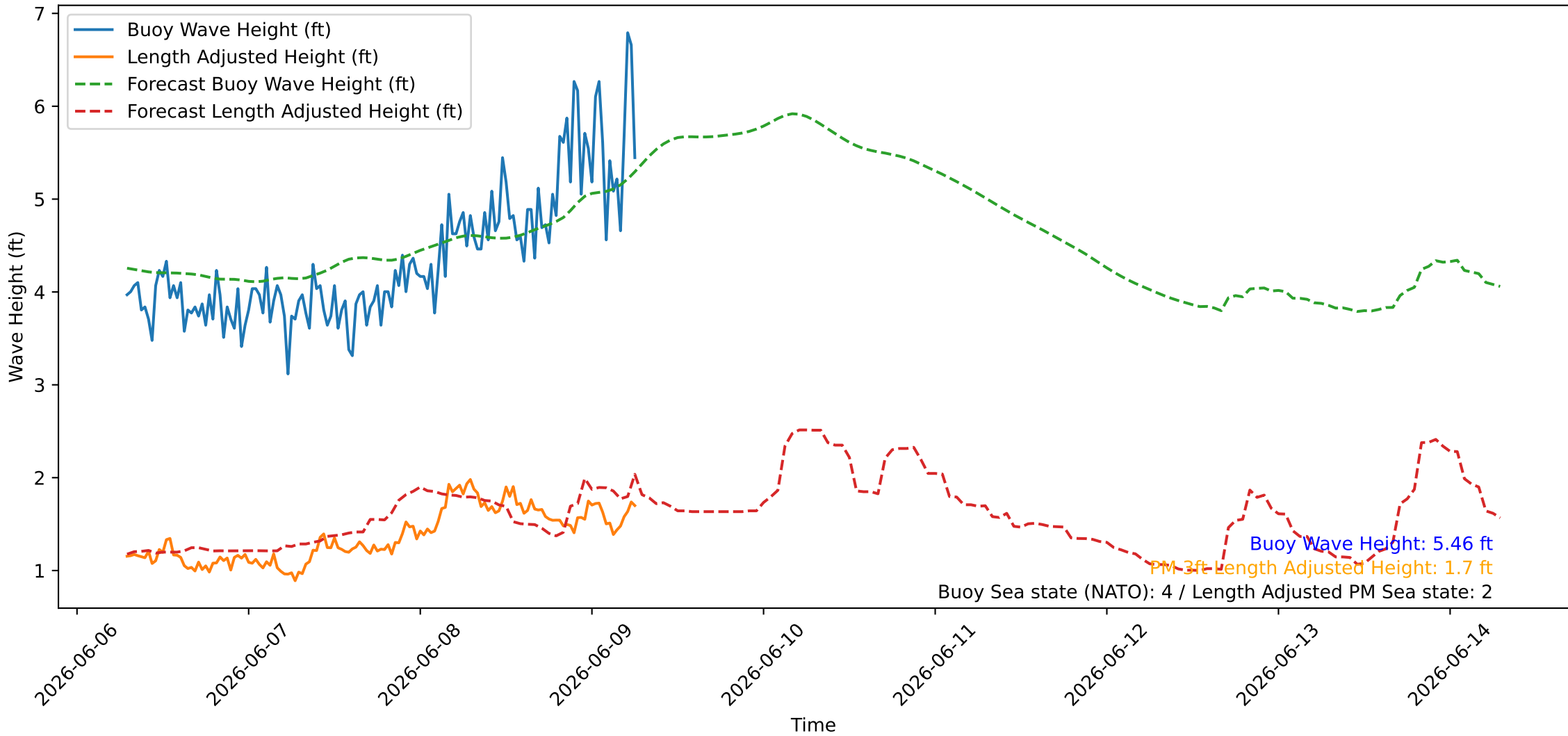
Wave Heights over Time for Green Beach at 2026-06-09 06:51:09
