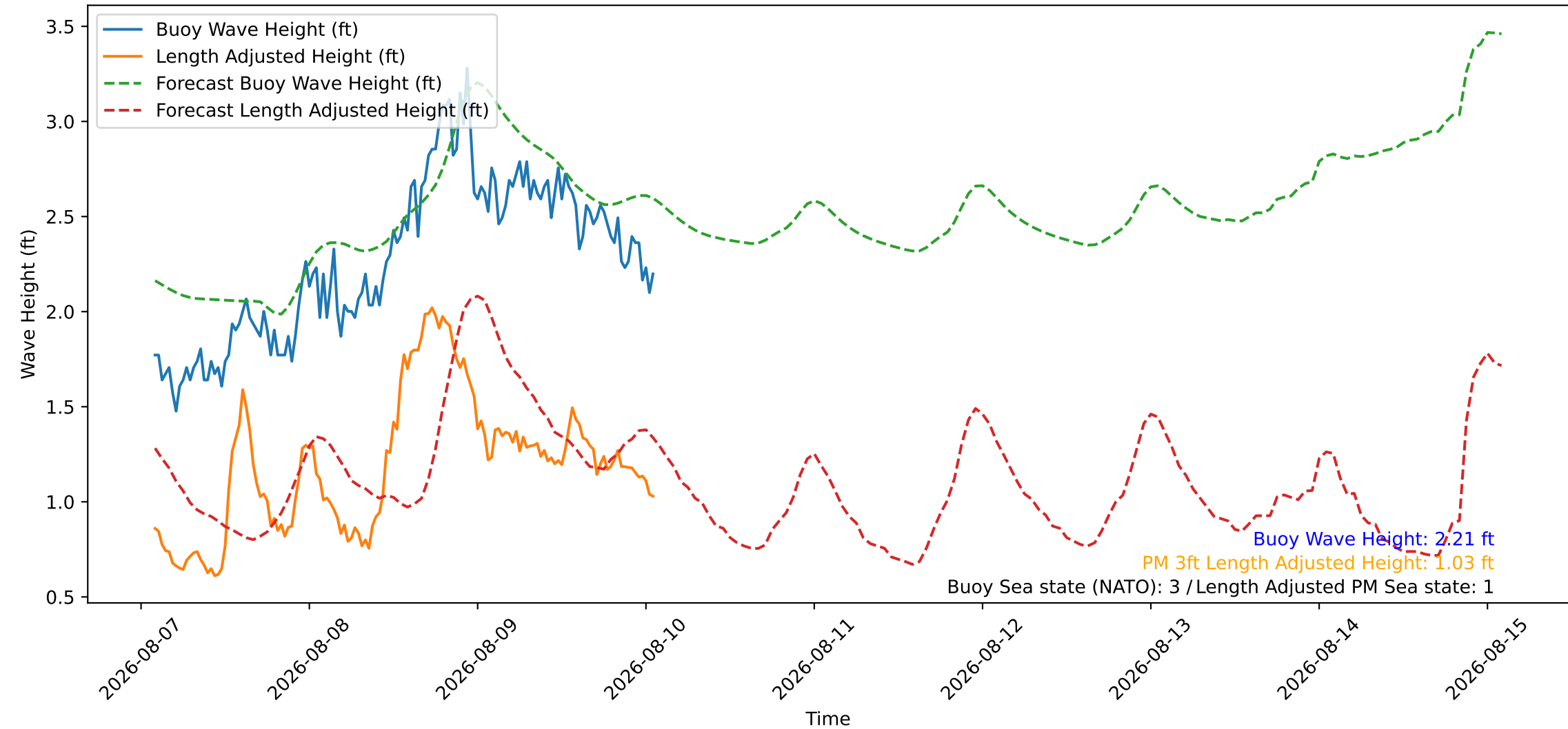
Wave Heights over Time for Red Beach at 2026-08-10 01:50:48
