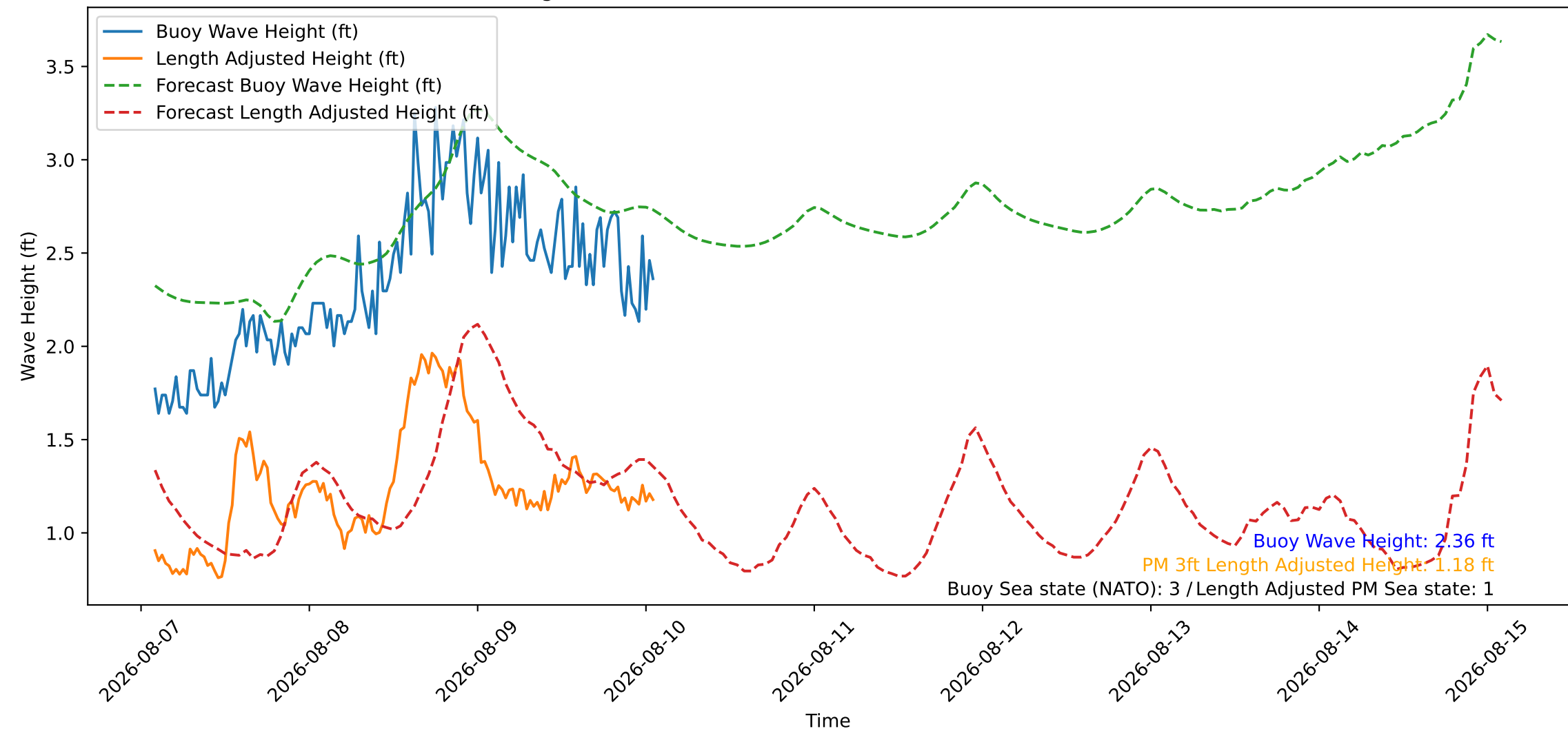
Wave Heights over Time for Oceanside Harbor at 2026-08-10 01:50:27
