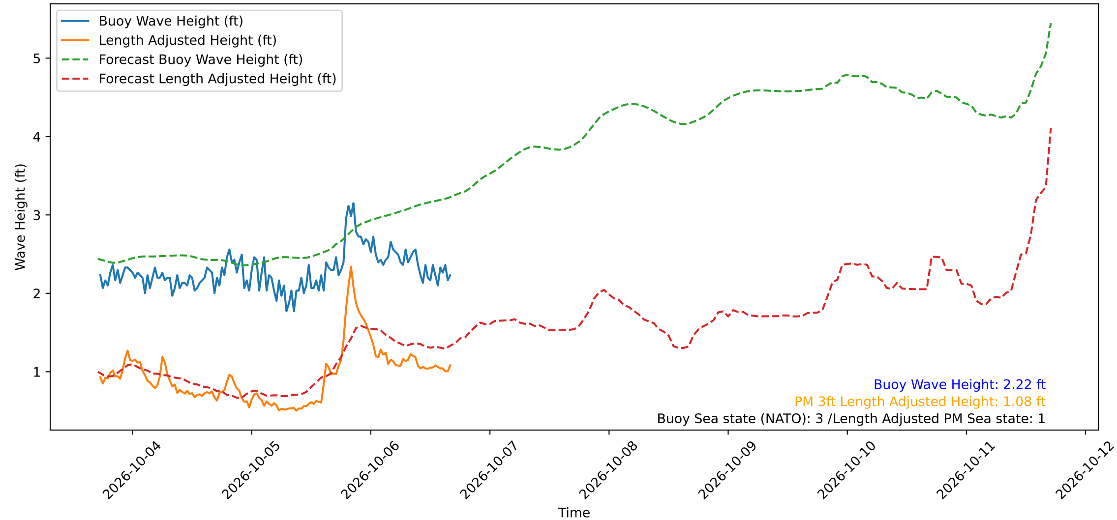
Wave Heights over Time for Green Beach at 2026-10-06 17:01:13
