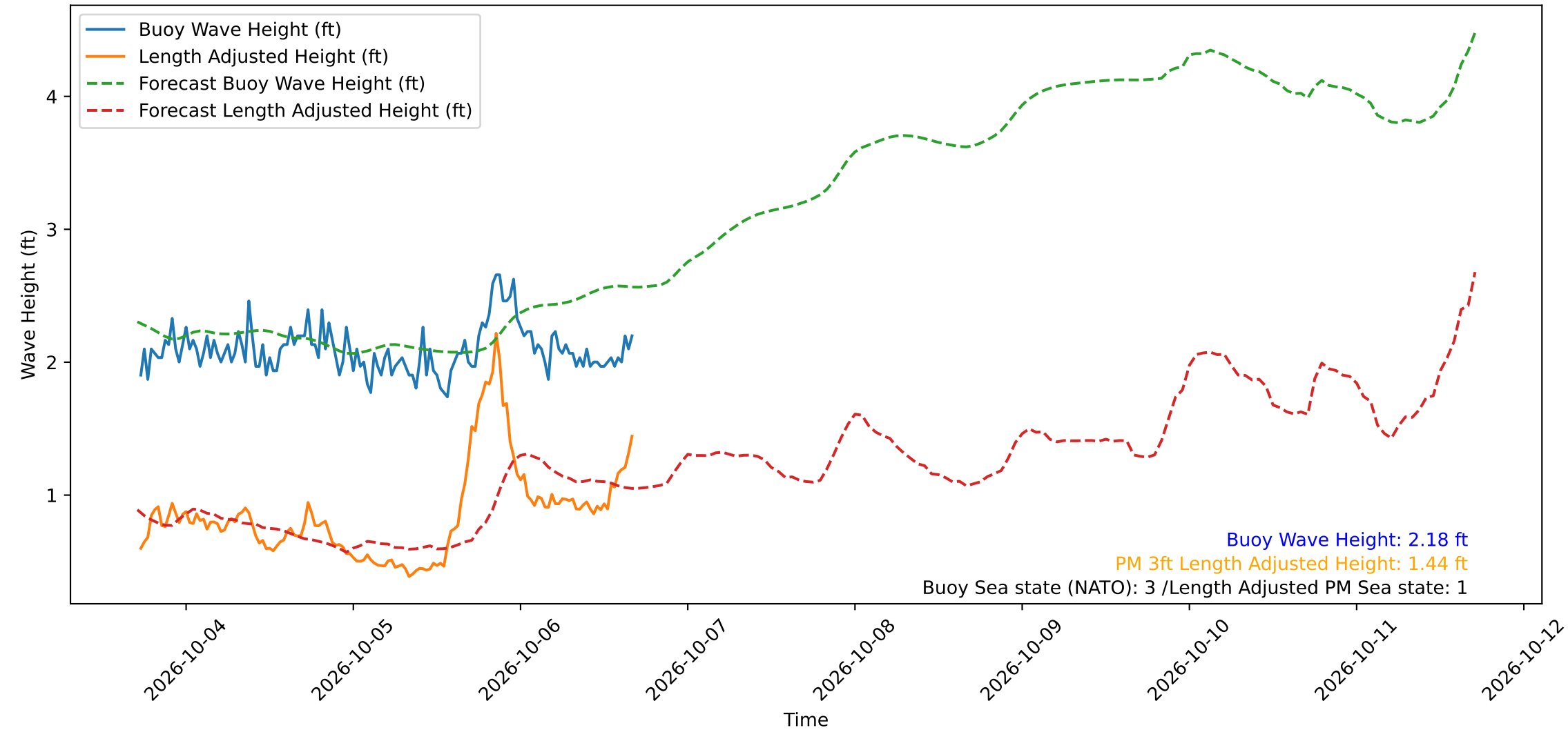
Wave Heights over Time for Red Beach at 2026-10-06 17:00:50
