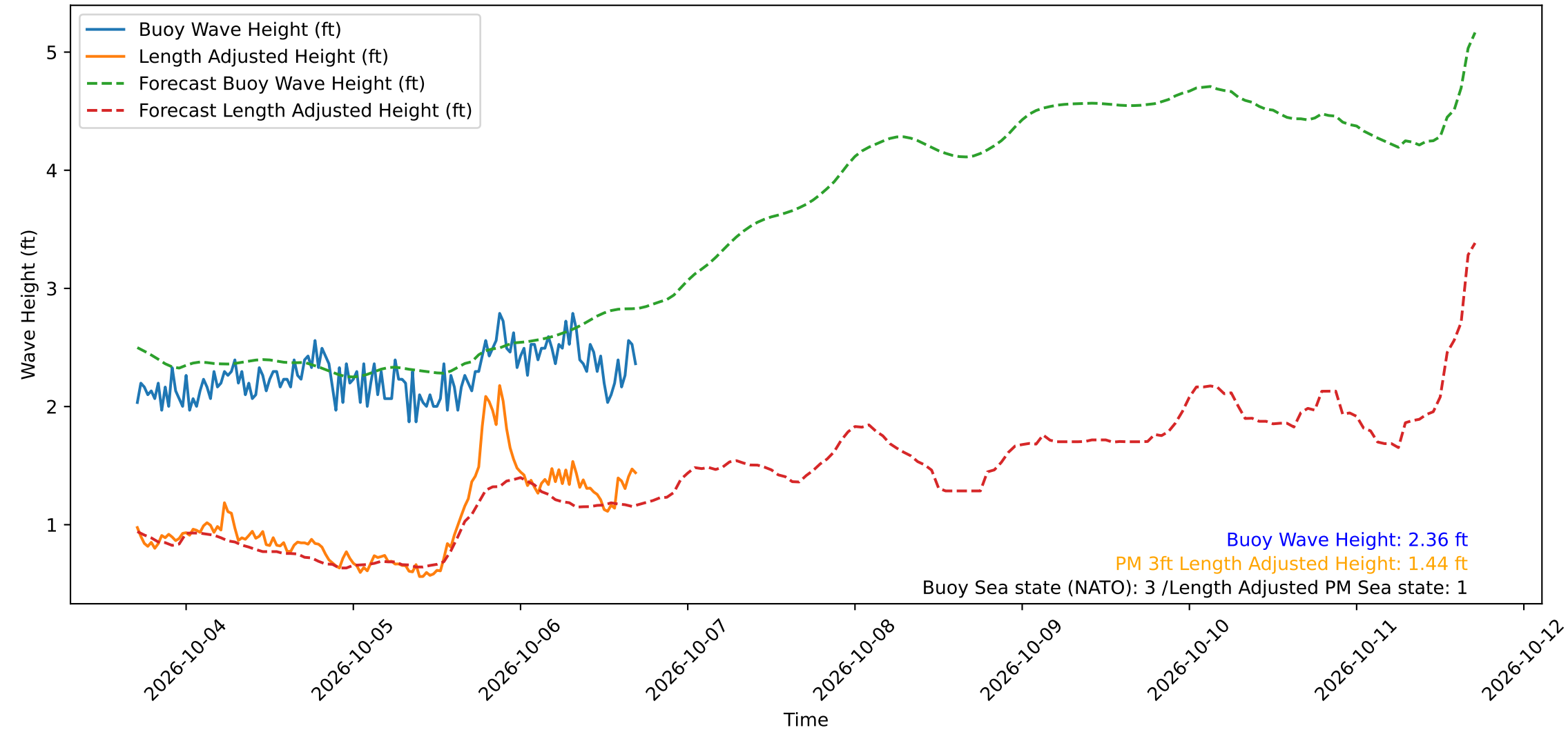
Wave Heights over Time for Oceanside Harbor at 2026-10-06 17:00:30
