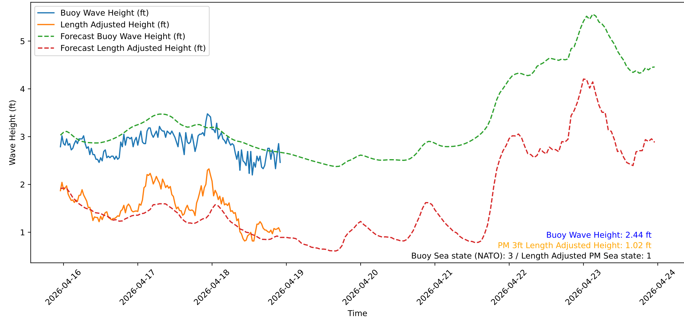
Wave Heights over Time for Green Beach at 2026-04-18 23:01:12
