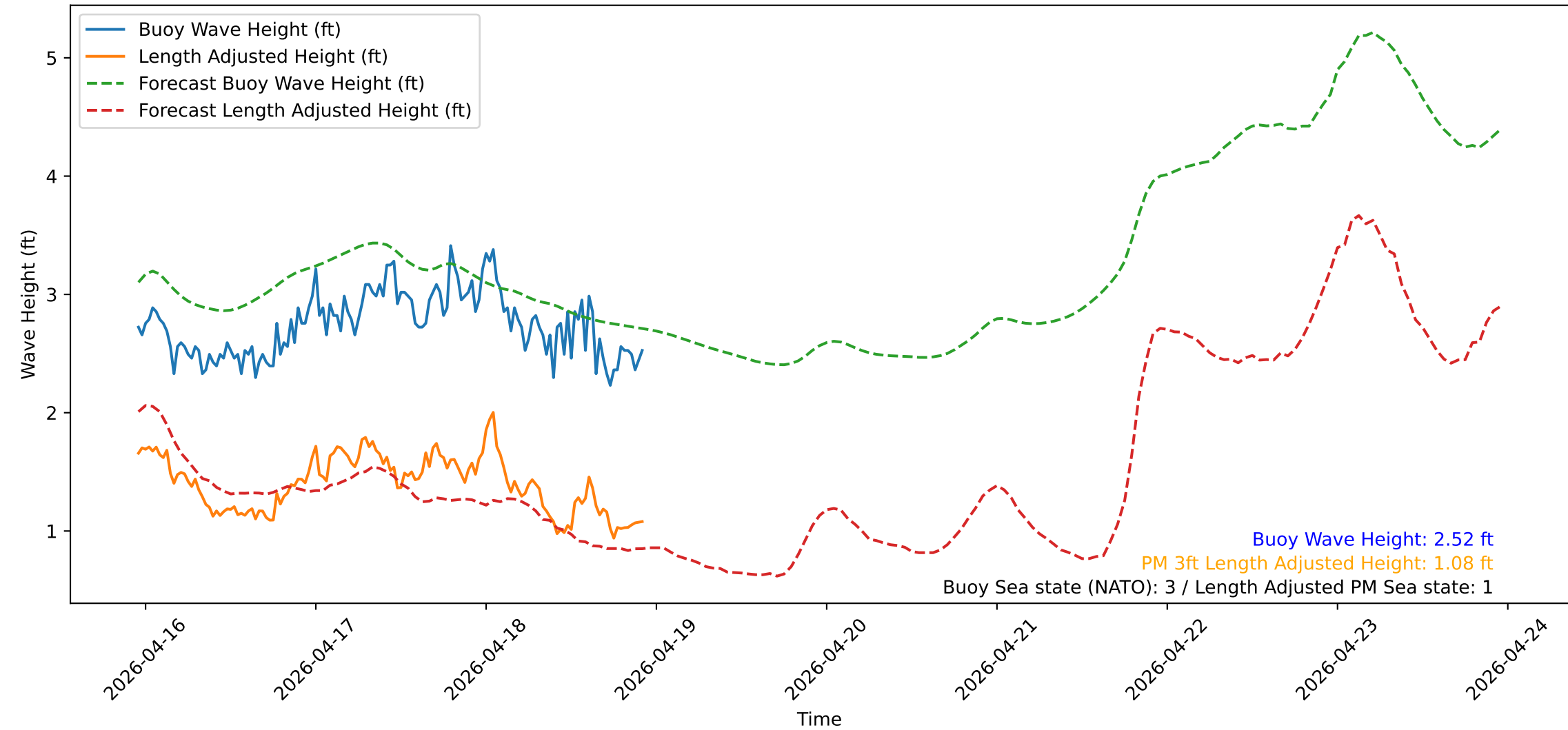
Wave Heights over Time for Oceanside Harbor at 2026-04-18 23:00:31
