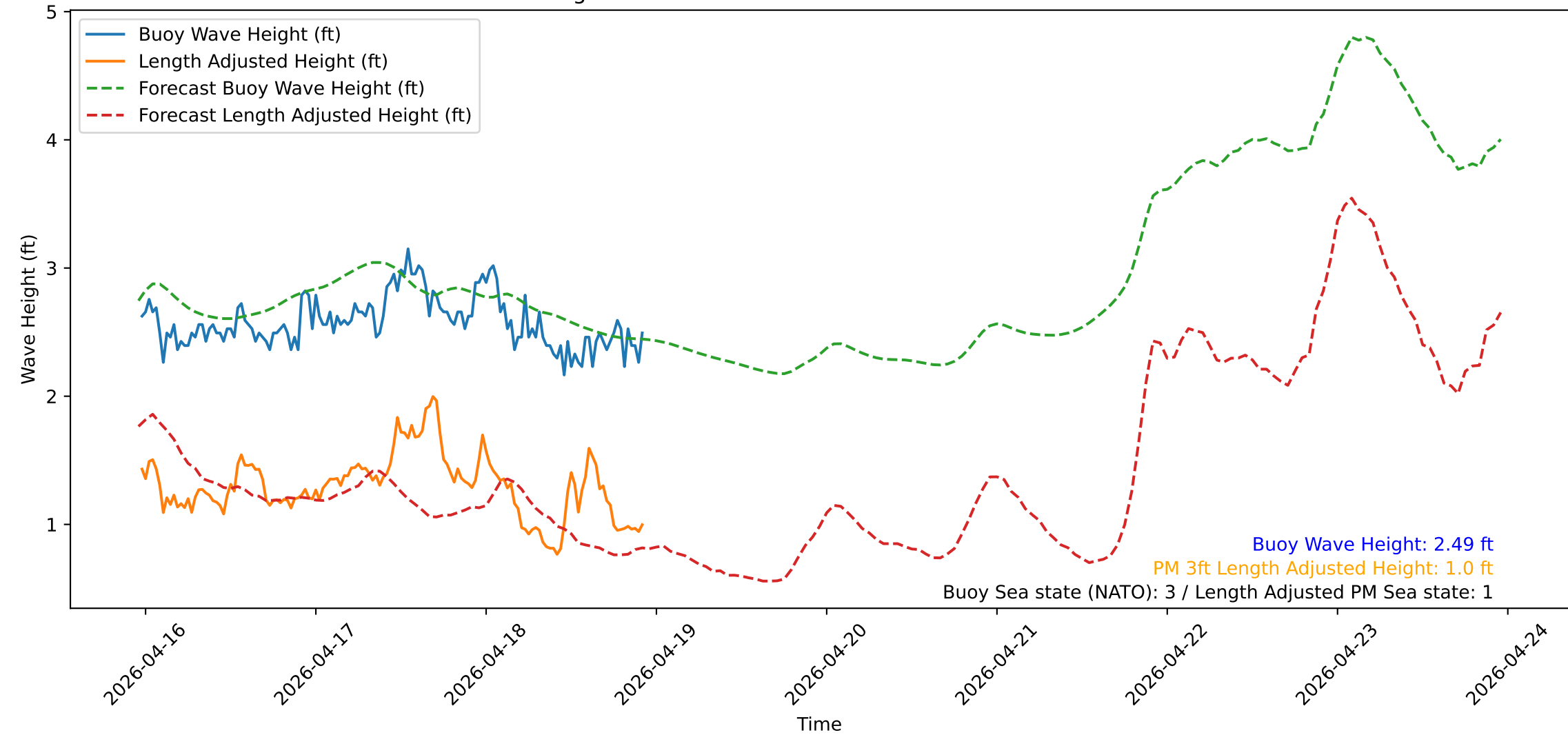
Wave Heights over Time for Red Beach at 2026-04-18 23:00:50
