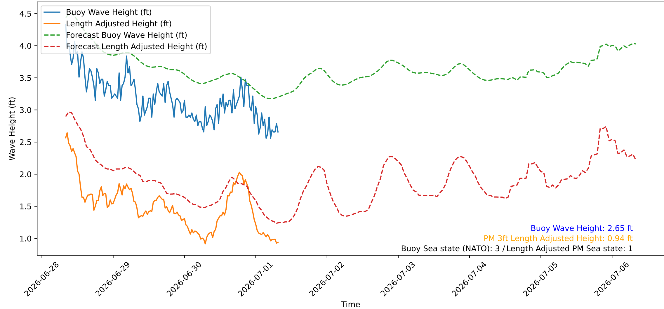
Wave Heights over Time for Green Beach at 2026-07-01 08:11:09
