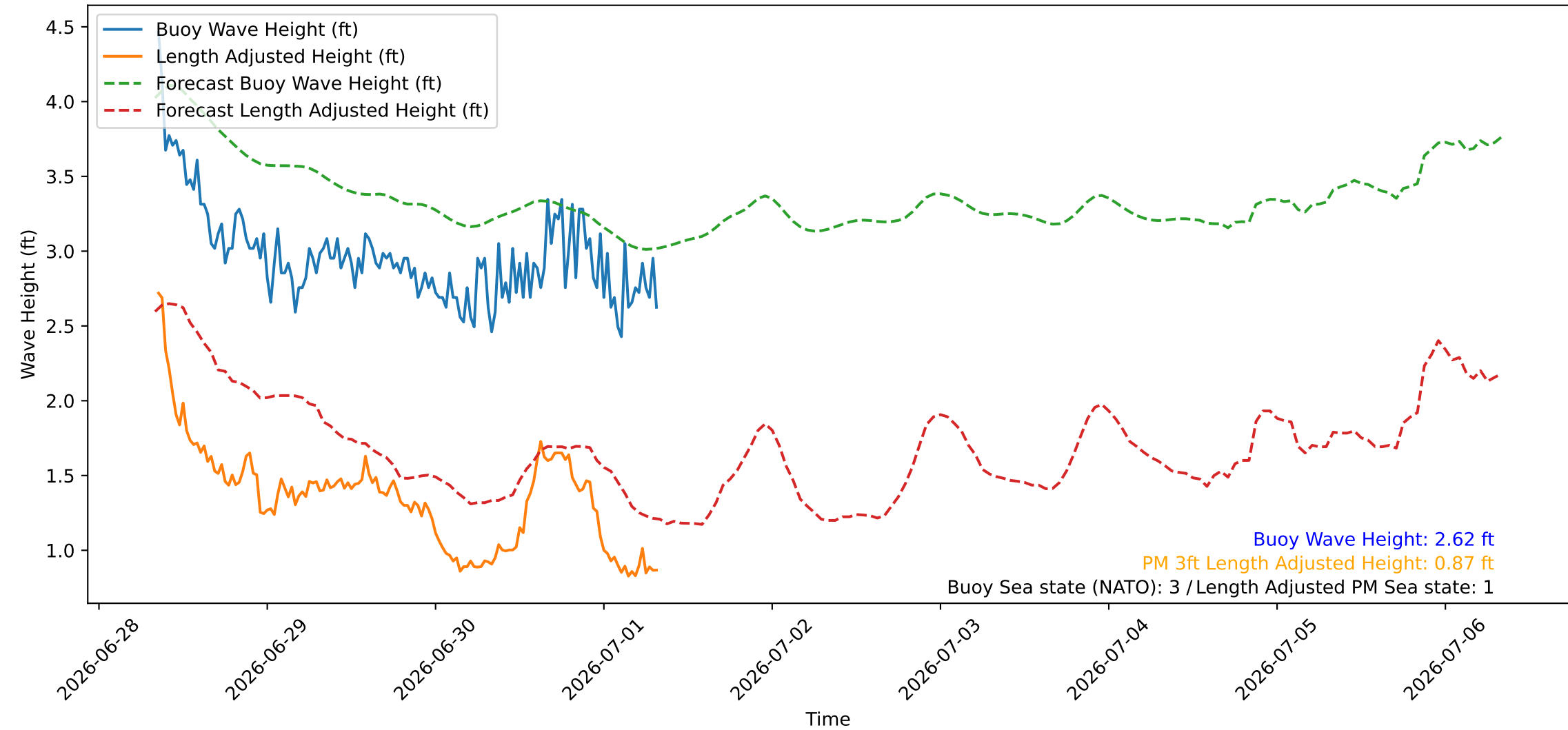
Wave Heights over Time for Red Beach at 2026-07-01 08:10:46
