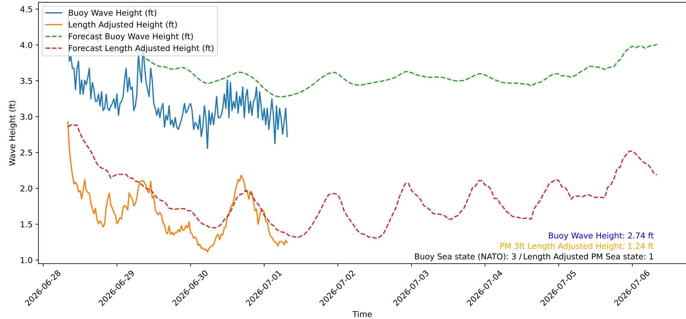
Wave Heights over Time for Oceanside Harbor at 2026-07-01 08:10:27
