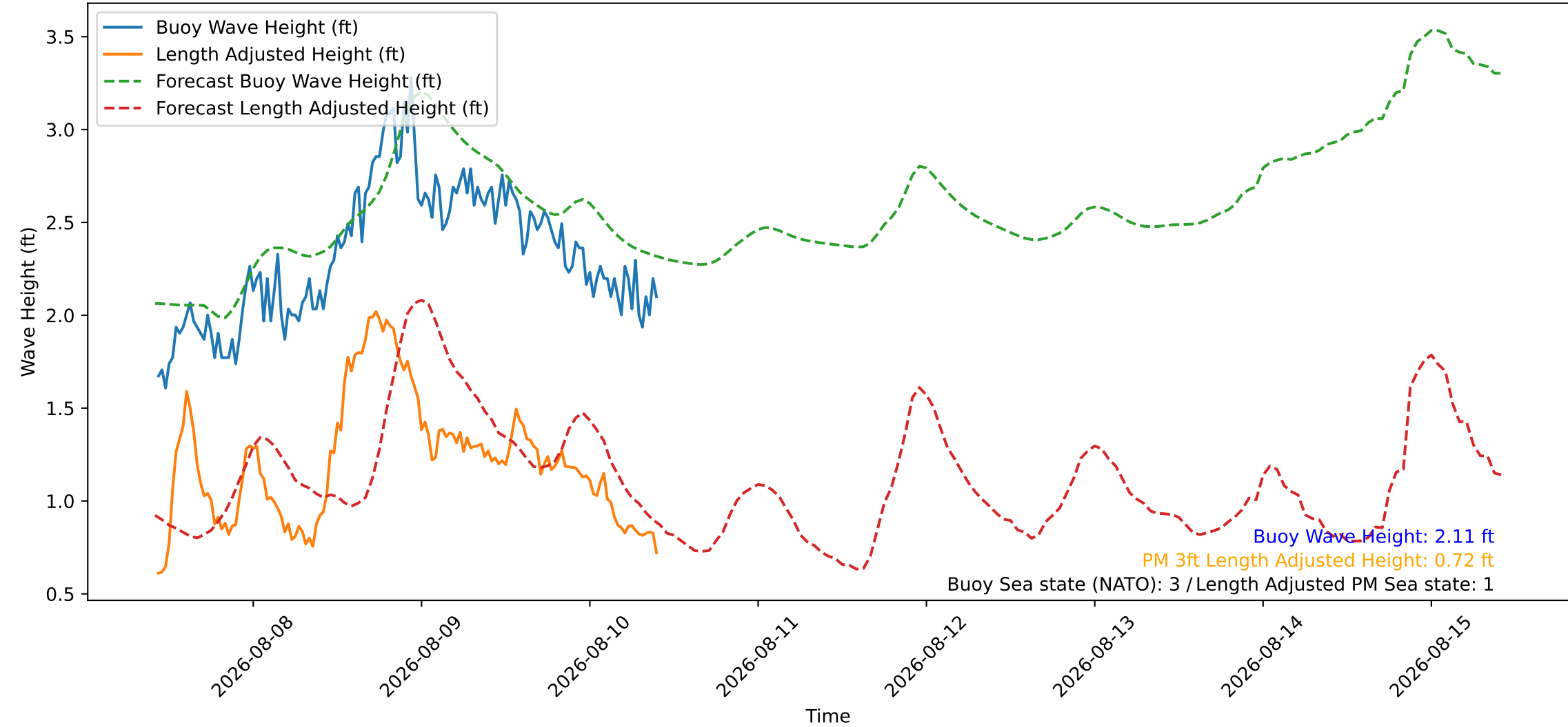
Wave Heights over Time for Red Beach at 2026-08-10 10:20:47
