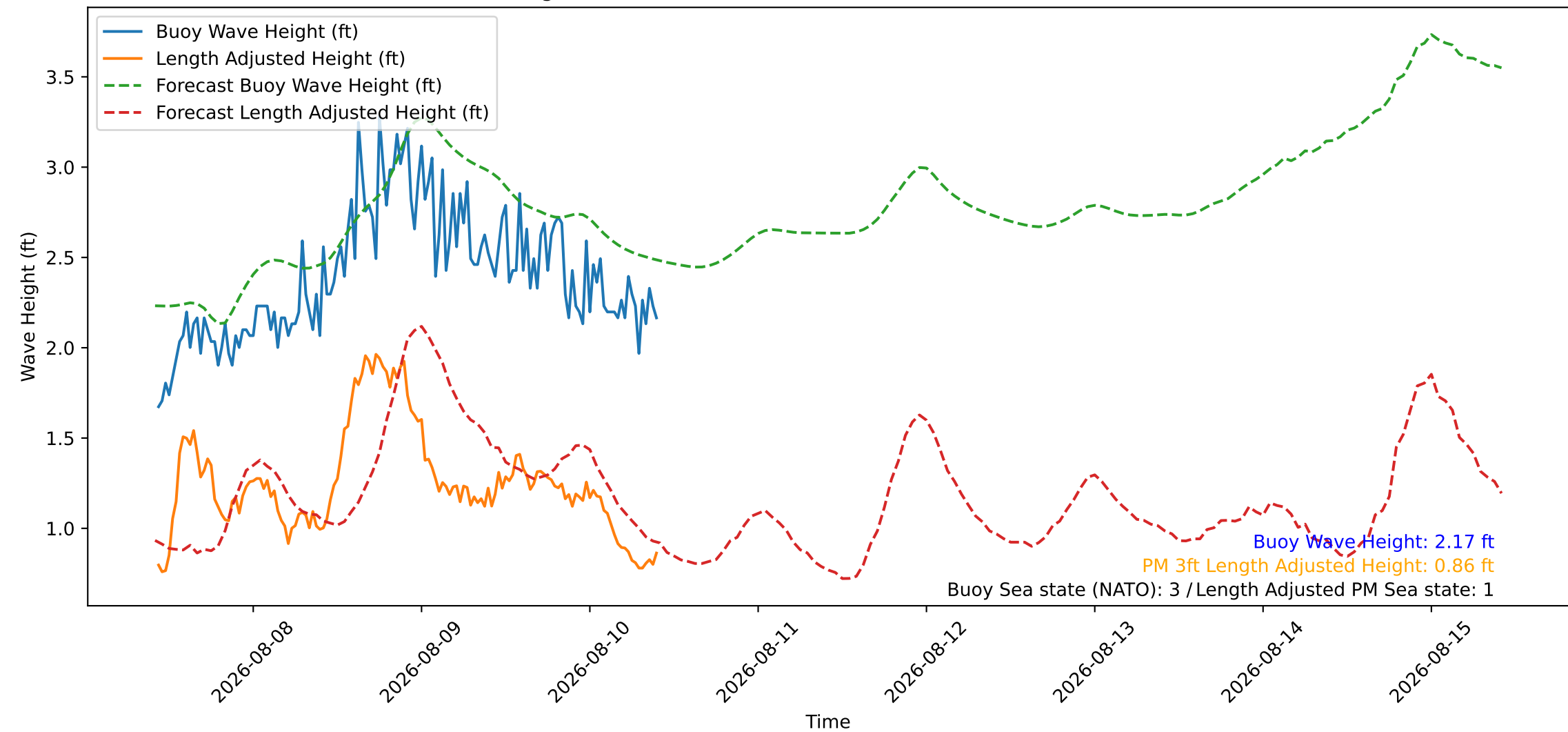
Wave Heights over Time for Oceanside Harbor at 2026-08-10 10:20:27
