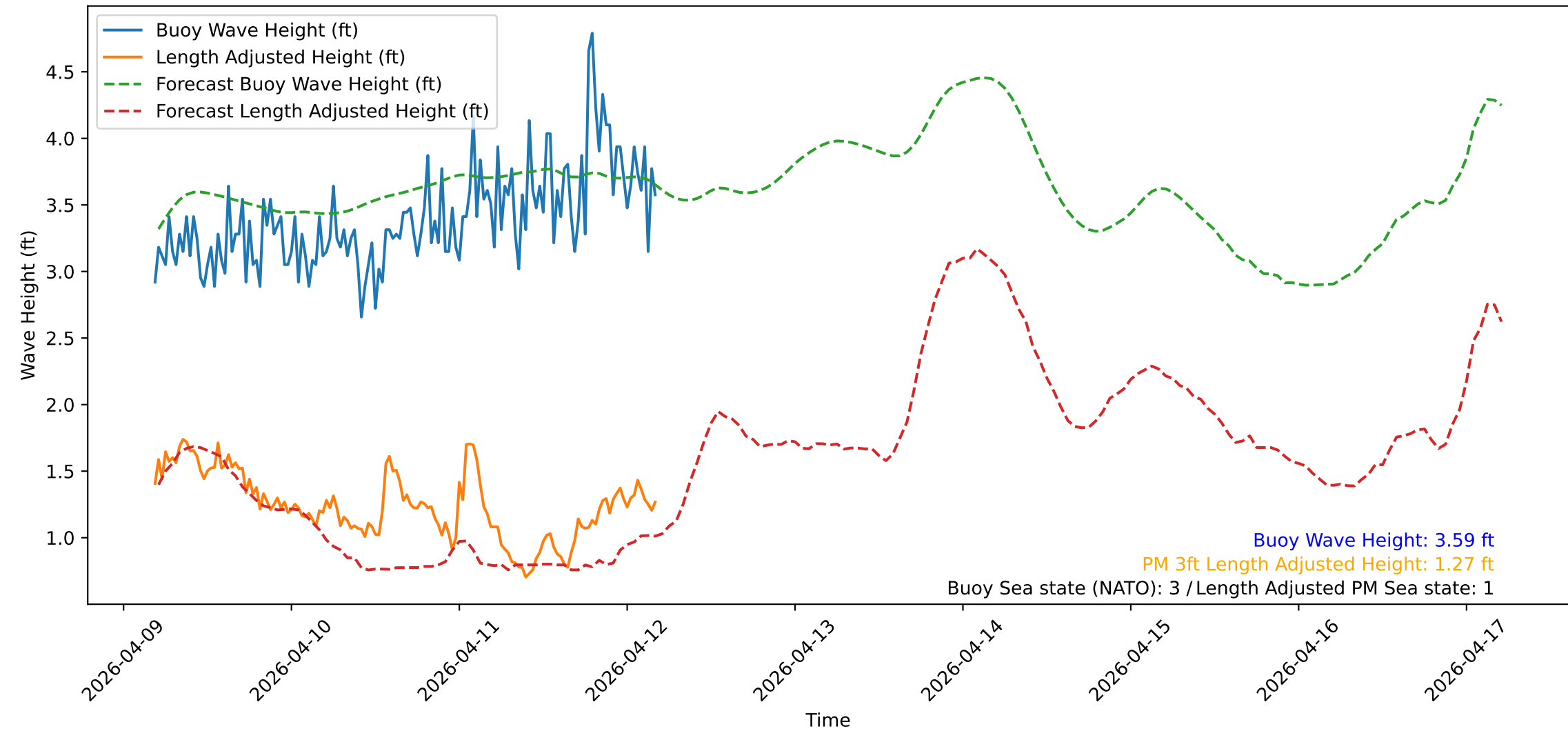
Wave Heights over Time for Oceanside Harbor at 2026-04-12 04:30:31
