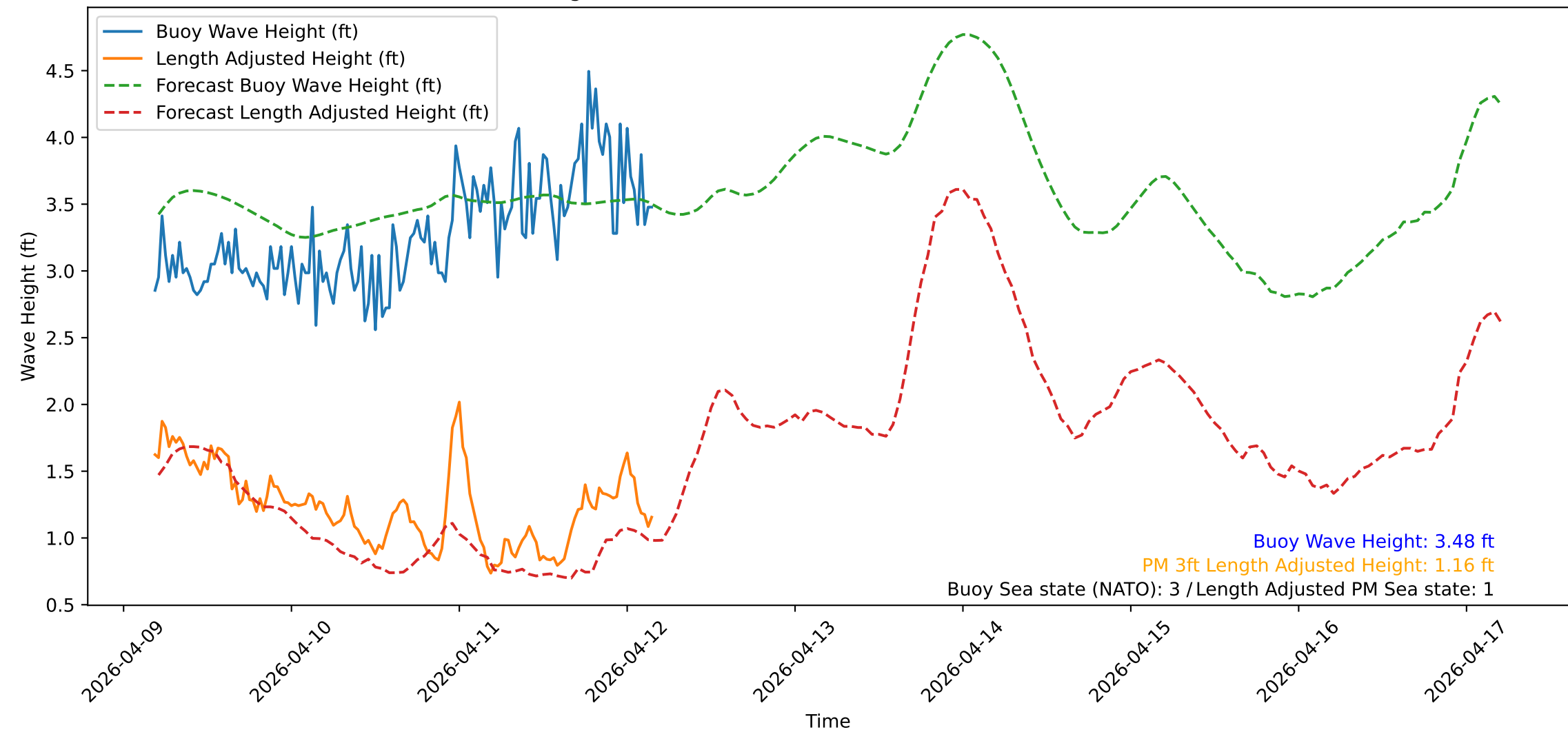
Wave Heights over Time for Green Beach at 2026-04-12 04:31:13
