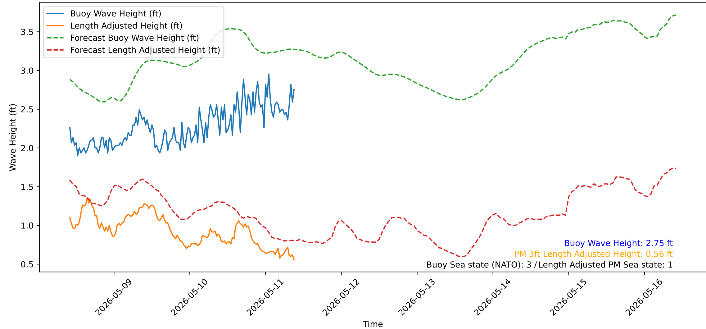
Wave Heights over Time for Red Beach at 2026-05-11 09:40:51
