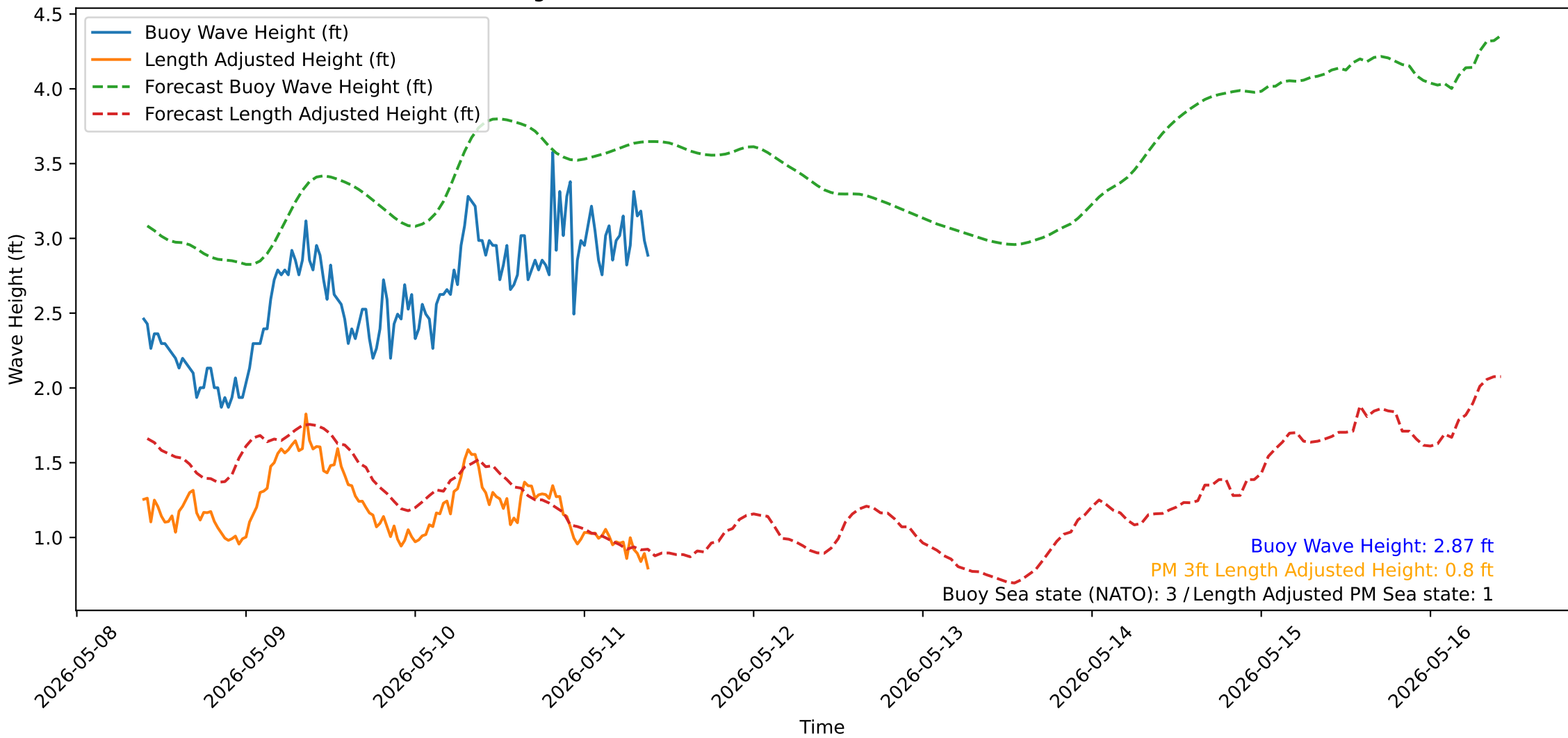
Wave Heights over Time for Oceanside Harbor at 2026-05-11 09:40:32
