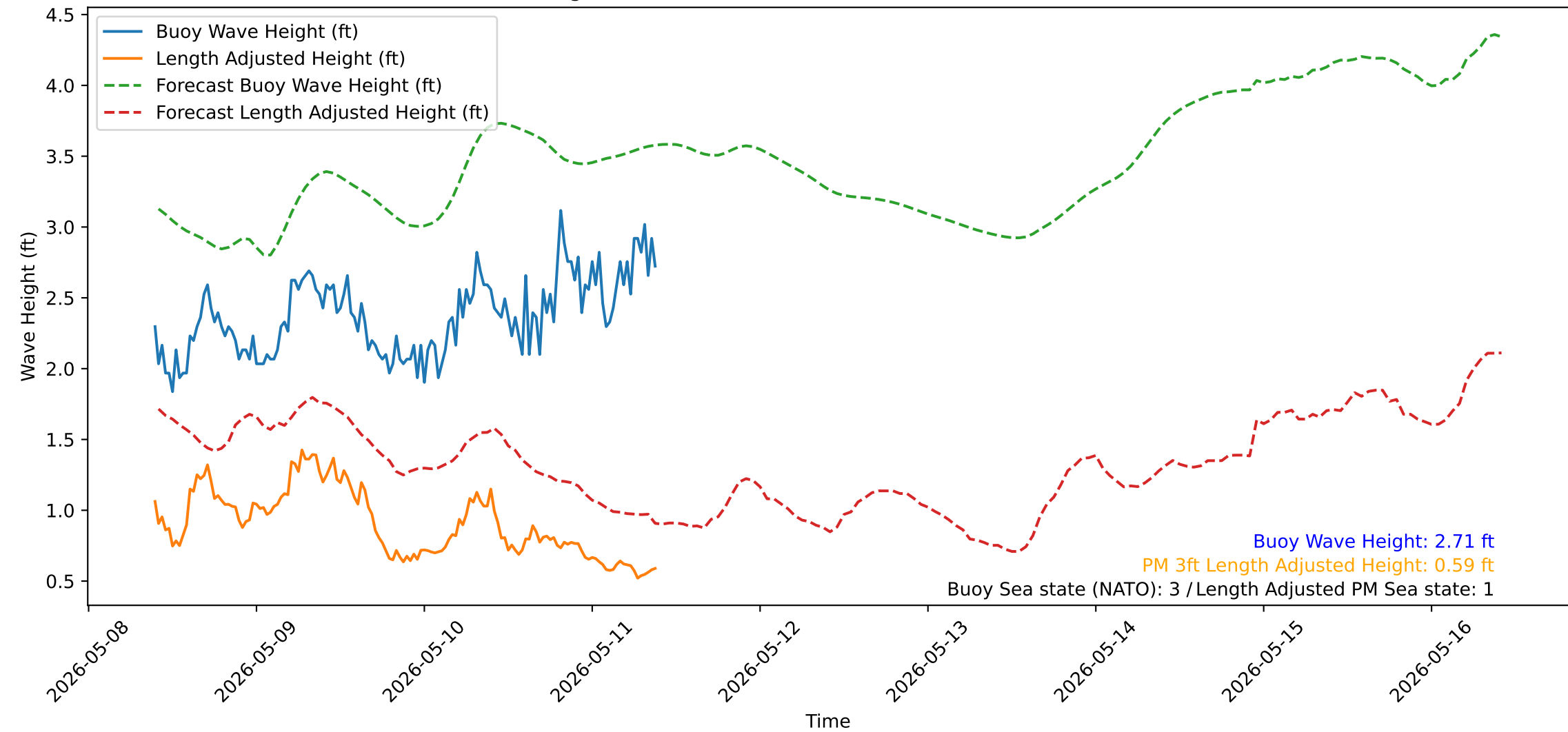
Wave Heights over Time for Green Beach at 2026-05-11 09:41:14
