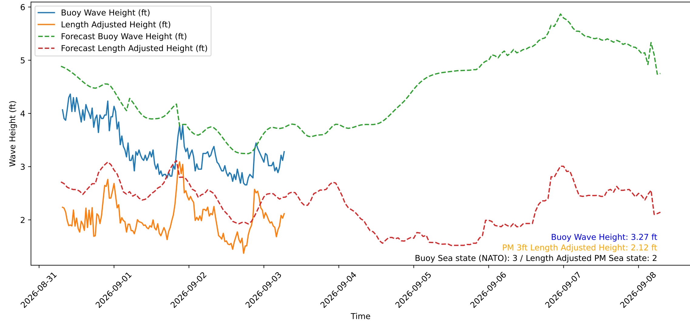
Wave Heights over Time for Green Beach at 2026-09-03 07:11:12
