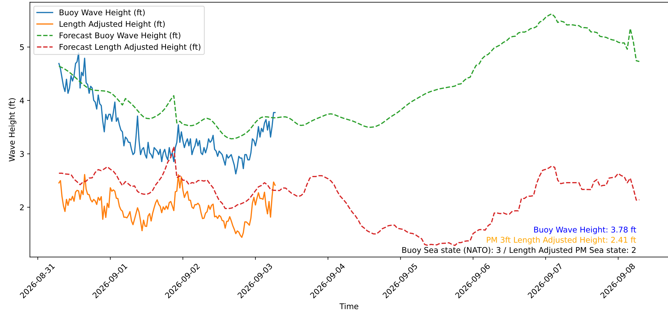
Wave Heights over Time for Oceanside Harbor at 2026-09-03 07:10:30
