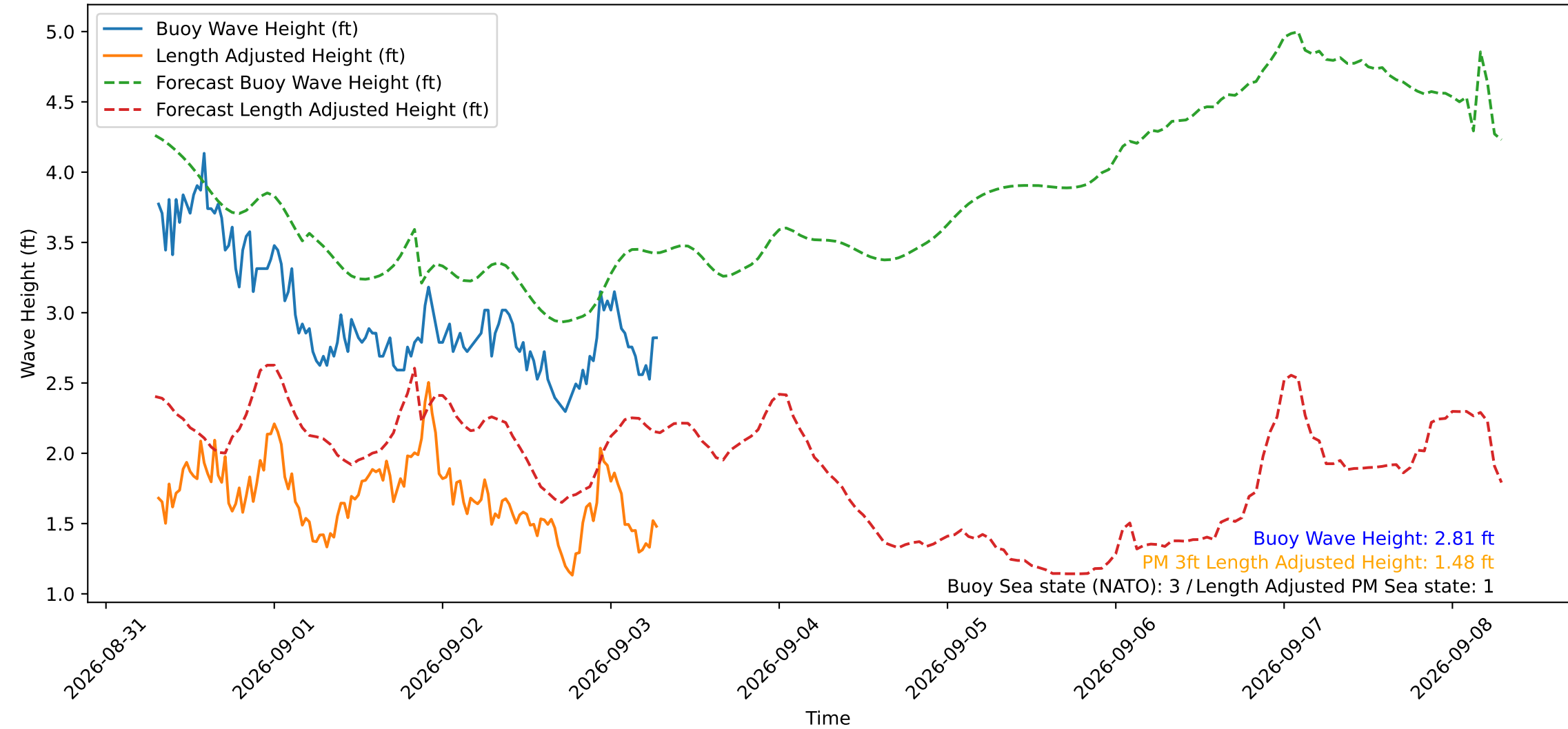
Wave Heights over Time for Red Beach at 2026-09-03 07:10:49
