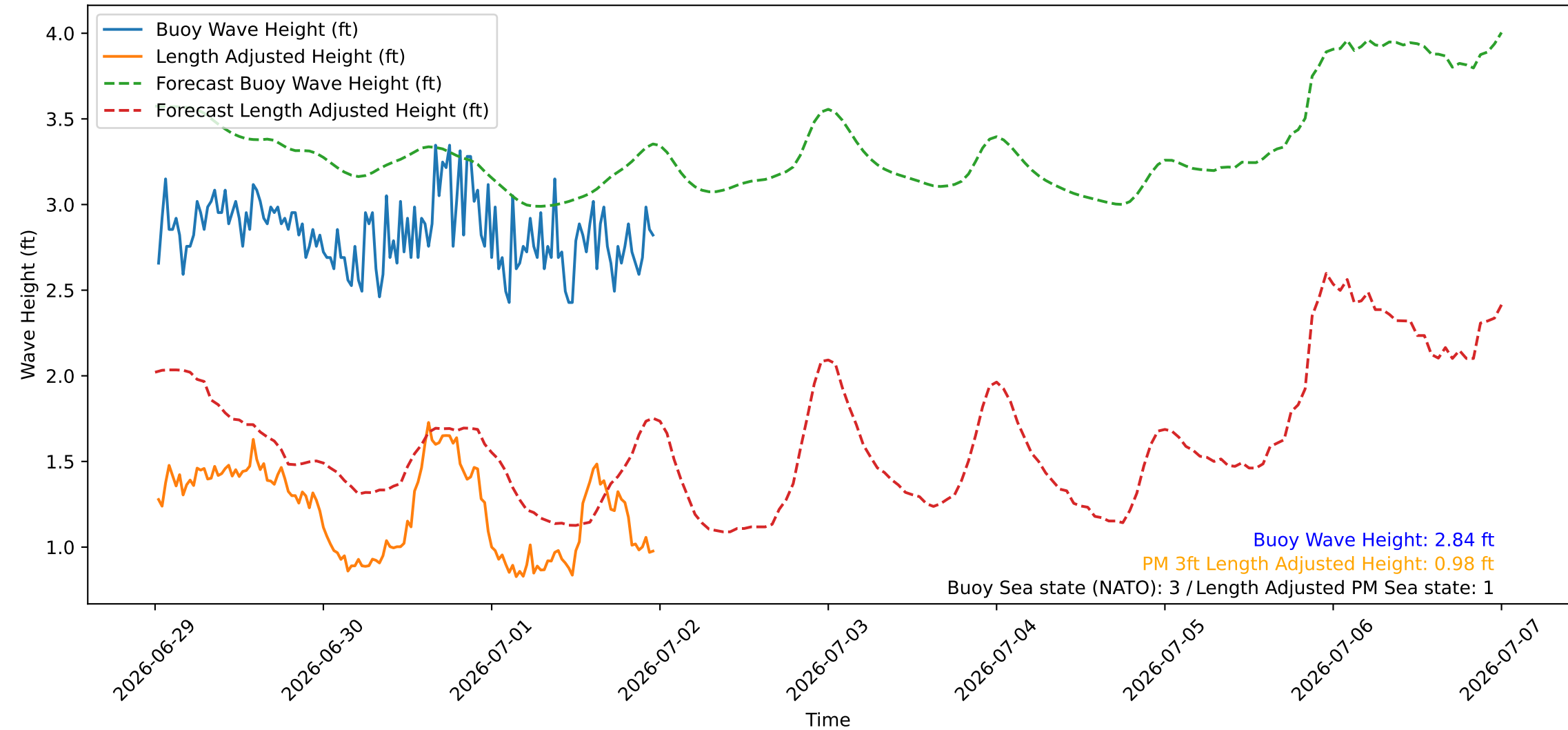
Wave Heights over Time for Red Beach at 2026-07-02 00:00:46
