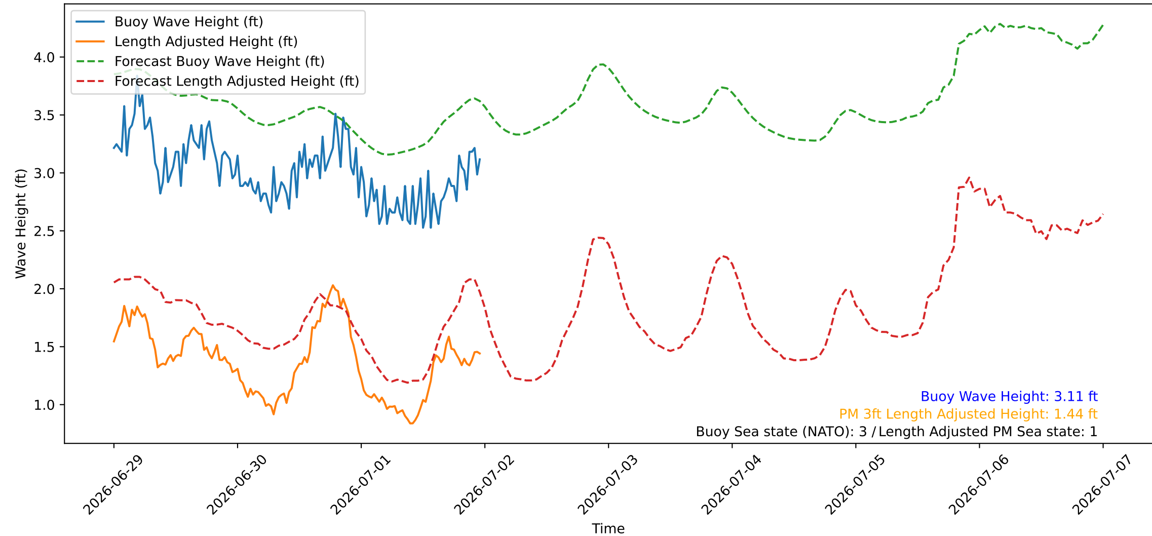
Wave Heights over Time for Green Beach at 2026-07-02 00:01:08
