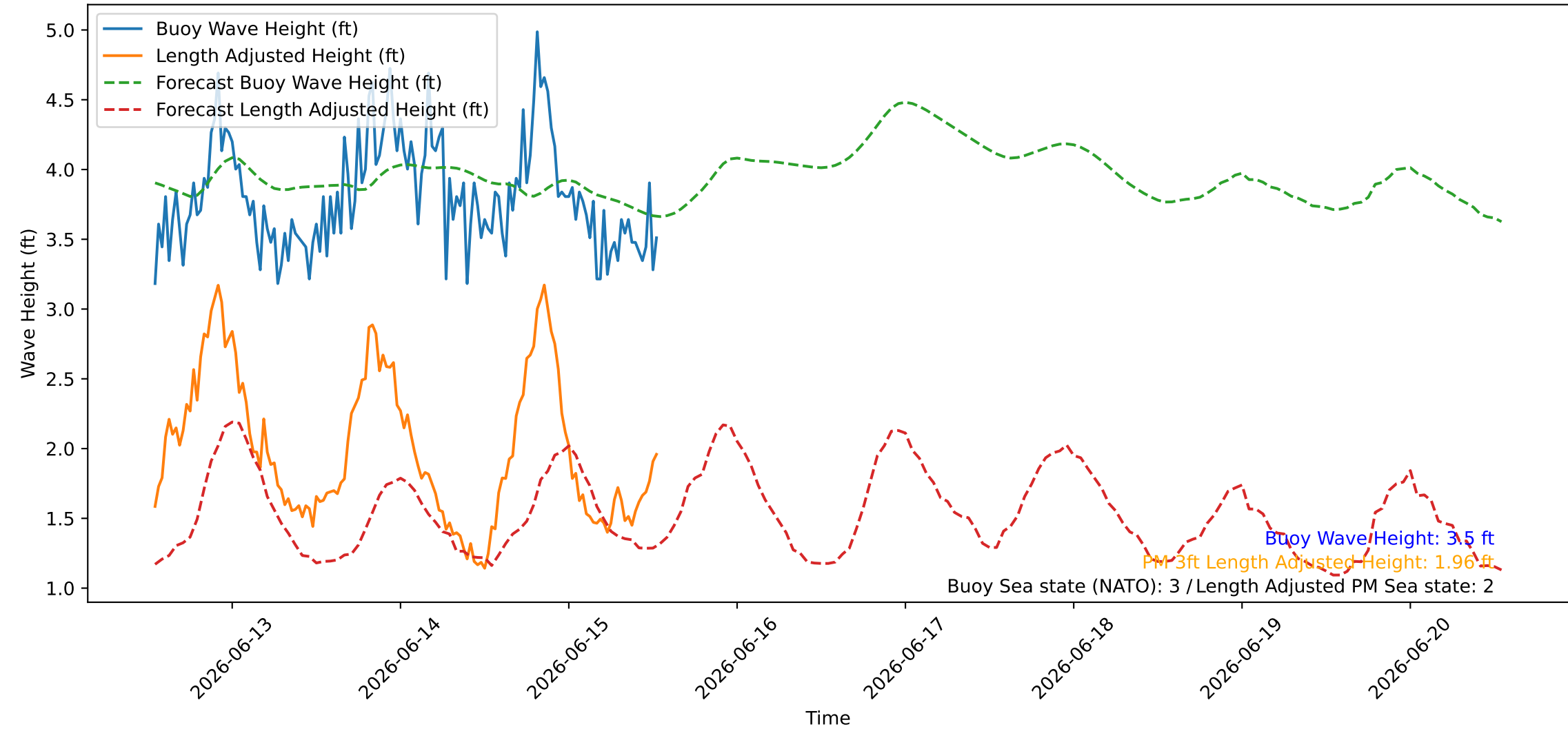
Wave Heights over Time for Oceanside Harbor at 2026-06-15 13:00:25
