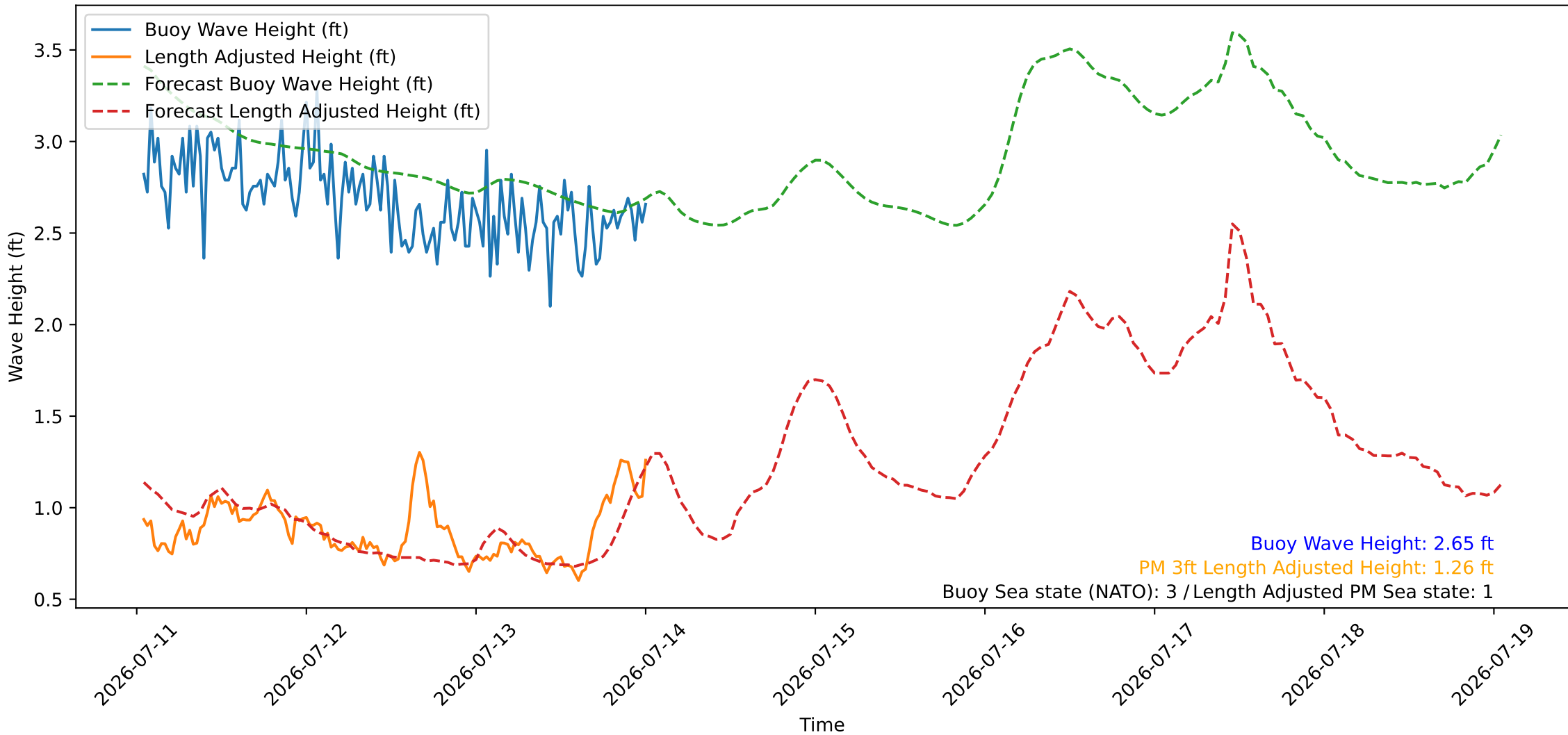
Wave Heights over Time for Oceanside Harbor at 2026-07-14 01:00:27
