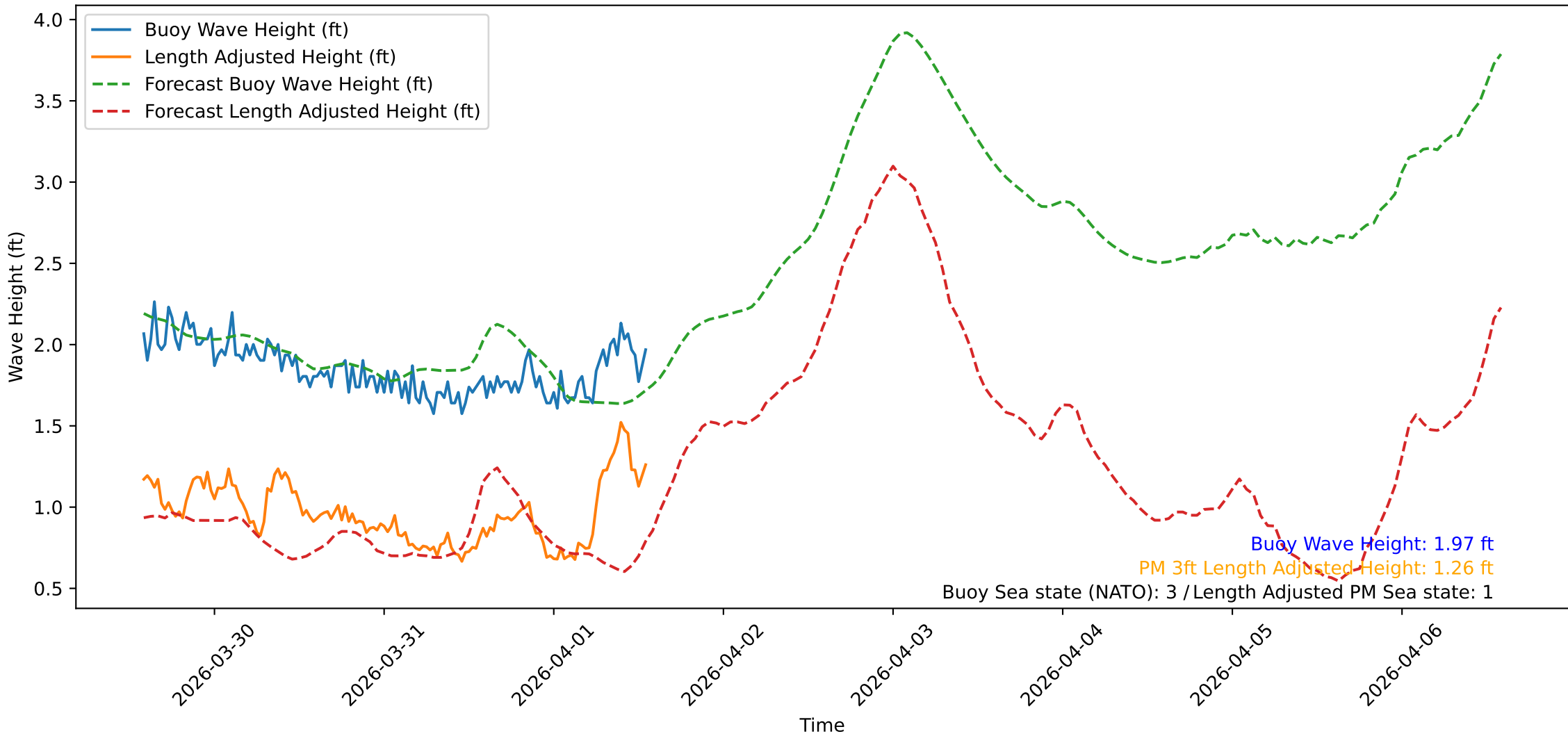
Wave Heights over Time for Oceanside Harbor at 2026-04-01 14:10:31
