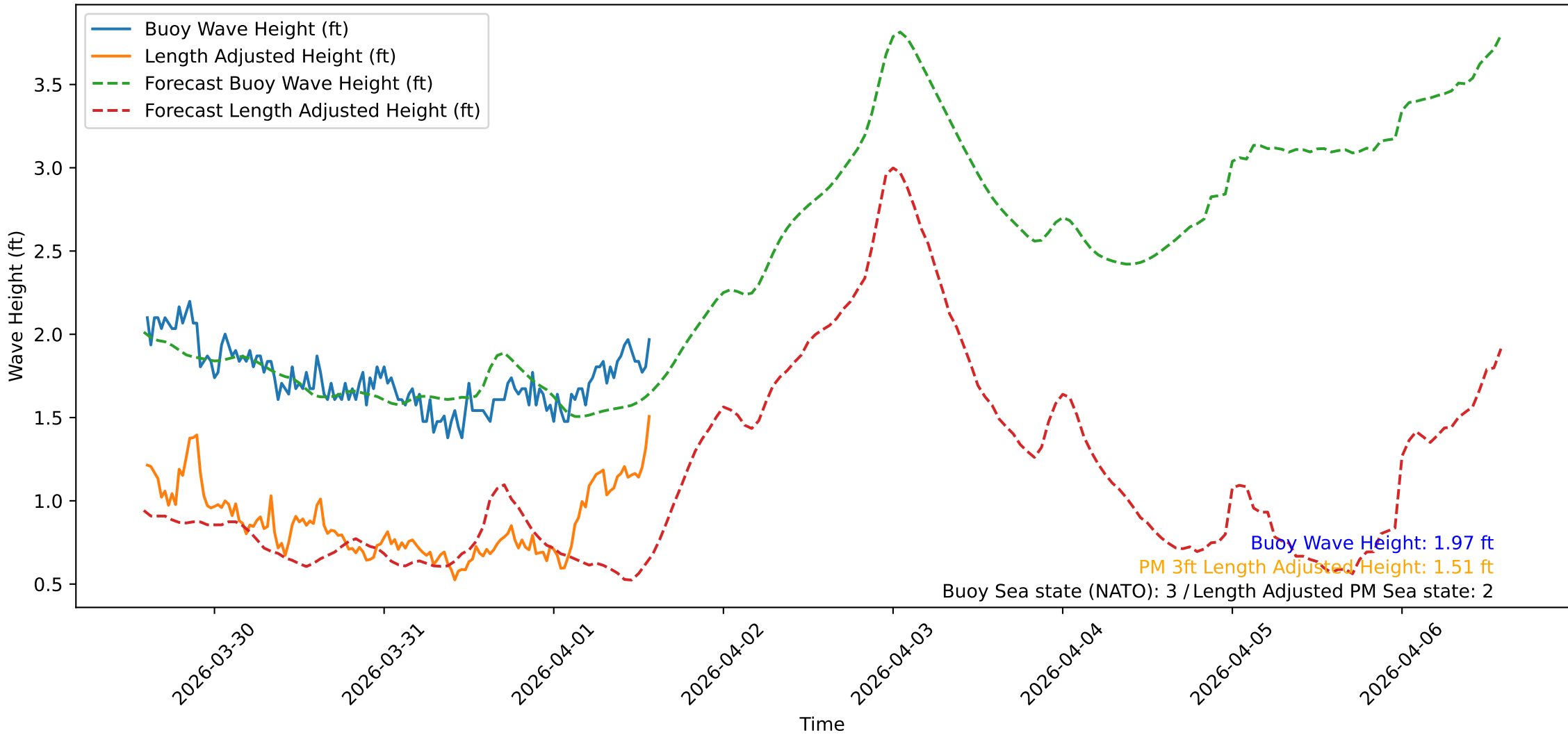
Wave Heights over Time for Red Beach at 2026-04-01 14:10:47
