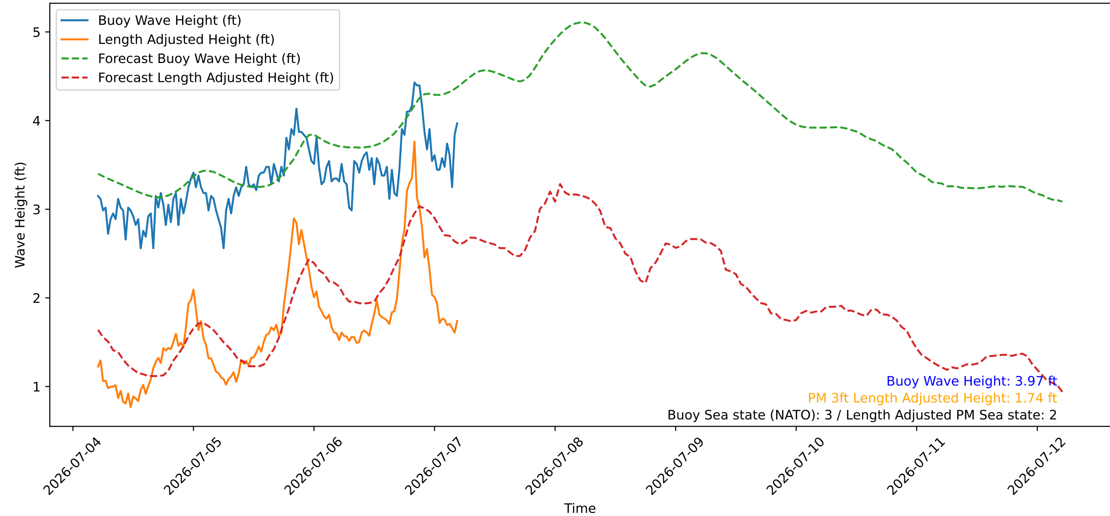
Wave Heights over Time for Green Beach at 2026-07-07 05:11:08
