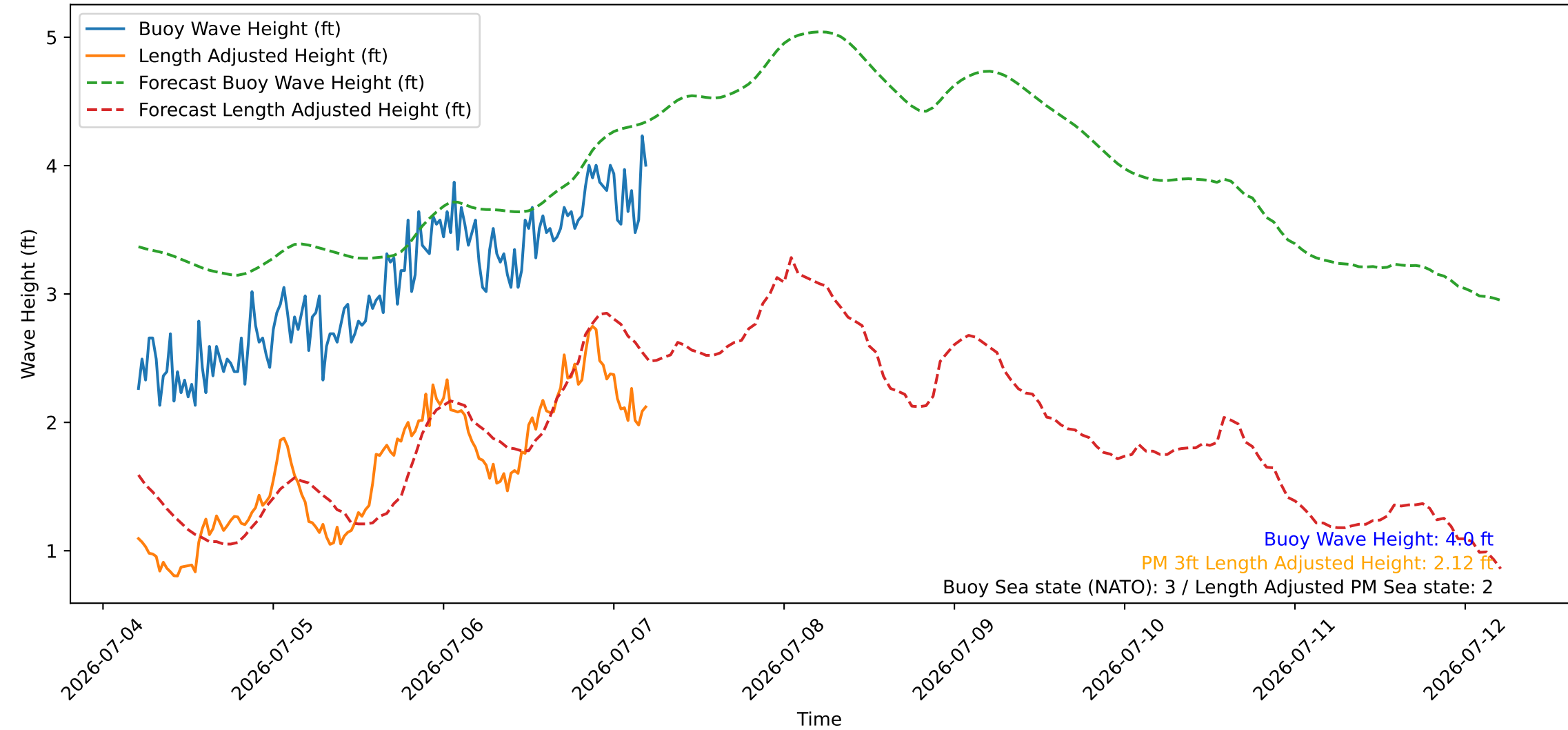
Wave Heights over Time for Oceanside Harbor at 2026-07-07 05:10:26
