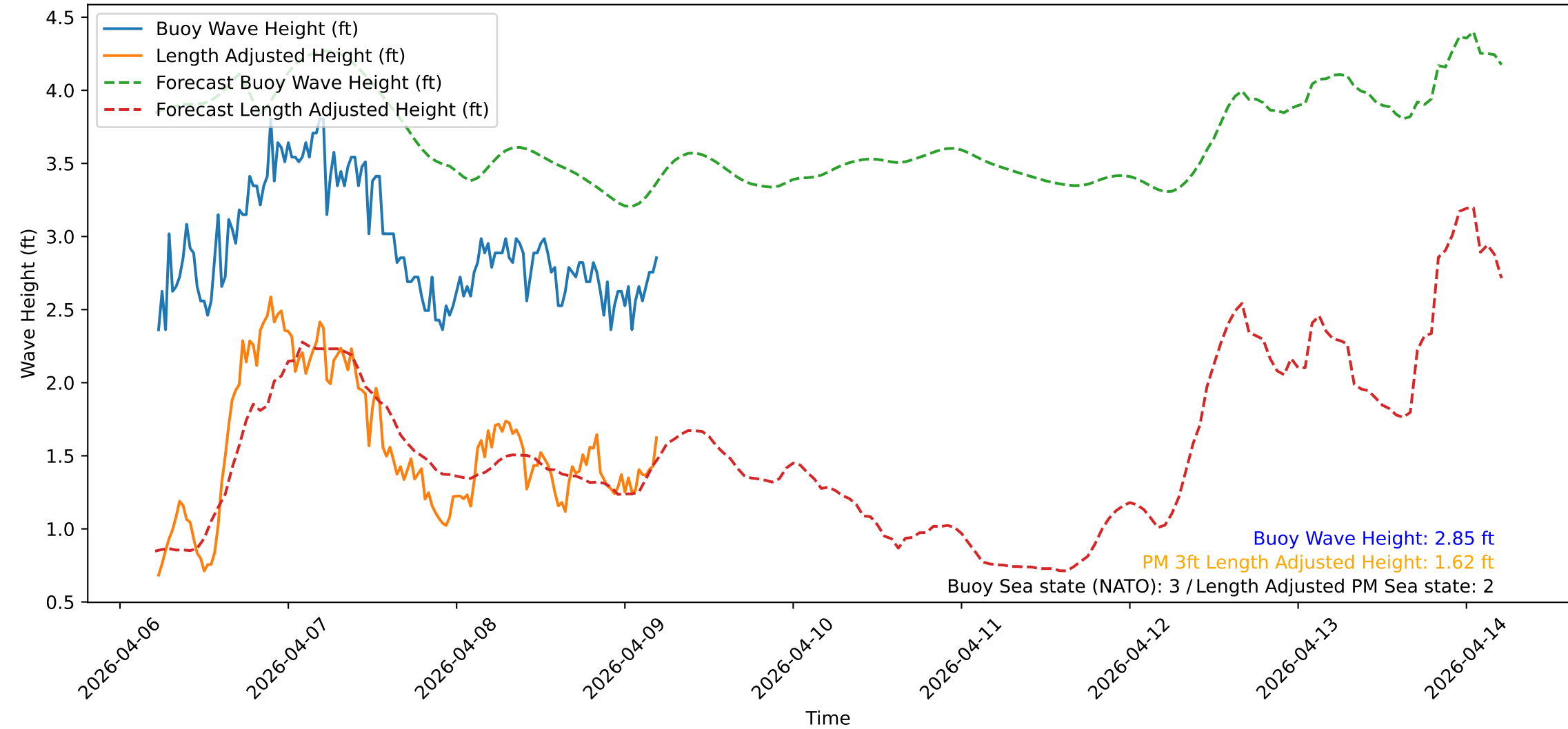
Wave Heights over Time for Green Beach at 2026-04-09 05:21:09
