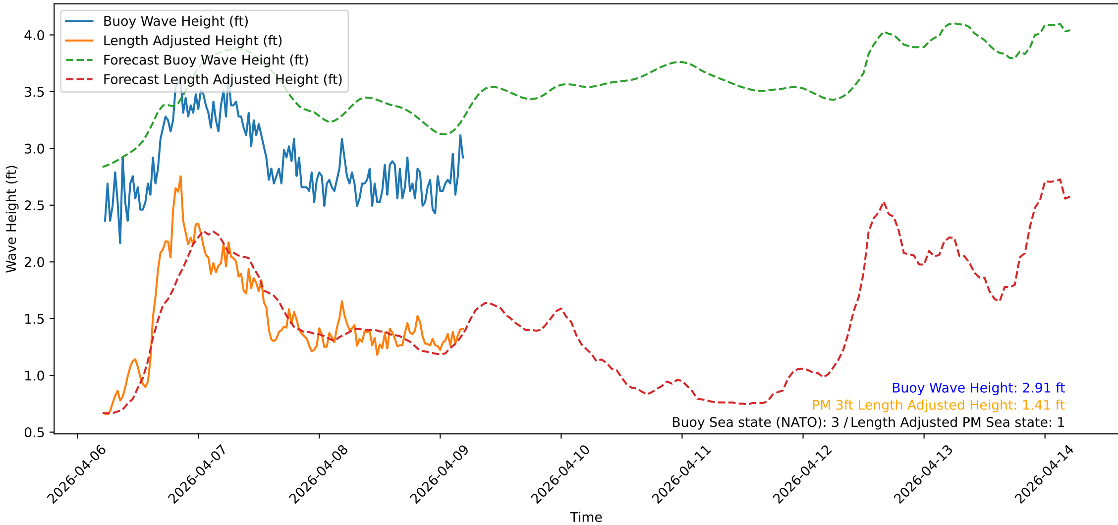
Wave Heights over Time for Oceanside Harbor at 2026-04-09 05:20:31
