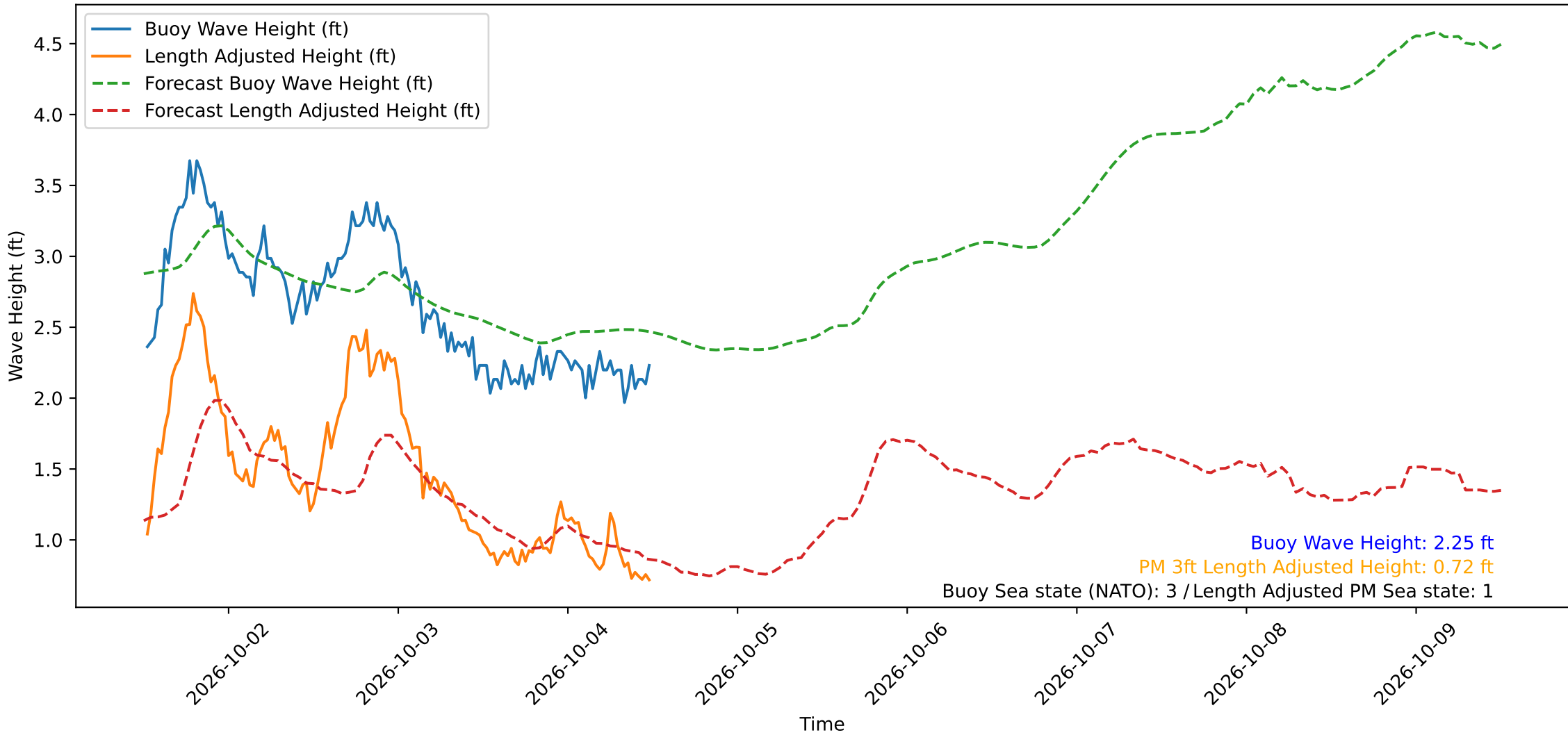
Wave Heights over Time for Green Beach at 2026-10-04 12:21:14
