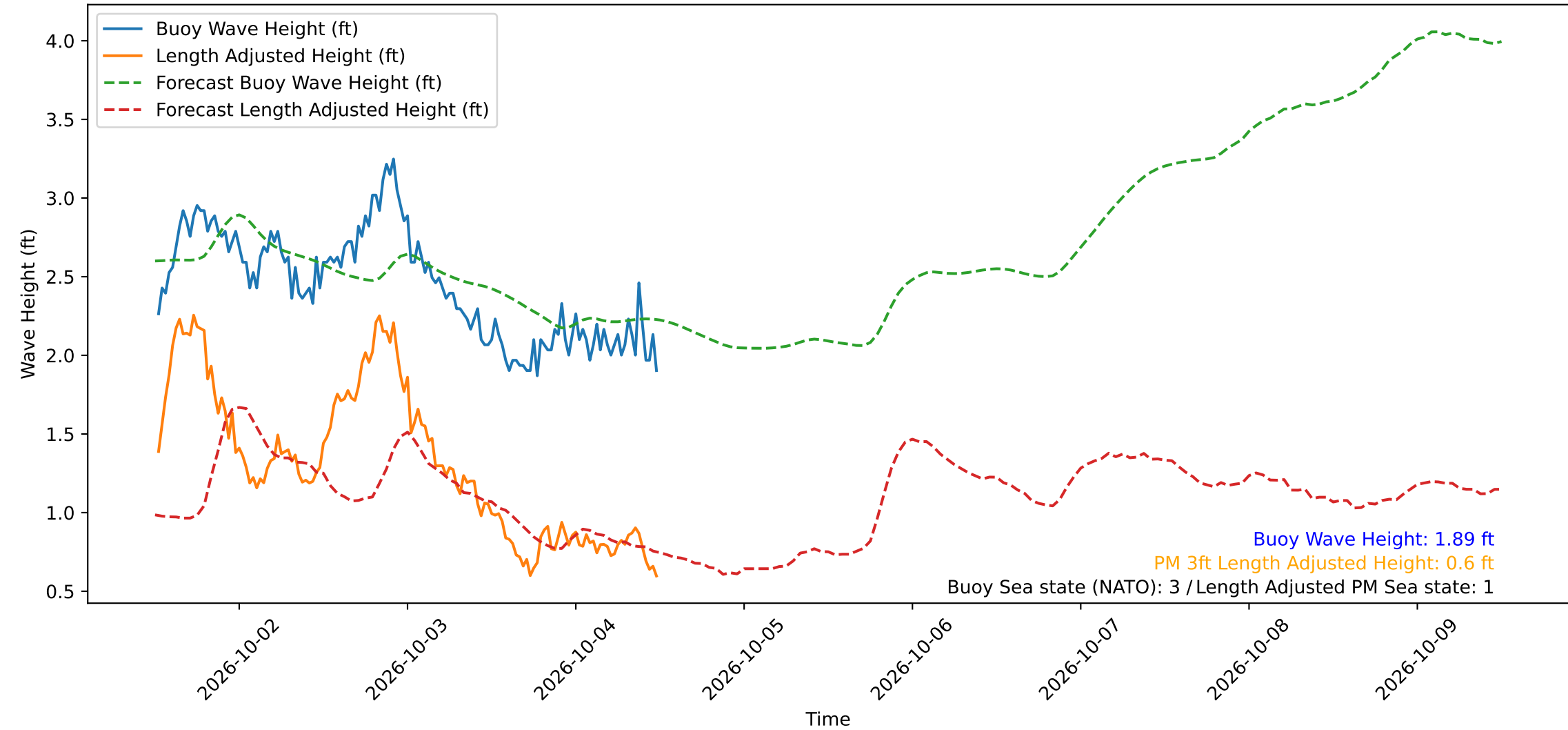
Wave Heights over Time for Red Beach at 2026-10-04 12:20:51
