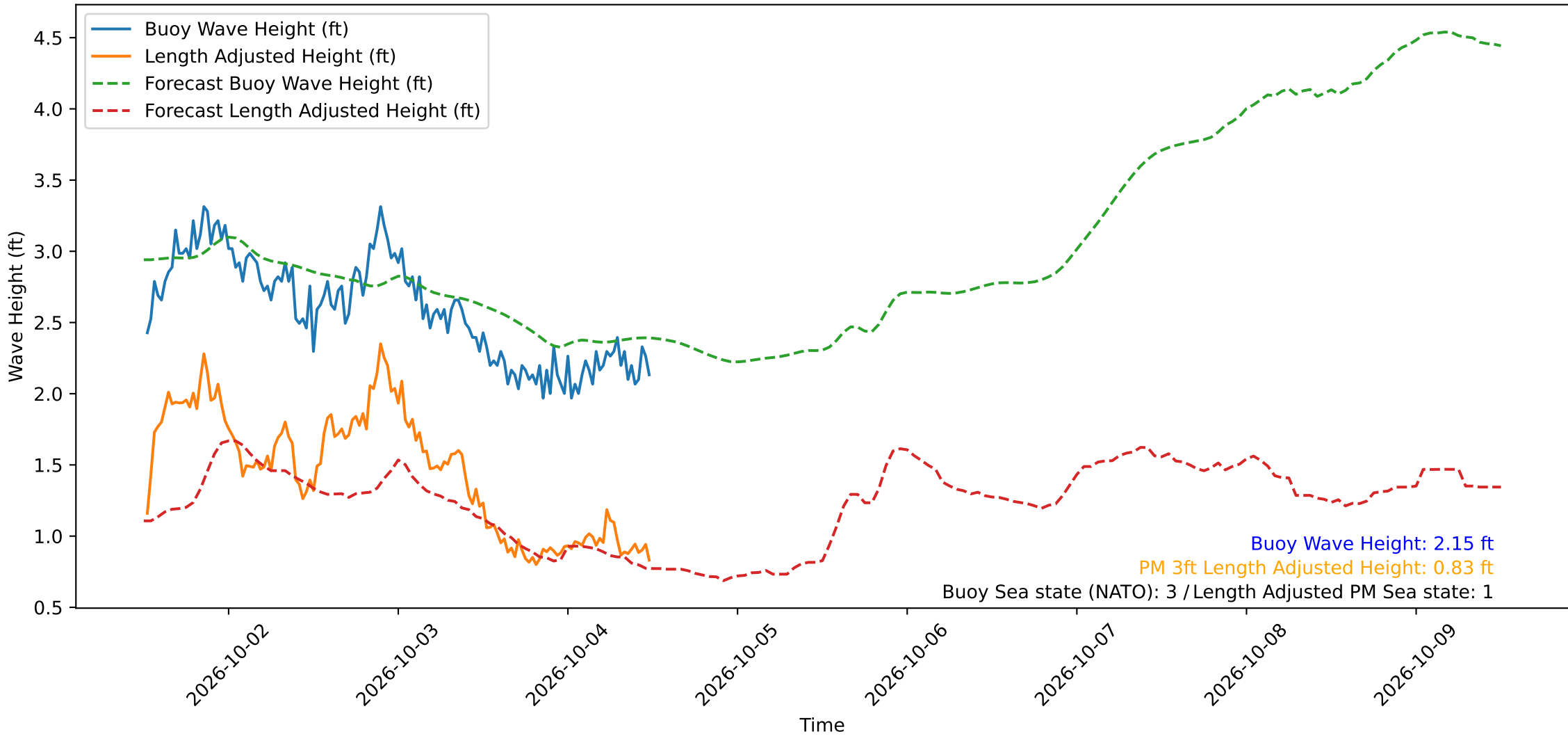
Wave Heights over Time for Oceanside Harbor at 2026-10-04 12:20:30
