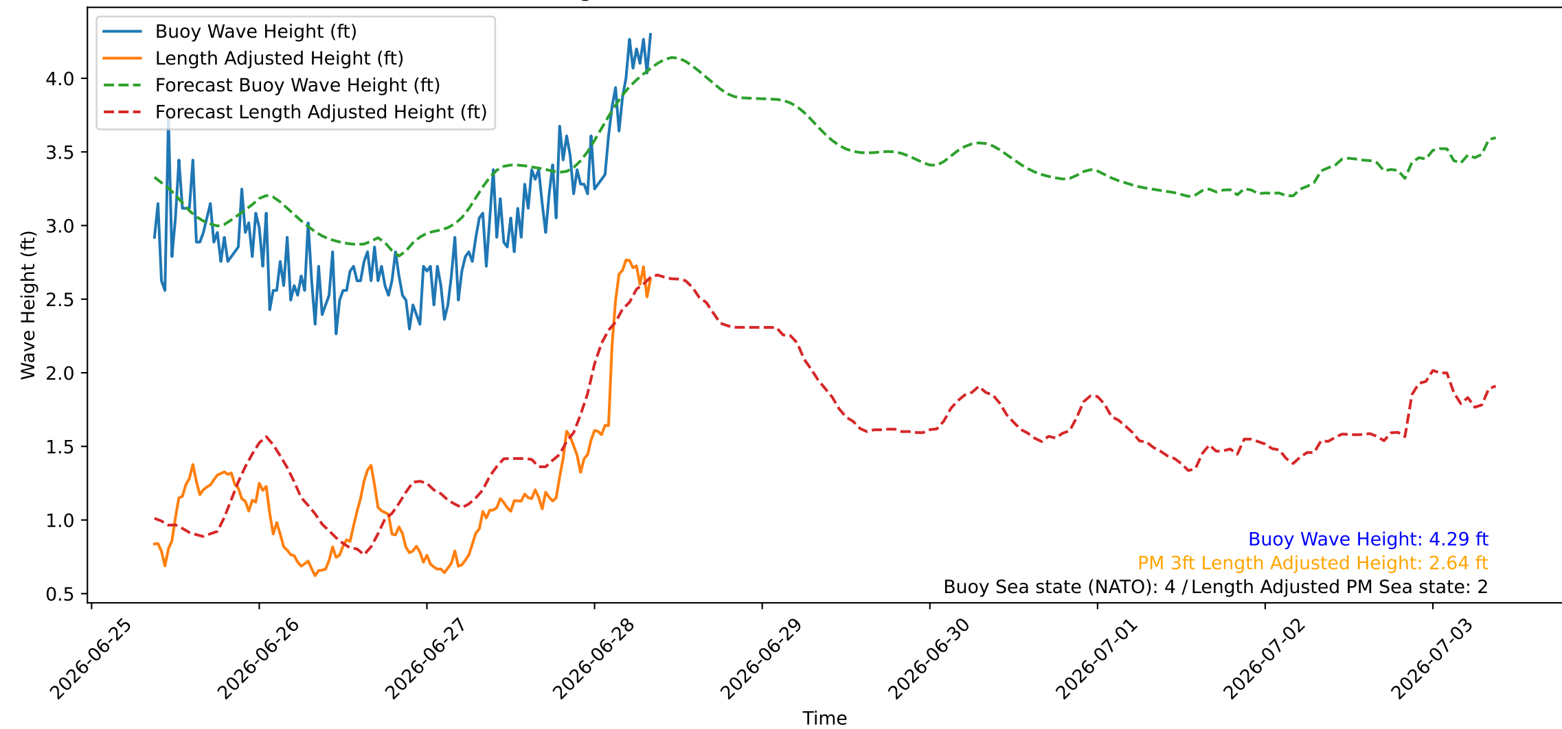
Wave Heights over Time for Red Beach at 2026-06-28 08:40:45
