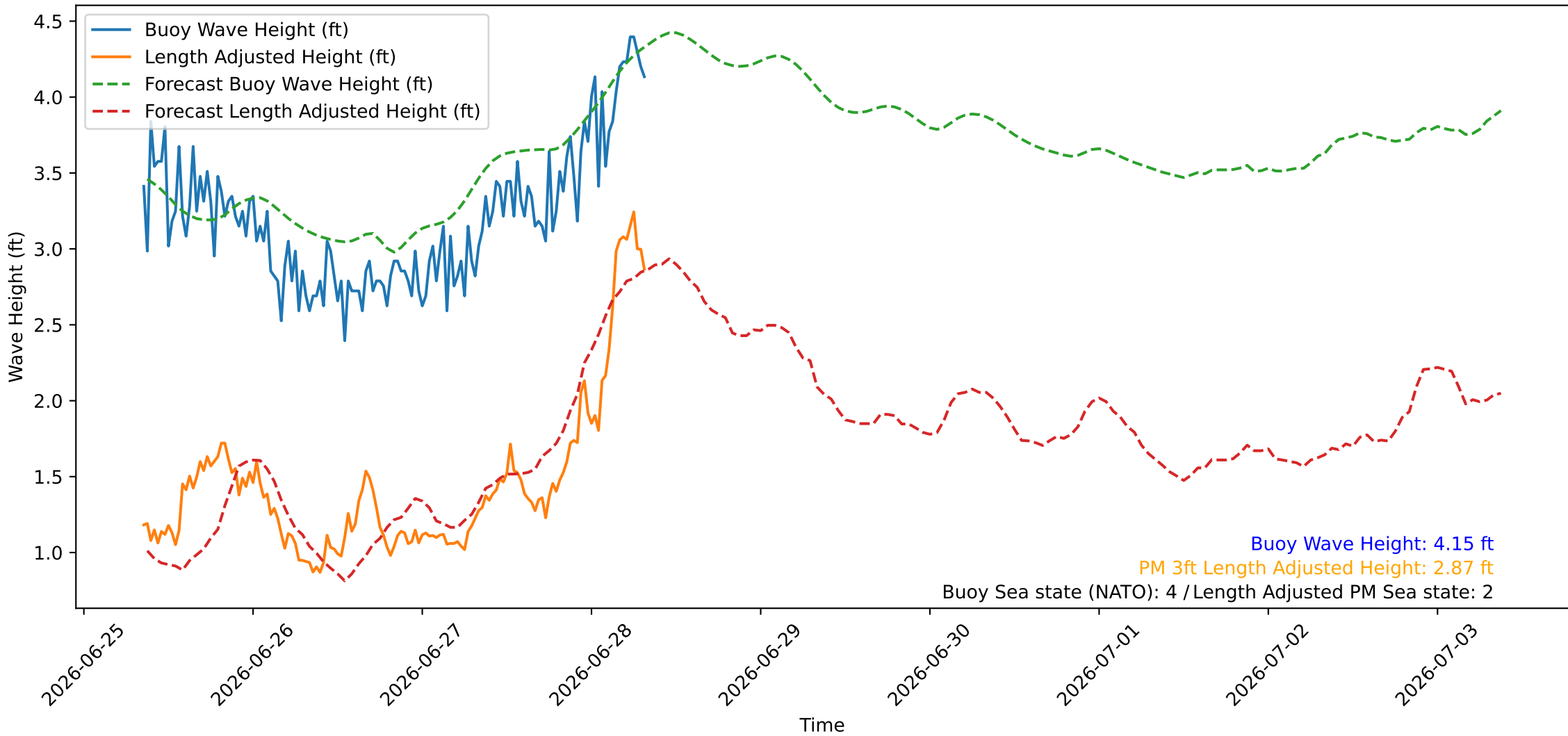
Wave Heights over Time for Oceanside Harbor at 2026-06-28 08:40:26
