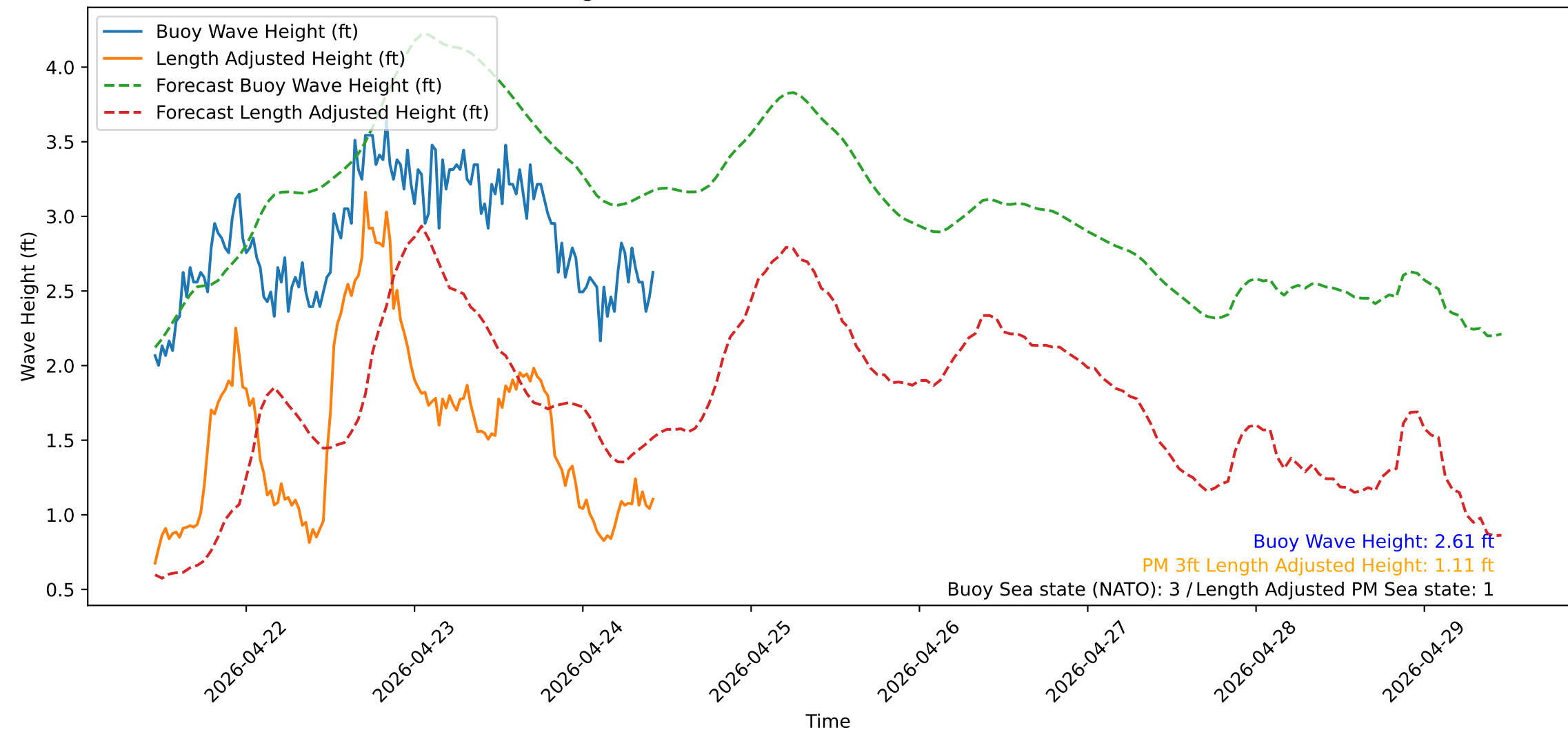
Wave Heights over Time for Red Beach at 2026-04-24 10:50:52
