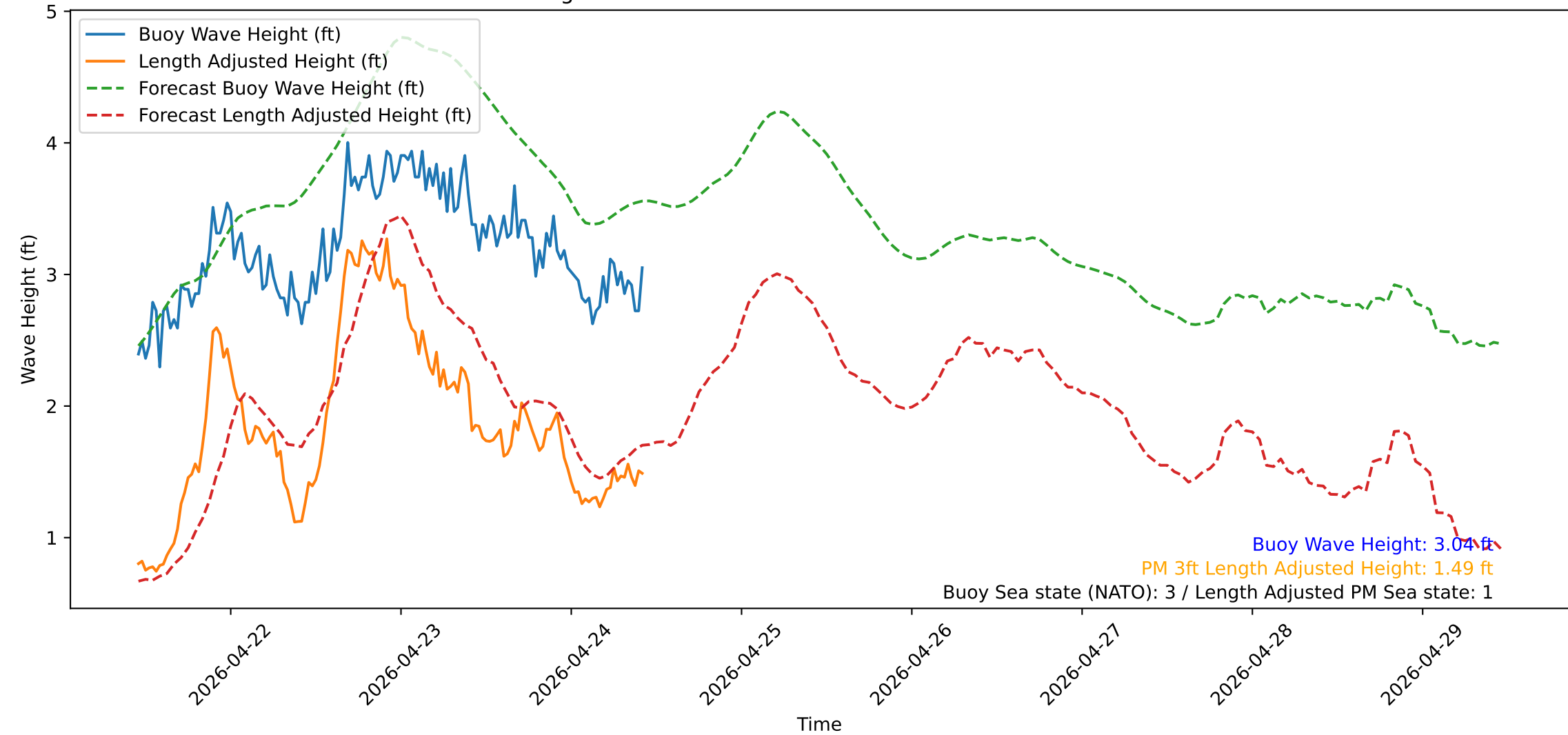
Wave Heights over Time for Green Beach at 2026-04-24 10:51:14
