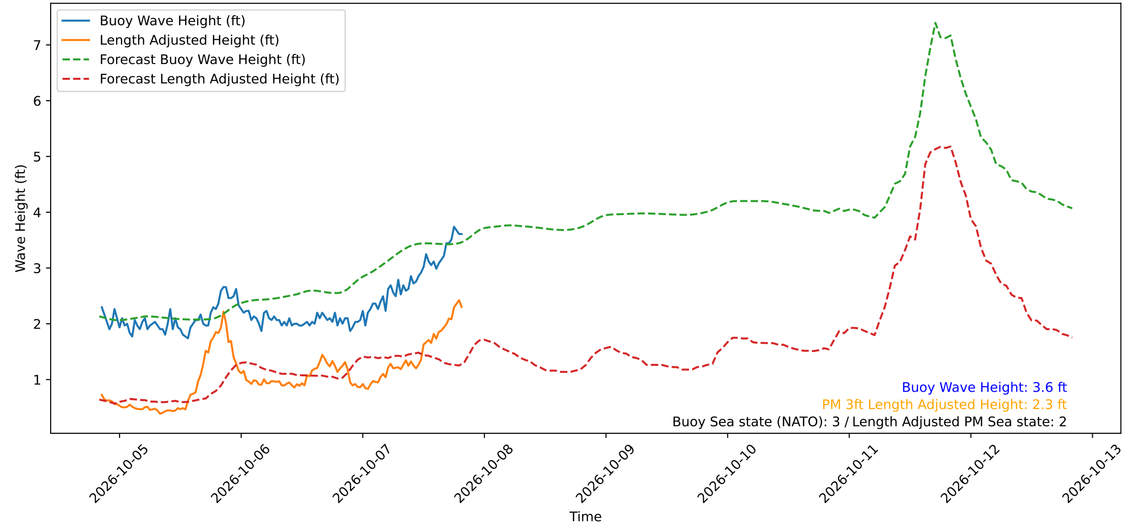
Wave Heights over Time for Red Beach at 2026-10-07 20:10:49
