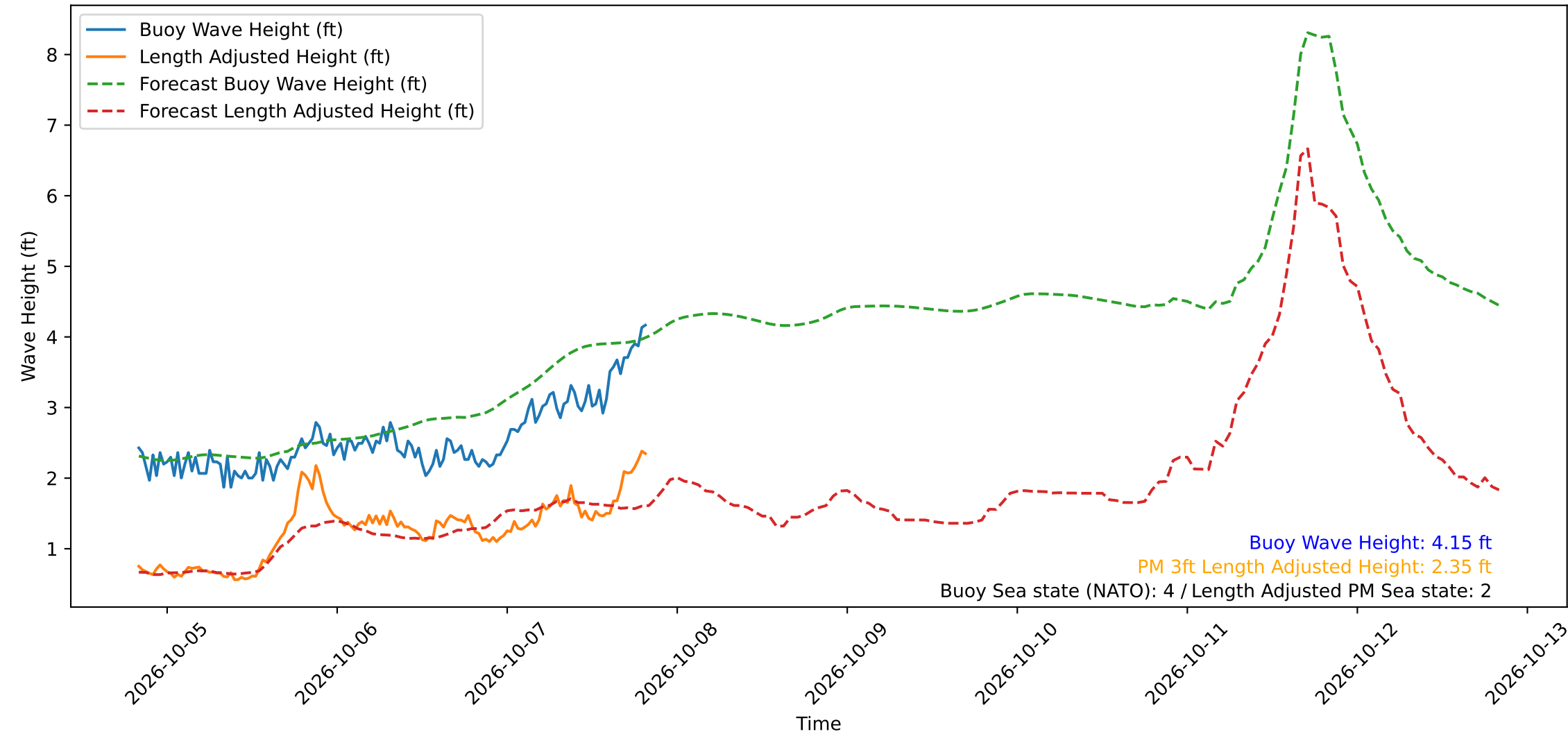
Wave Heights over Time for Oceanside Harbor at 2026-10-07 20:10:29
