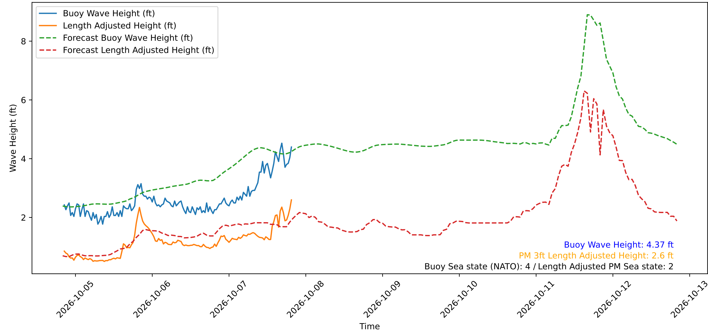
Wave Heights over Time for Green Beach at 2026-10-07 20:11:12
