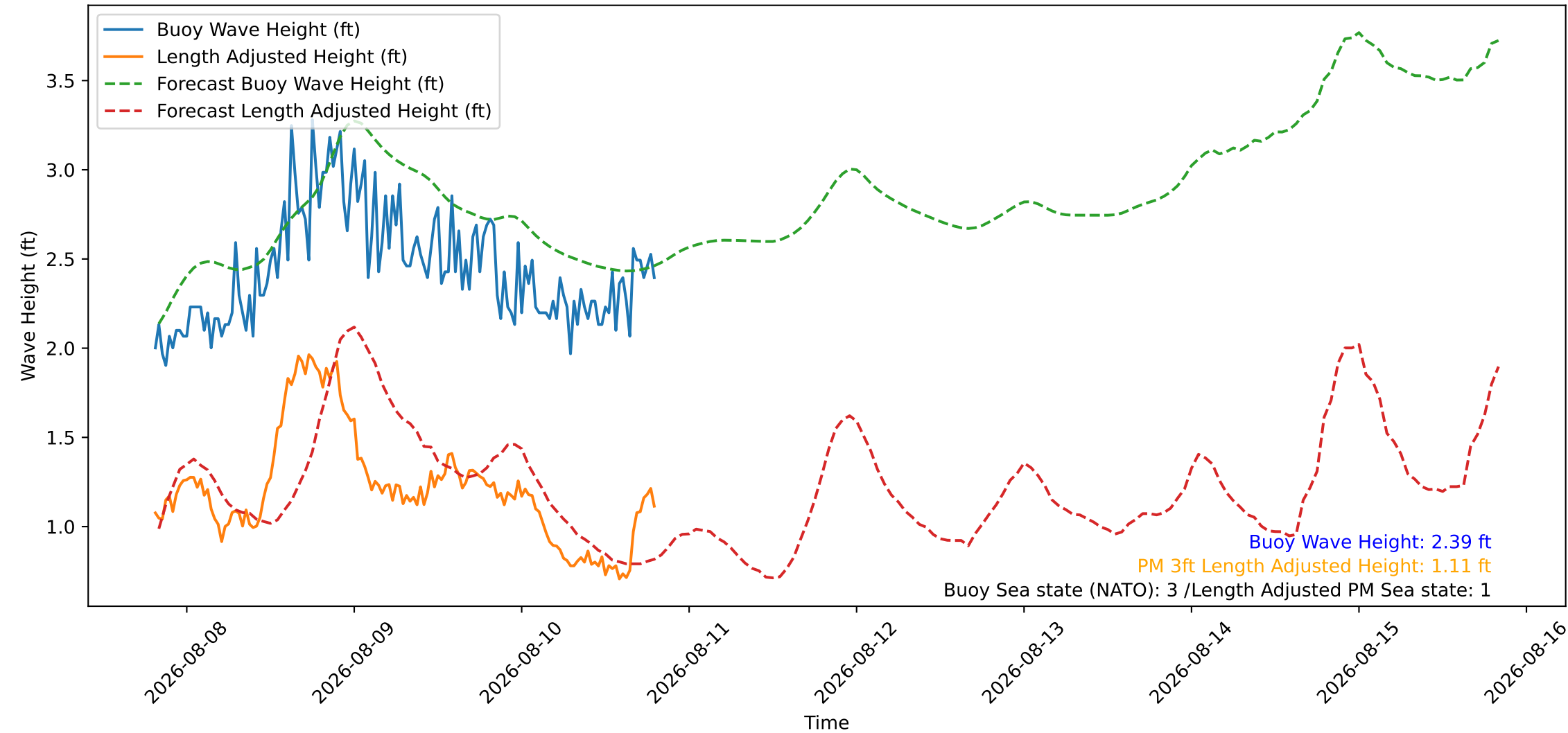
Wave Heights over Time for Oceanside Harbor at 2026-08-10 19:40:26
