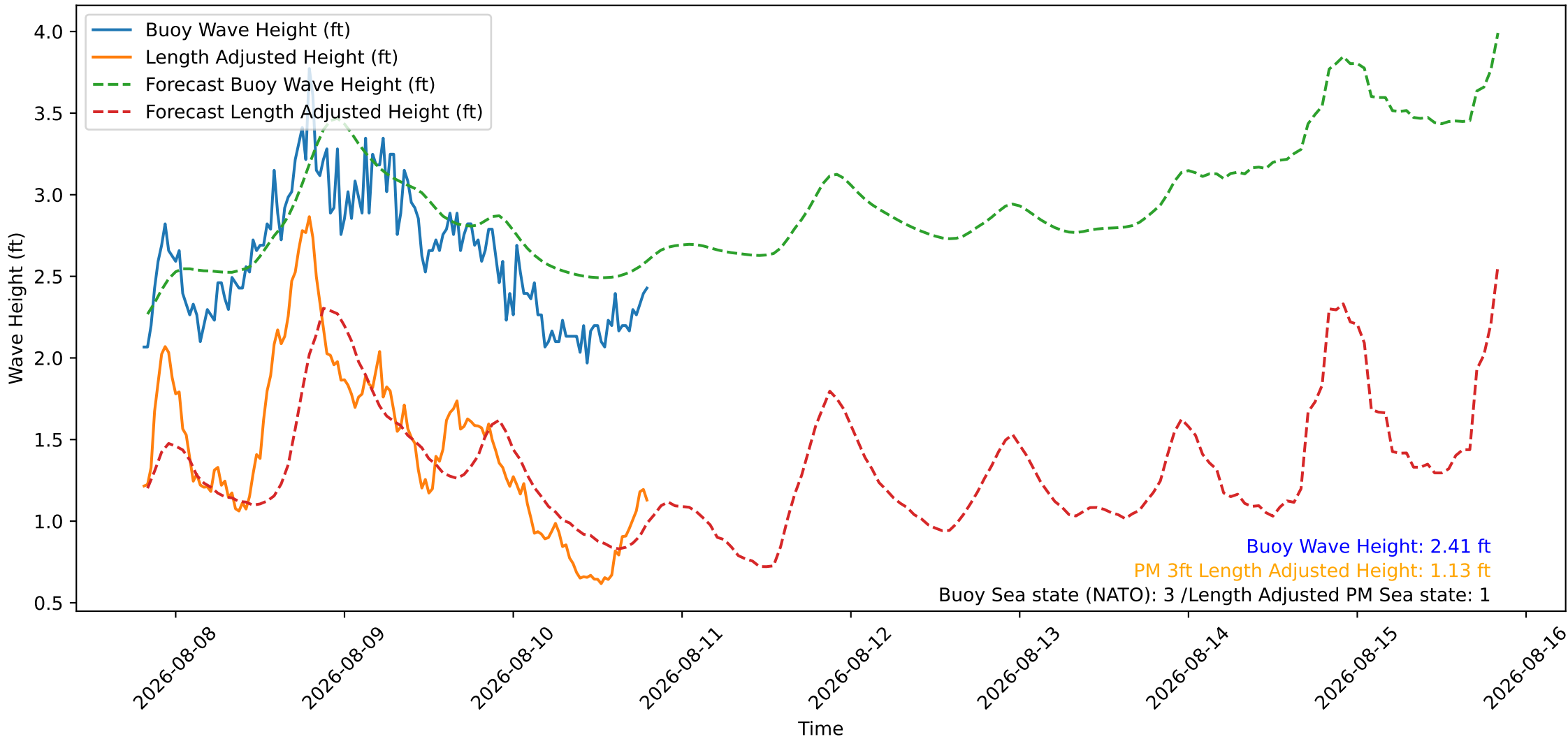
Wave Heights over Time for Green Beach at 2026-08-10 19:41:08
