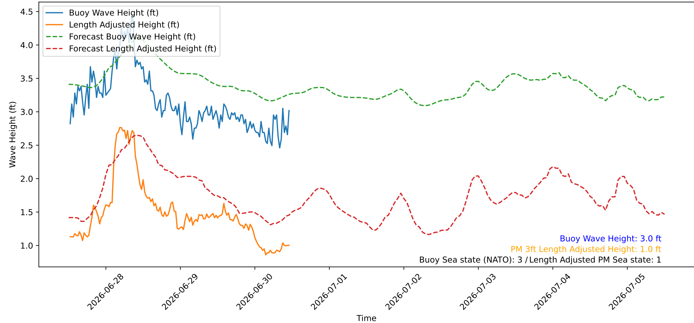
Wave Heights over Time for Red Beach at 2026-06-30 12:10:45
