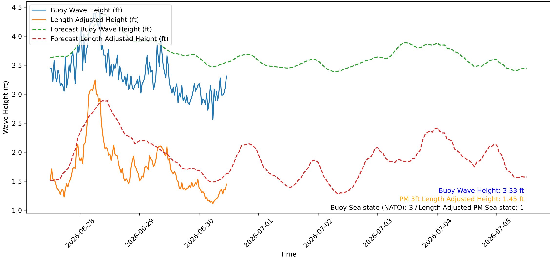
Wave Heights over Time for Oceanside Harbor at 2026-06-30 12:10:26
