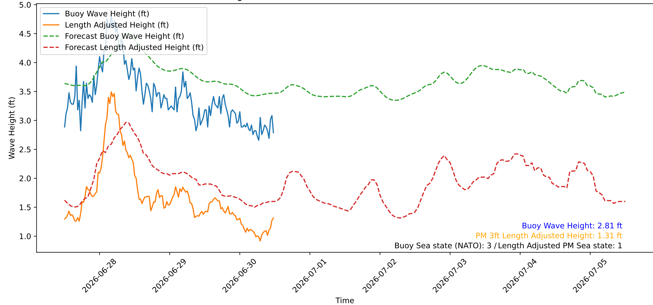
Wave Heights over Time for Green Beach at 2026-06-30 12:11:07
