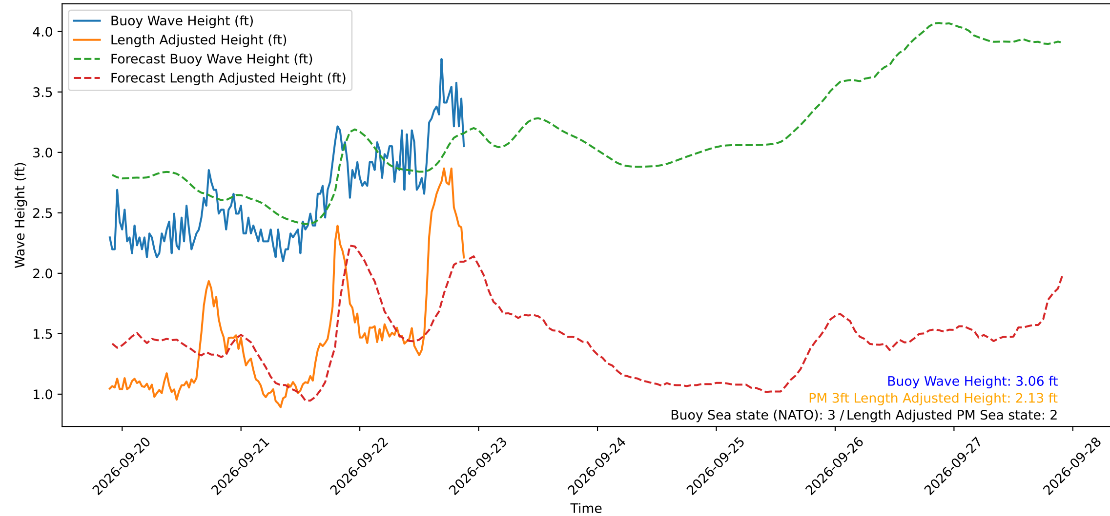
Wave Heights over Time for Oceanside Harbor at 2026-09-22 21:40:30
