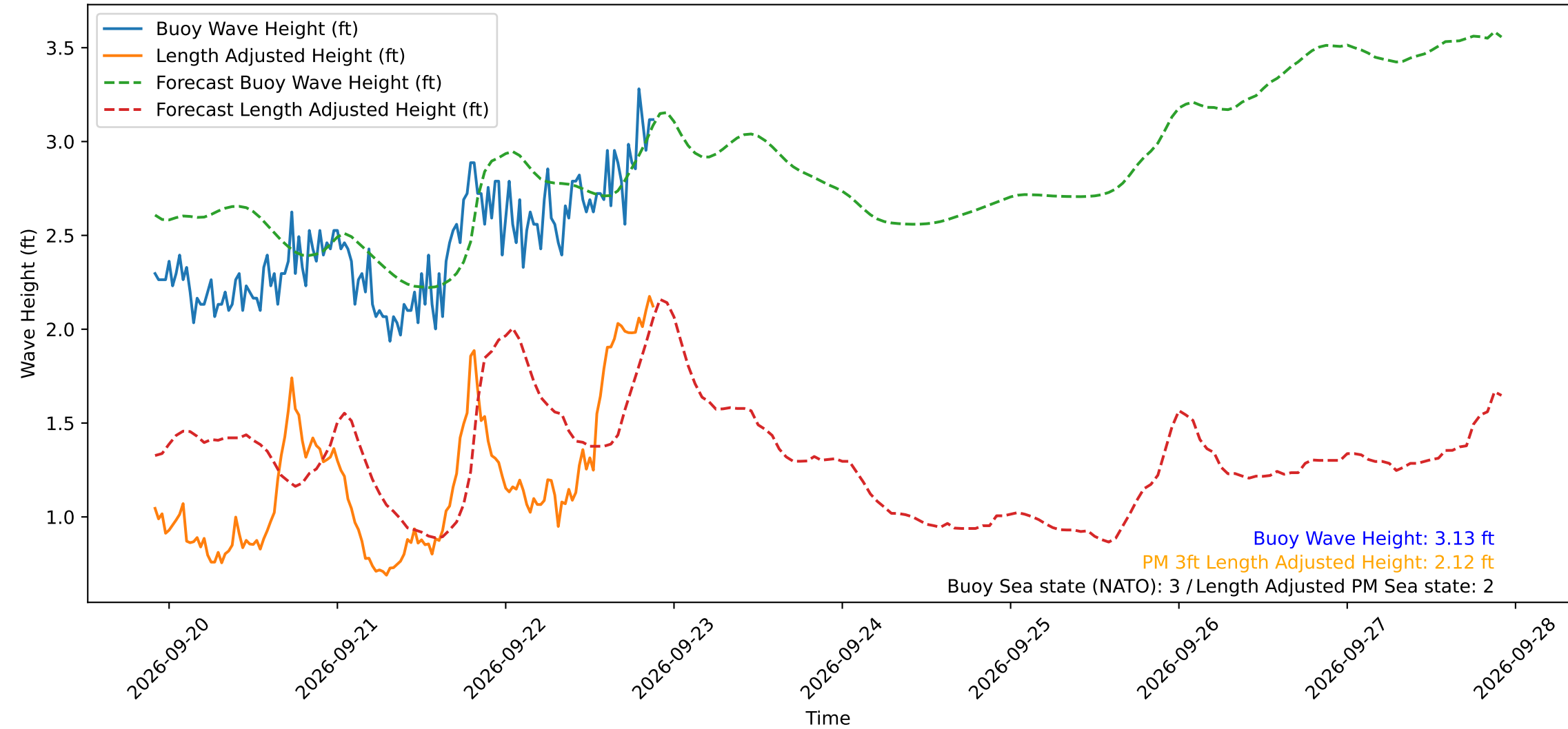
Wave Heights over Time for Red Beach at 2026-09-22 21:40:49
