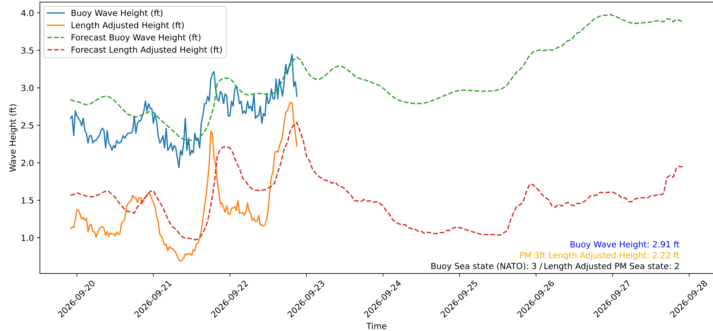
Wave Heights over Time for Green Beach at 2026-09-22 21:41:12
