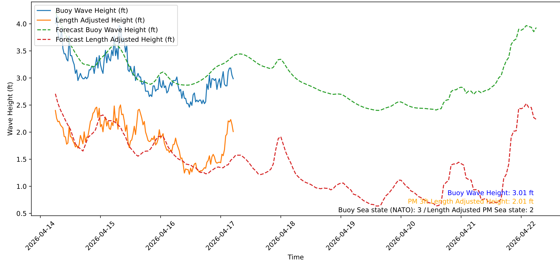
Wave Heights over Time for Green Beach at 2026-04-17 05:51:14
