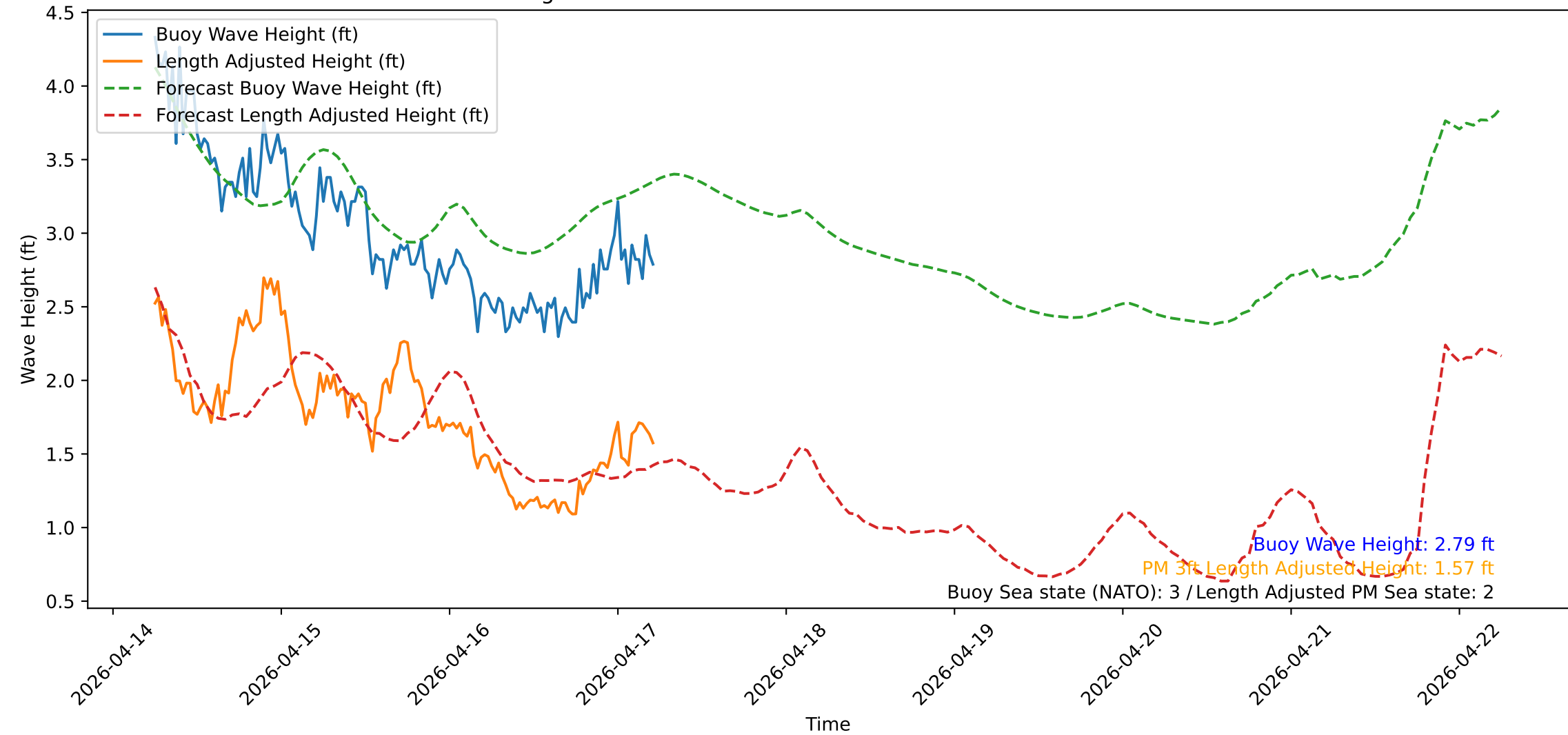
Wave Heights over Time for Oceanside Harbor at 2026-04-17 05:50:31
