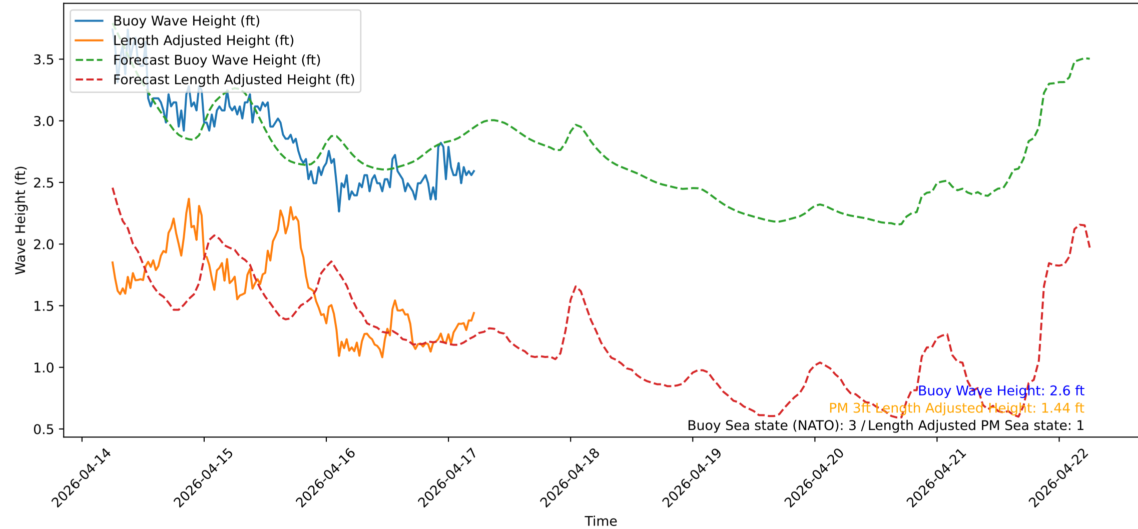
Wave Heights over Time for Red Beach at 2026-04-17 05:50:52
