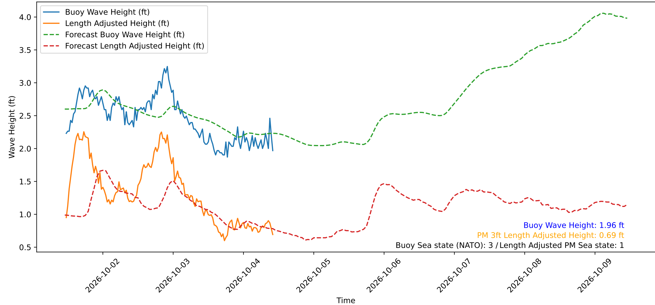
Wave Heights over Time for Red Beach at 2026-10-04 11:00:49
