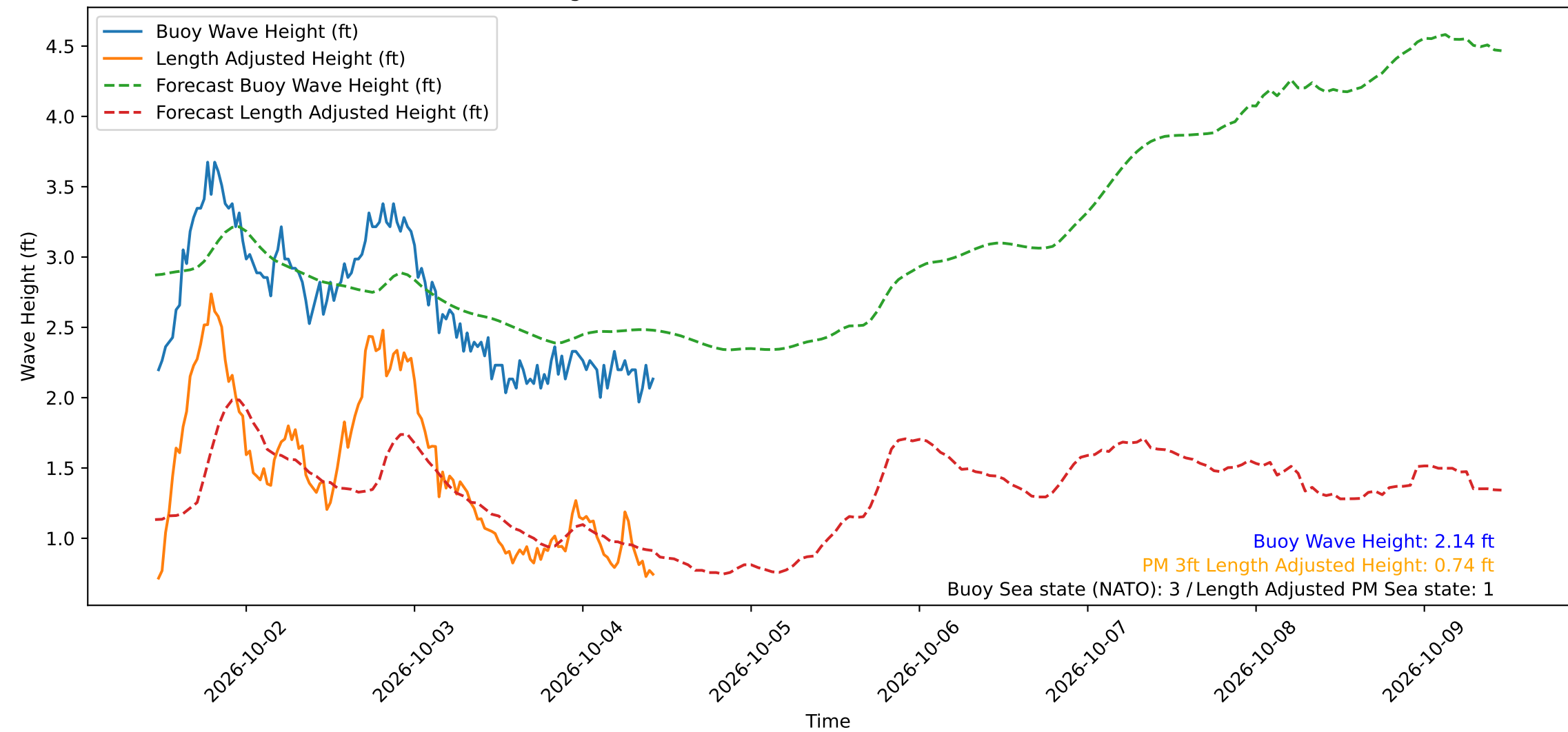
Wave Heights over Time for Green Beach at 2026-10-04 11:01:11
