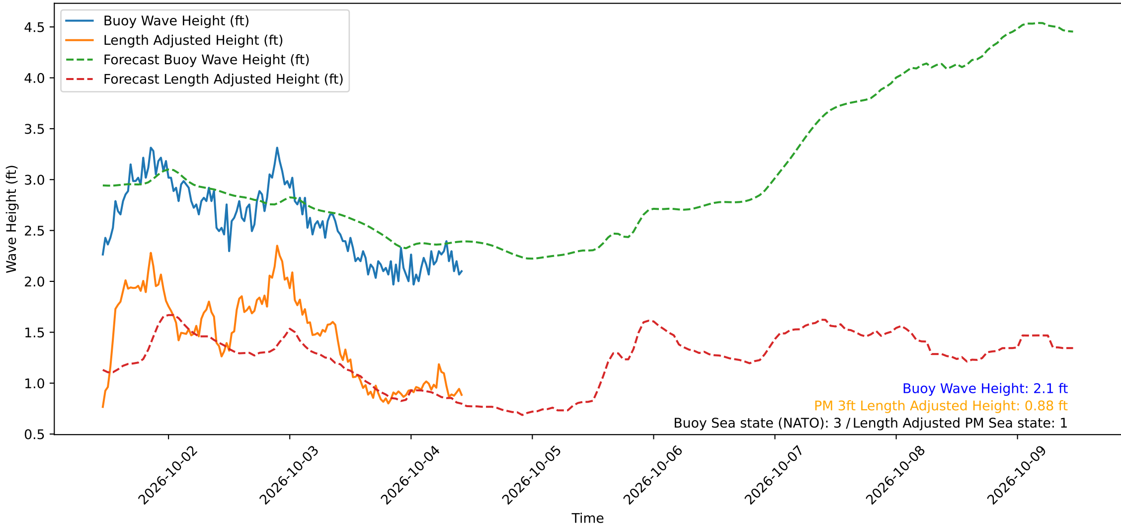
Wave Heights over Time for Oceanside Harbor at 2026-10-04 11:00:29
