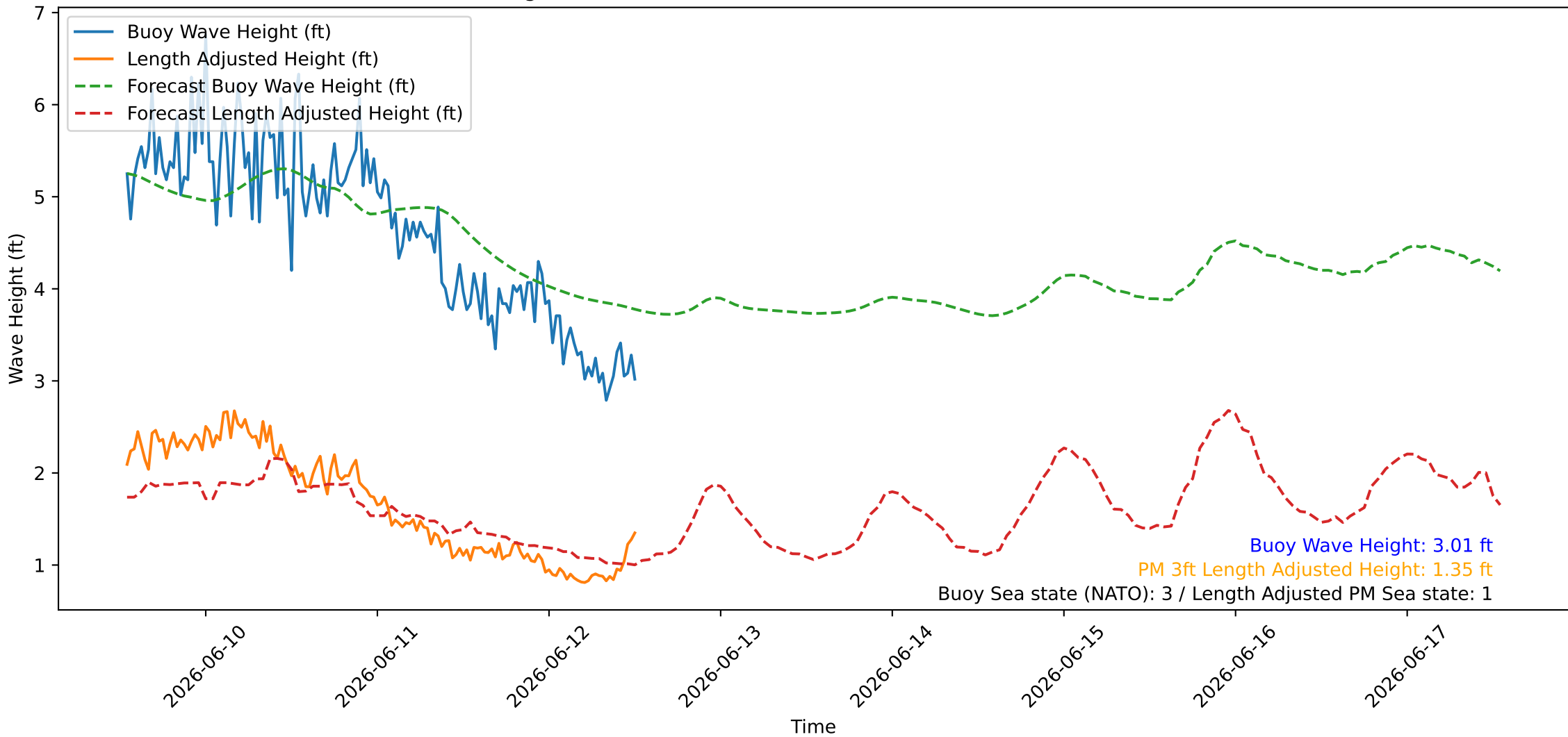
Wave Heights over Time for Oceanside Harbor at 2026-06-12 12:50:26
