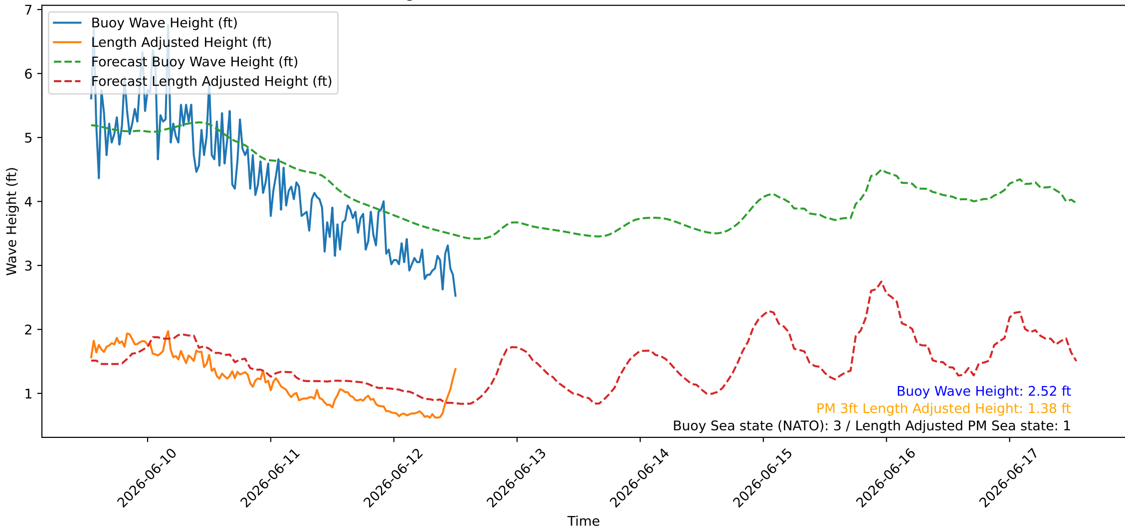
Wave Heights over Time for Red Beach at 2026-06-12 12:50:47
