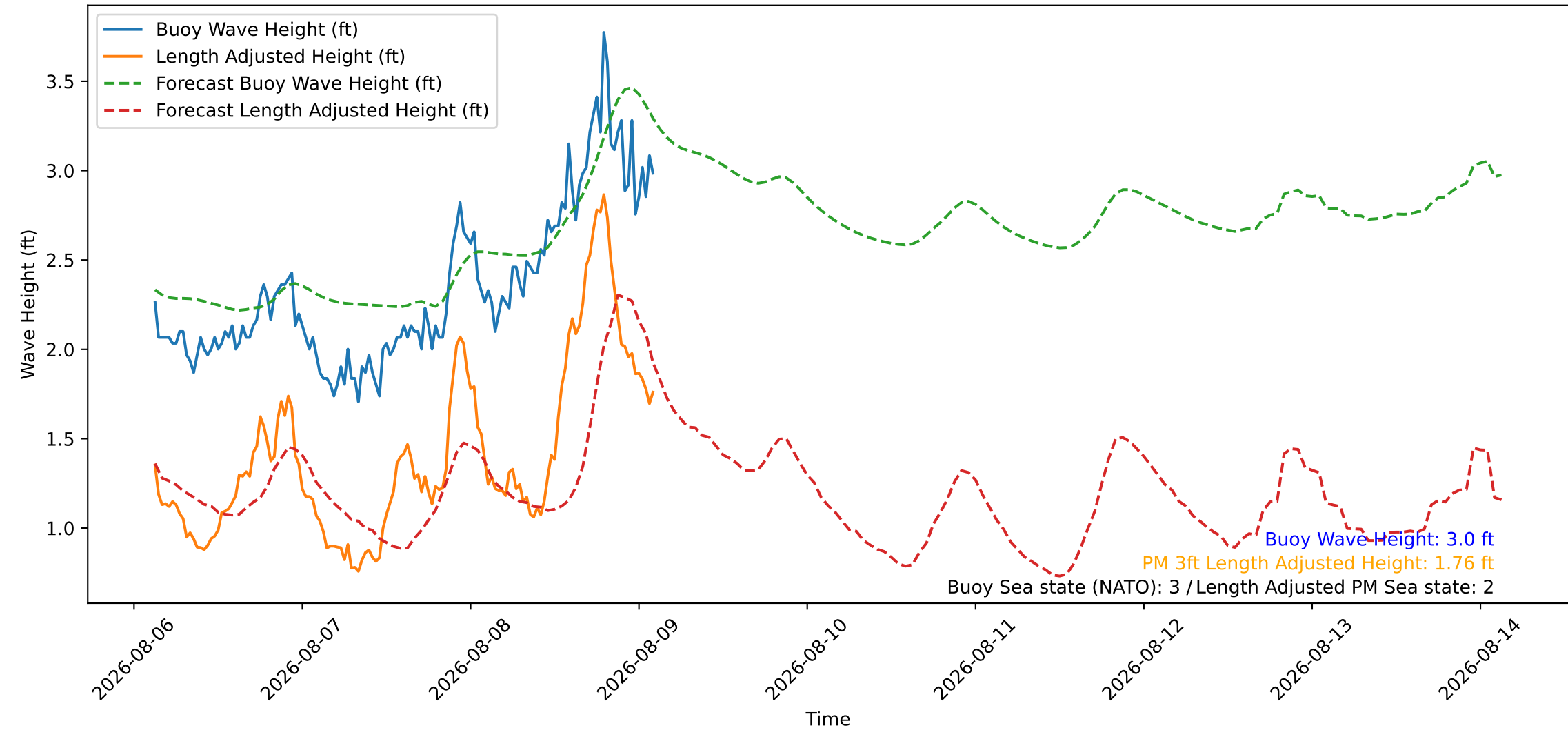
Wave Heights over Time for Green Beach at 2026-08-09 02:51:09
