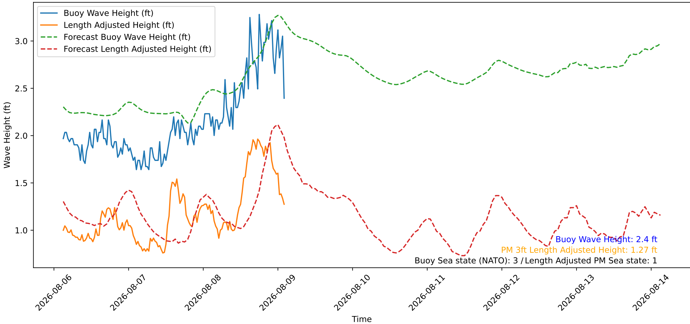
Wave Heights over Time for Oceanside Harbor at 2026-08-09 02:50:27
