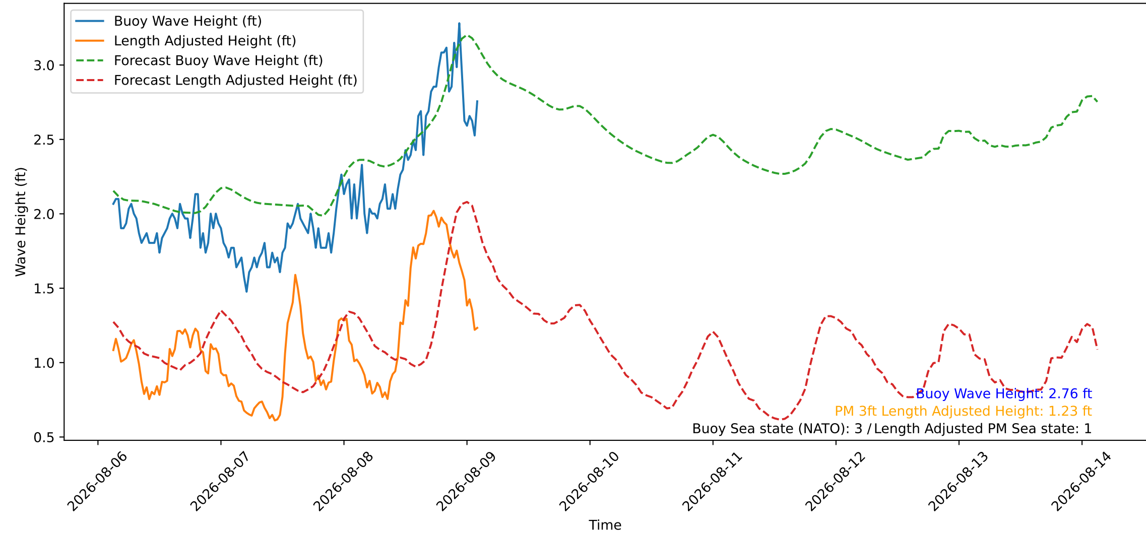
Wave Heights over Time for Red Beach at 2026-08-09 02:50:47
