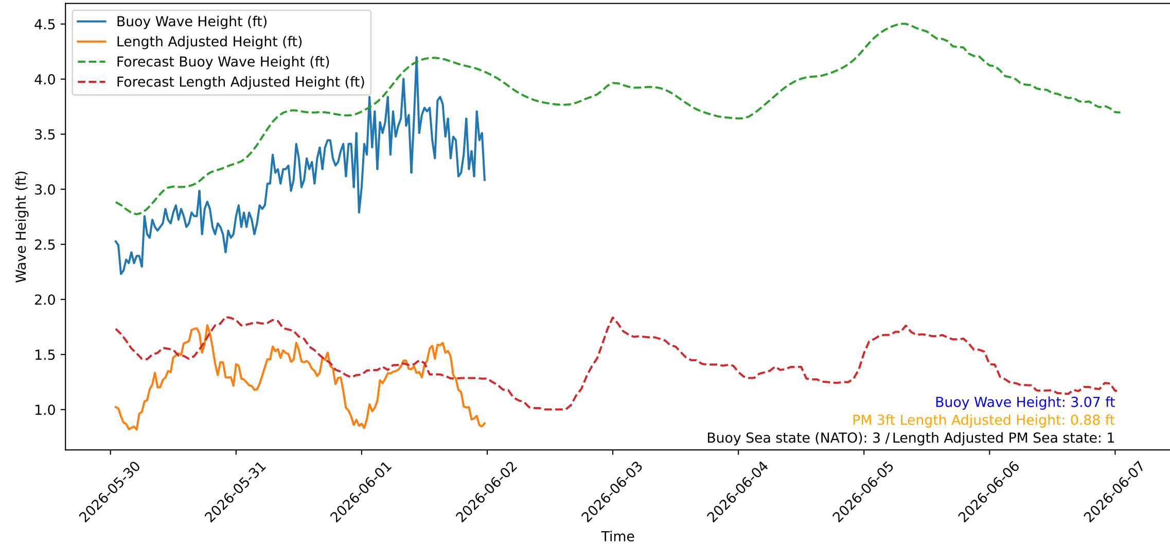
Wave Heights over Time for Red Beach at 2026-06-02 00:30:45
