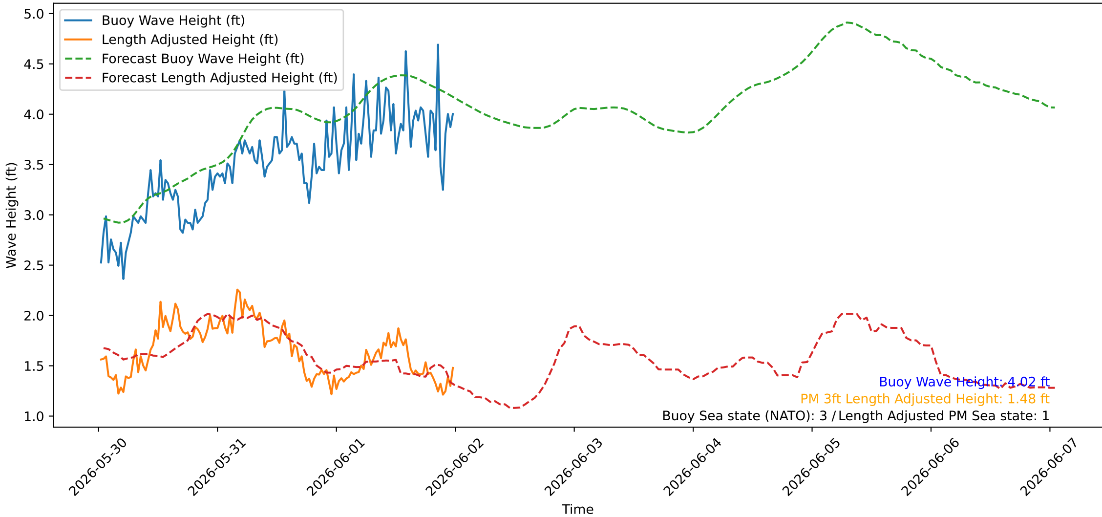
Wave Heights over Time for Oceanside Harbor at 2026-06-02 00:30:25
