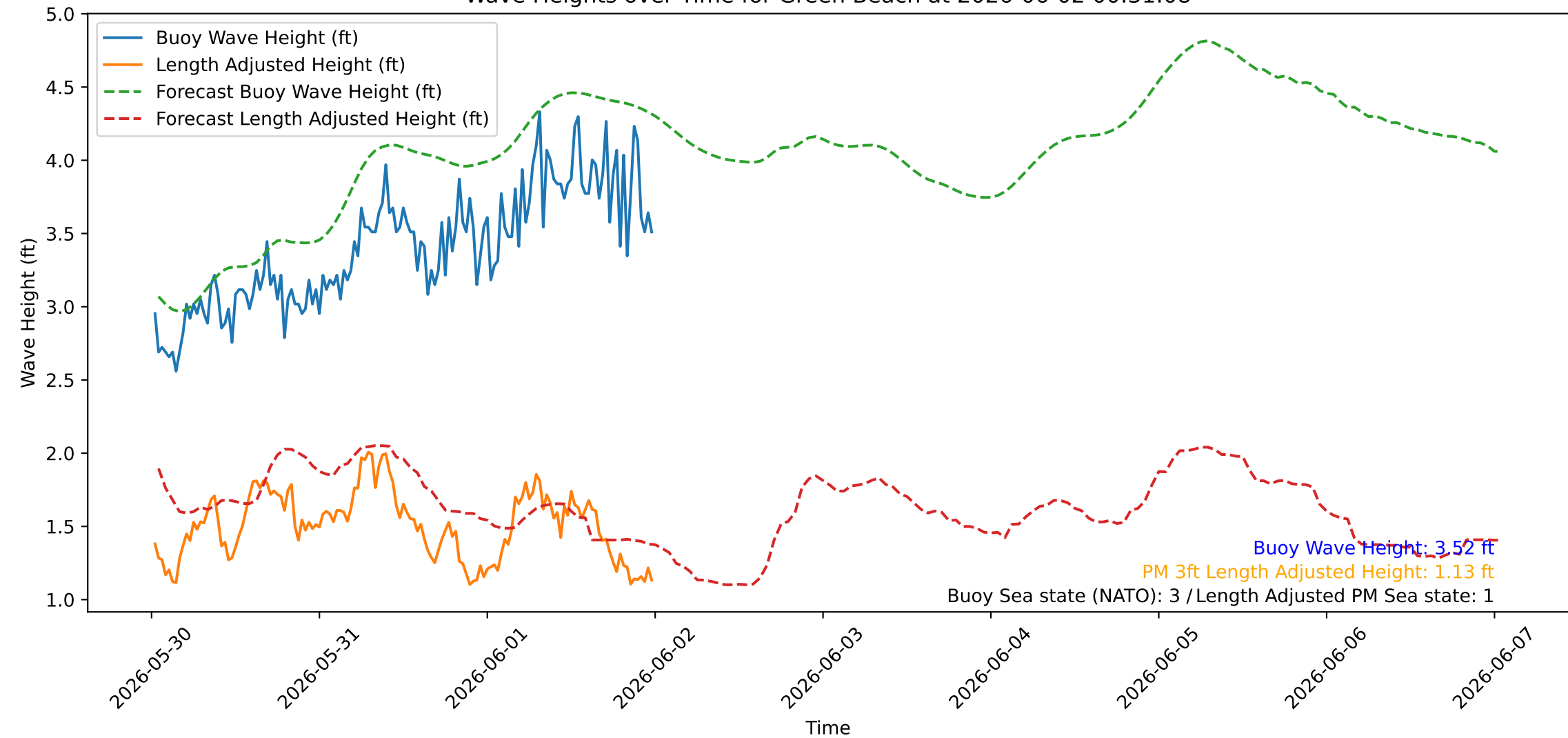
Wave Heights over Time for Green Beach at 2026-06-02 00:31:08
