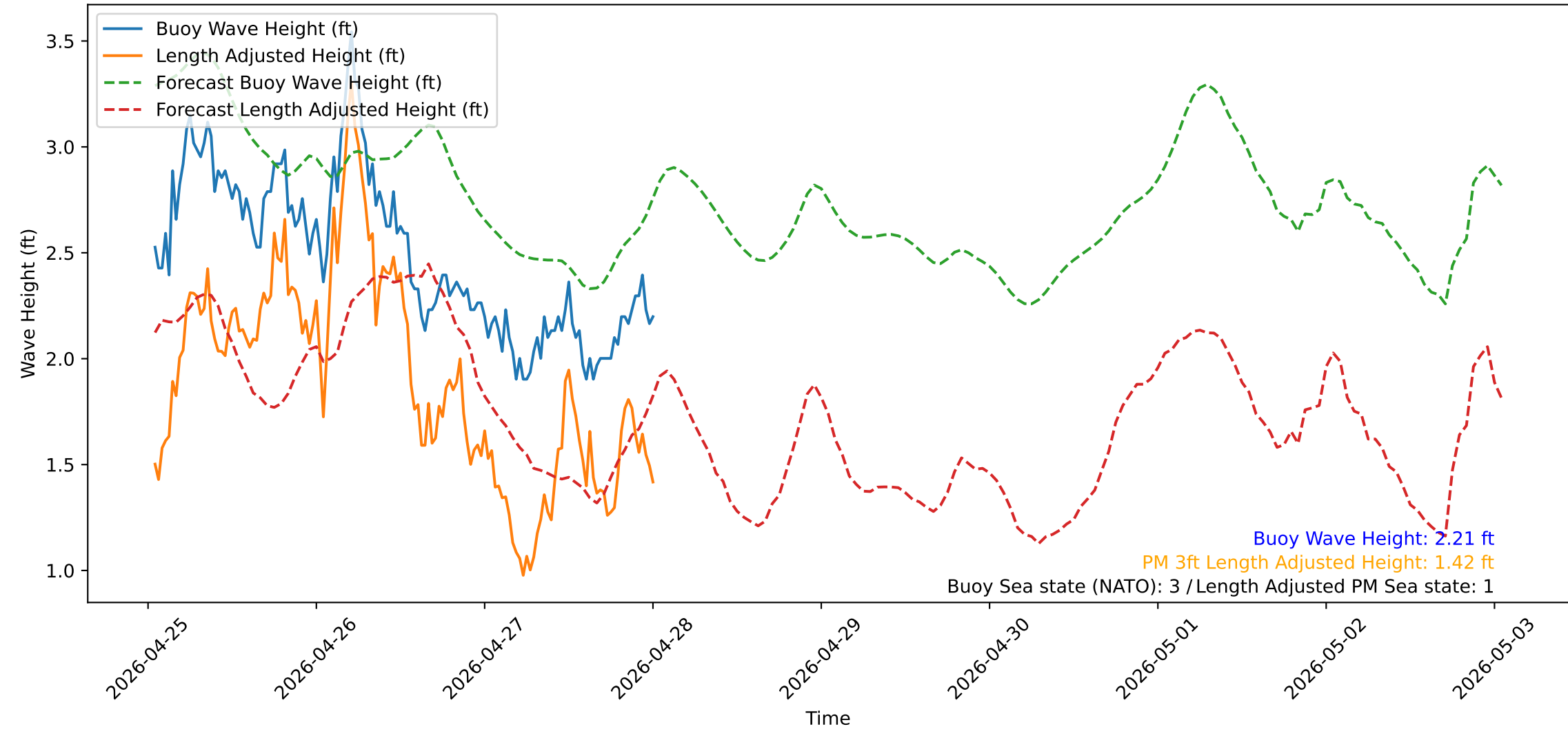
Wave Heights over Time for Red Beach at 2026-04-28 00:50:51
