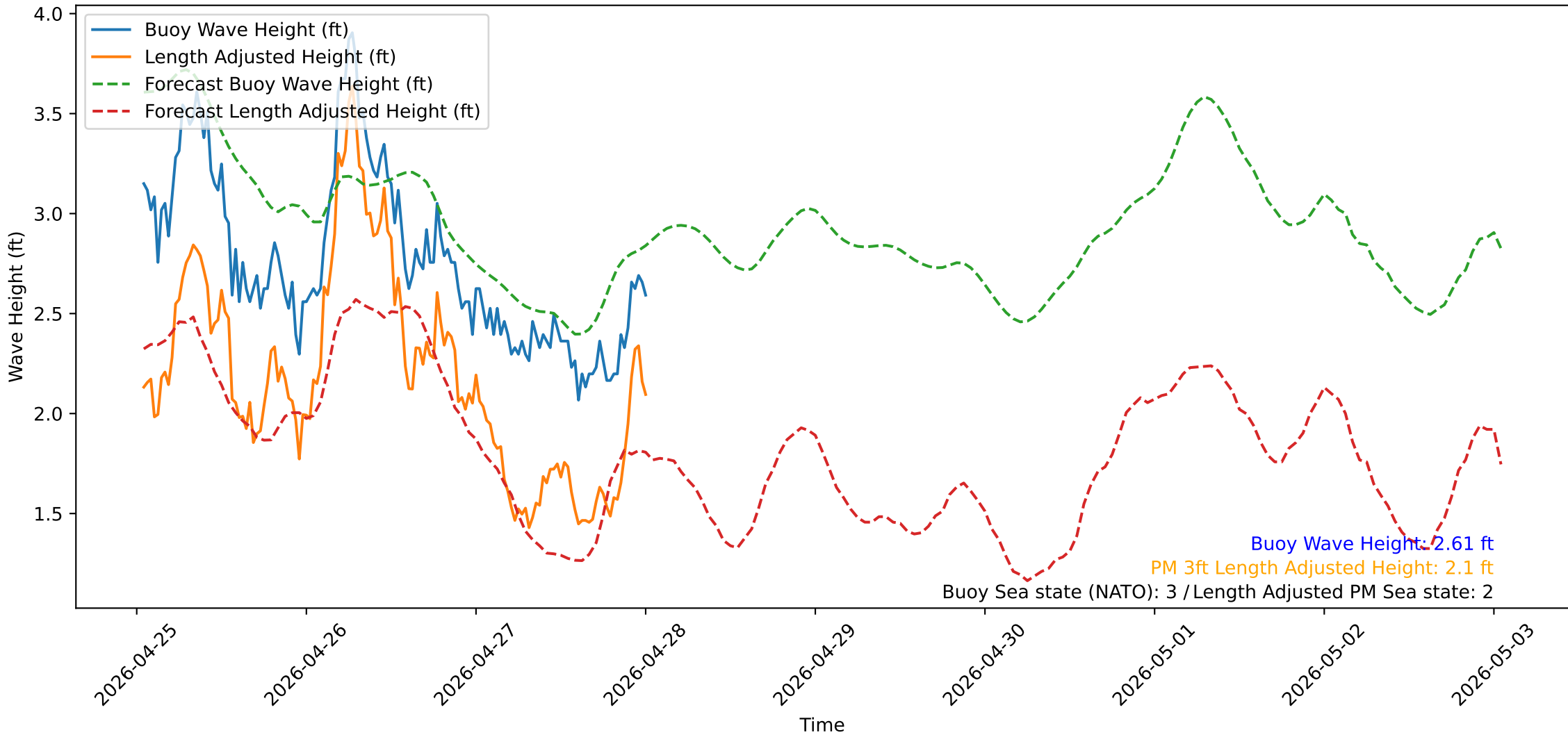
Wave Heights over Time for Oceanside Harbor at 2026-04-28 00:50:30
