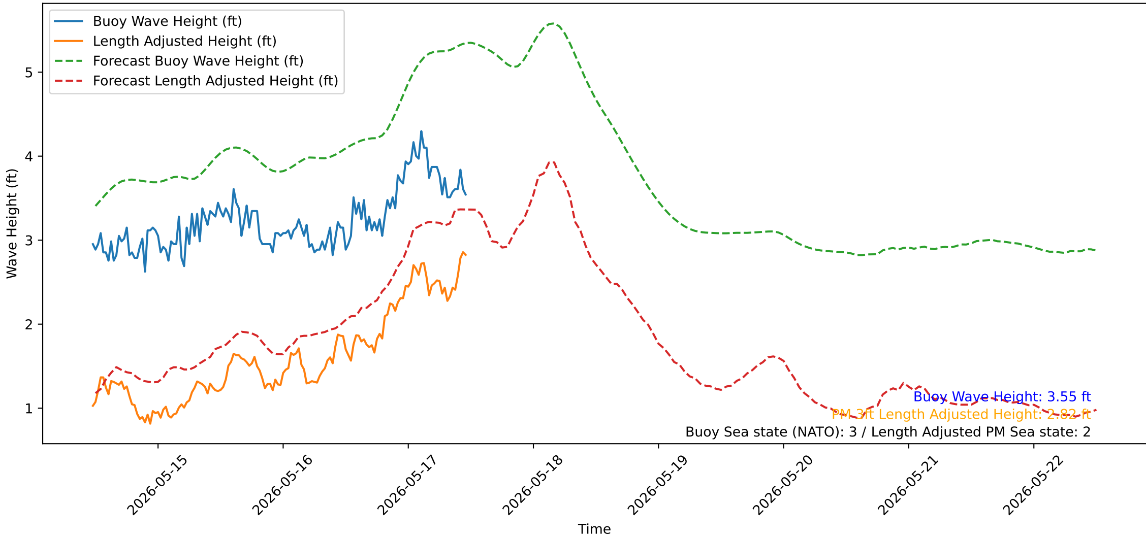
Wave Heights over Time for Oceanside Harbor at 2026-05-17 11:40:32
