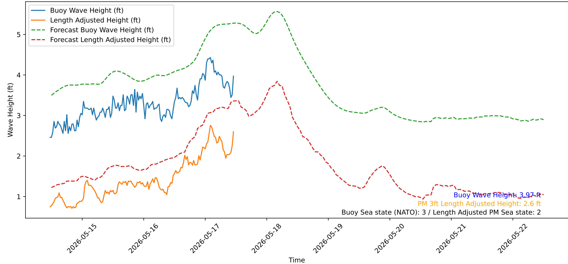
Wave Heights over Time for Green Beach at 2026-05-17 11:41:14
