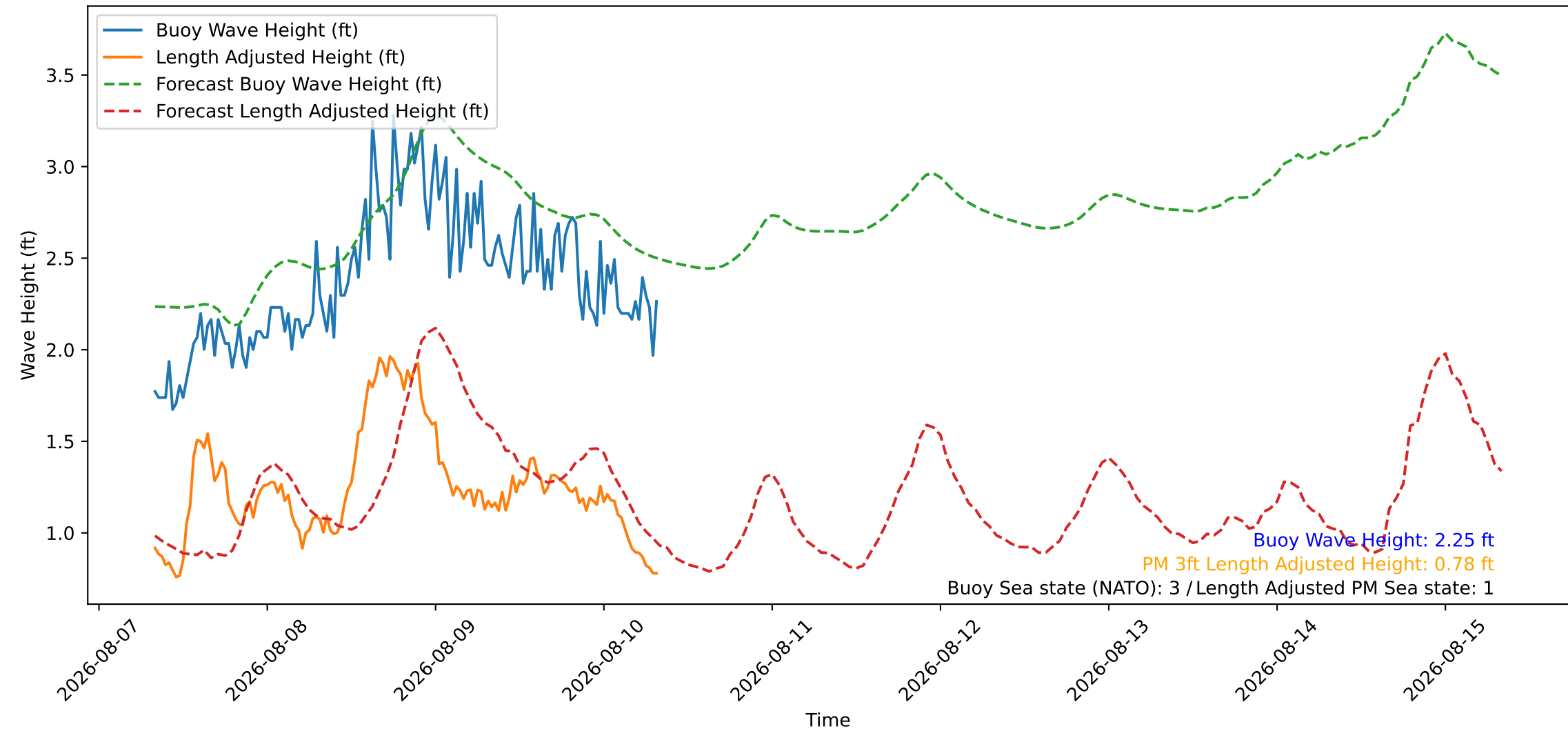
Wave Heights over Time for Oceanside Harbor at 2026-08-10 08:10:26
