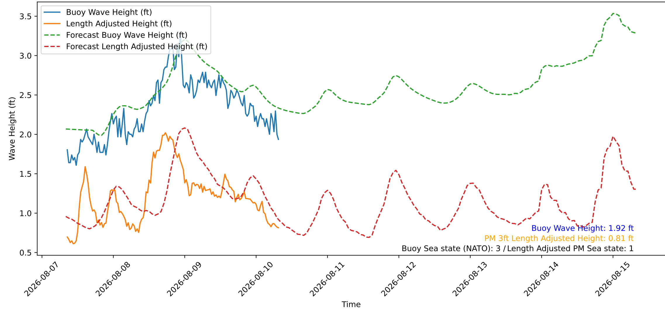
Wave Heights over Time for Red Beach at 2026-08-10 08:10:46
