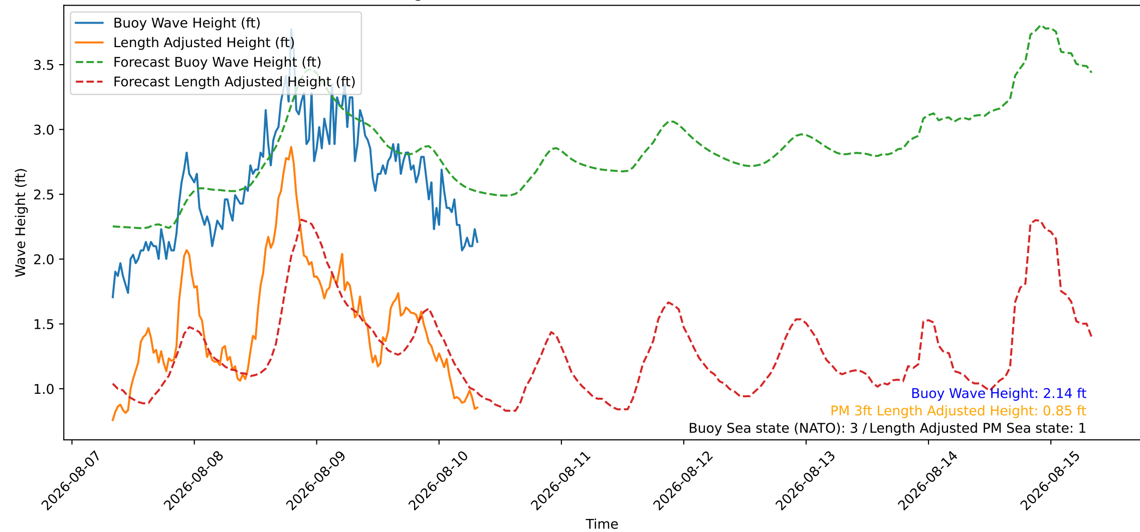
Wave Heights over Time for Green Beach at 2026-08-10 08:11:09
