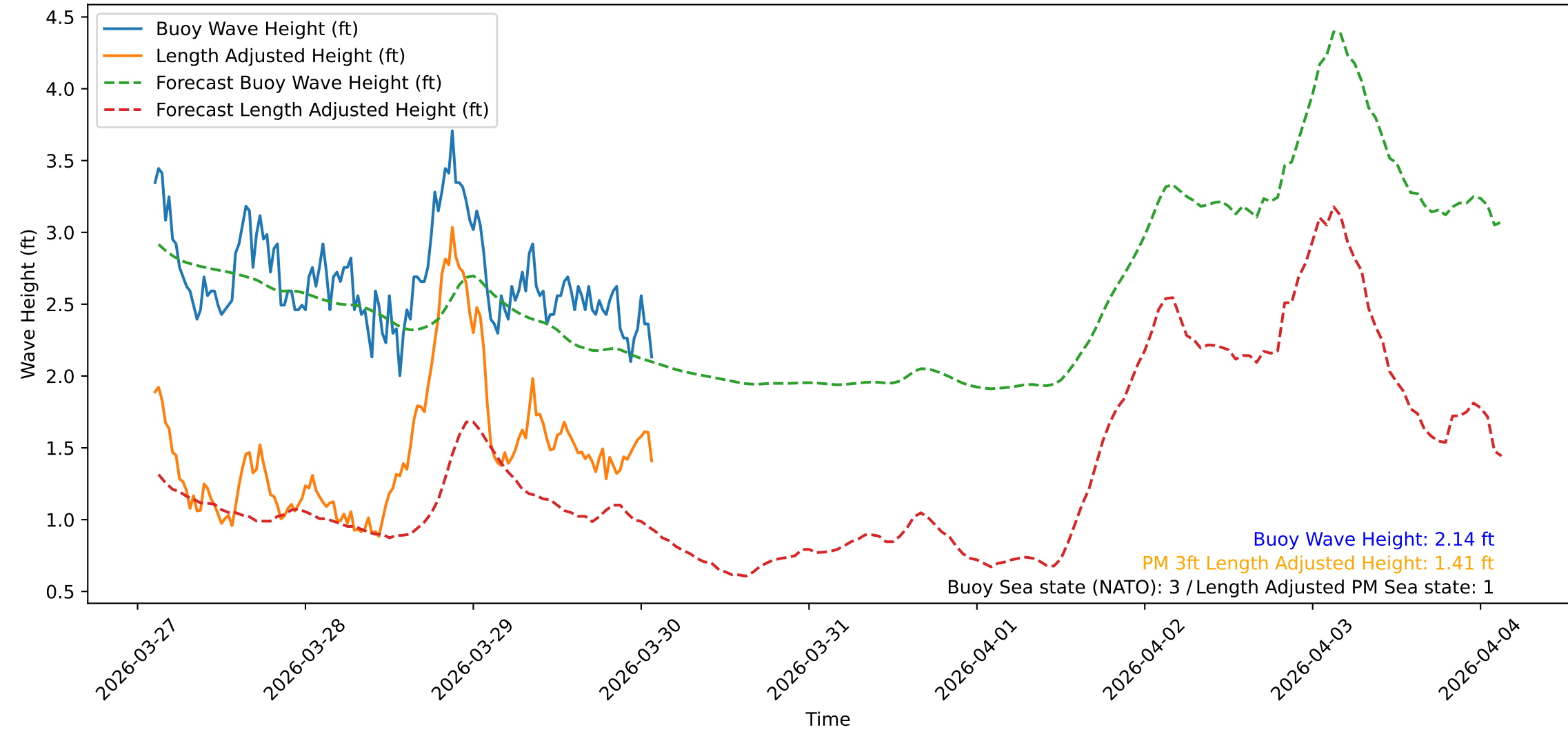
Wave Heights over Time for Green Beach at 2026-03-30 02:31:10
