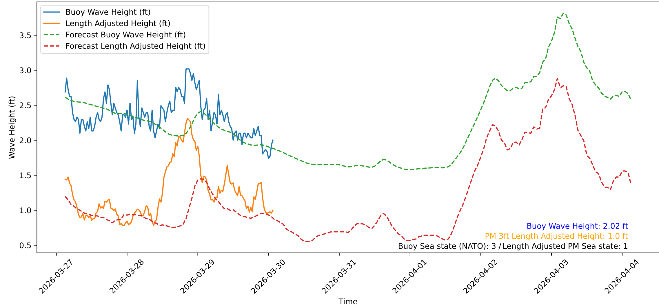
Wave Heights over Time for Red Beach at 2026-03-30 02:30:48
