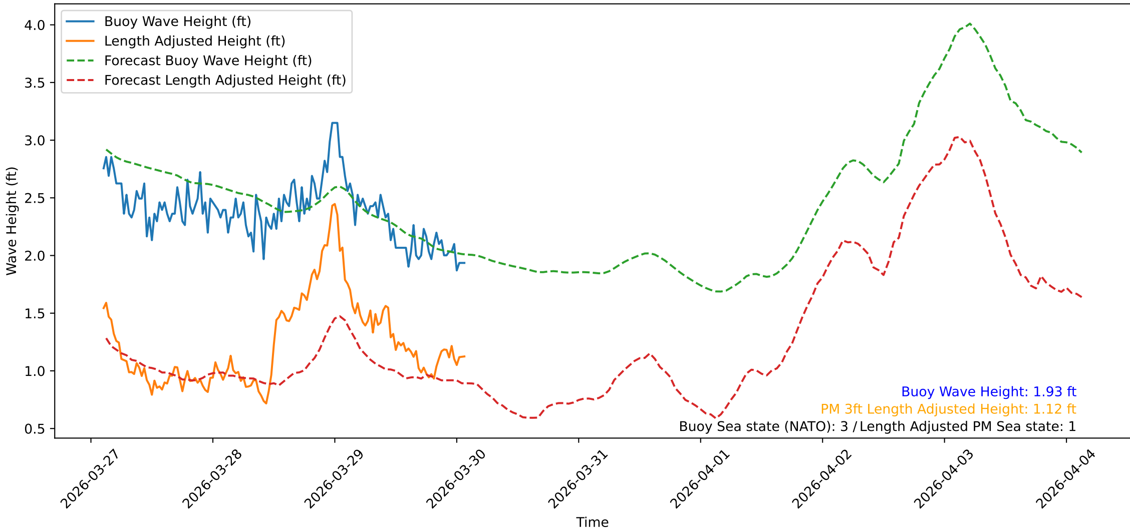
Wave Heights over Time for Oceanside Harbor at 2026-03-30 02:30:31
