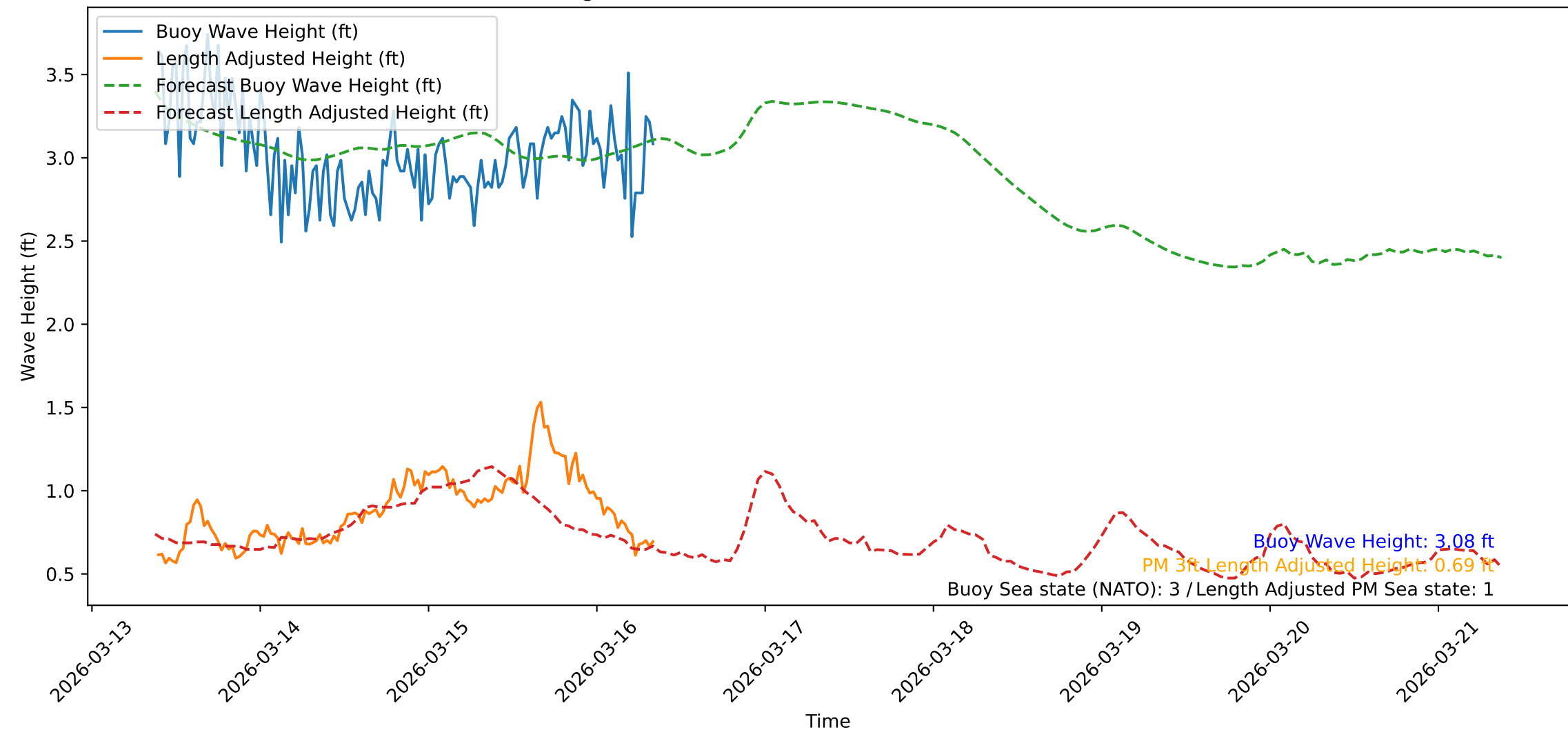
Wave Heights over Time for Red Beach at 2026-03-16 09:01:06
