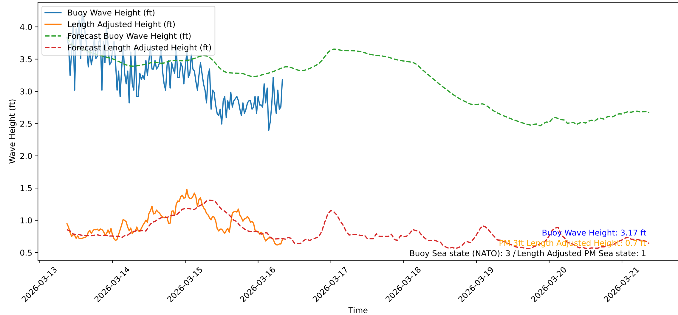
Wave Heights over Time for Oceanside Harbor at 2026-03-16 09:00:43
