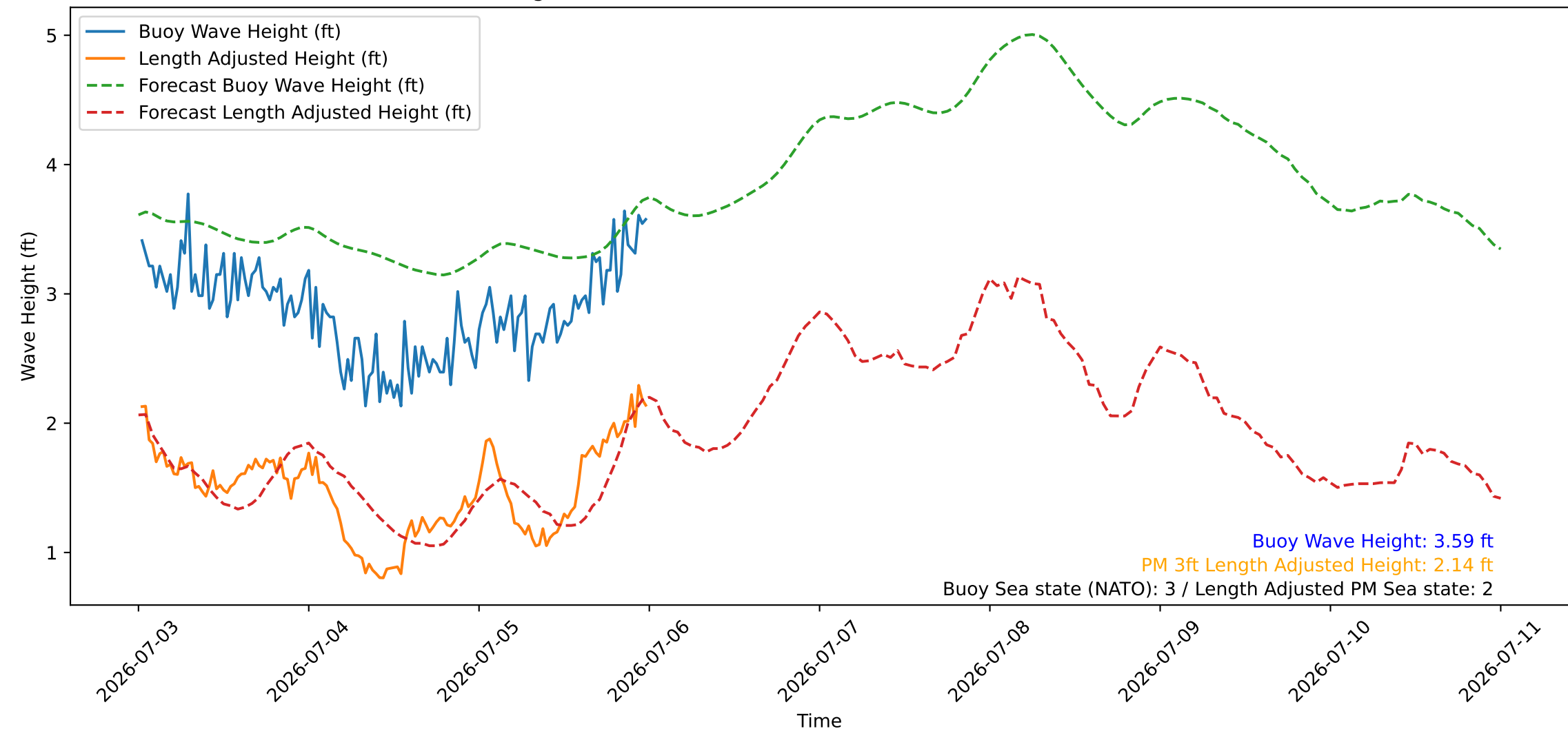
Wave Heights over Time for Oceanside Harbor at 2026-07-06 00:20:26
