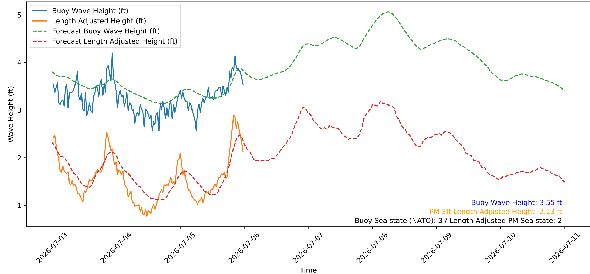
Wave Heights over Time for Green Beach at 2026-07-06 00:21:10
