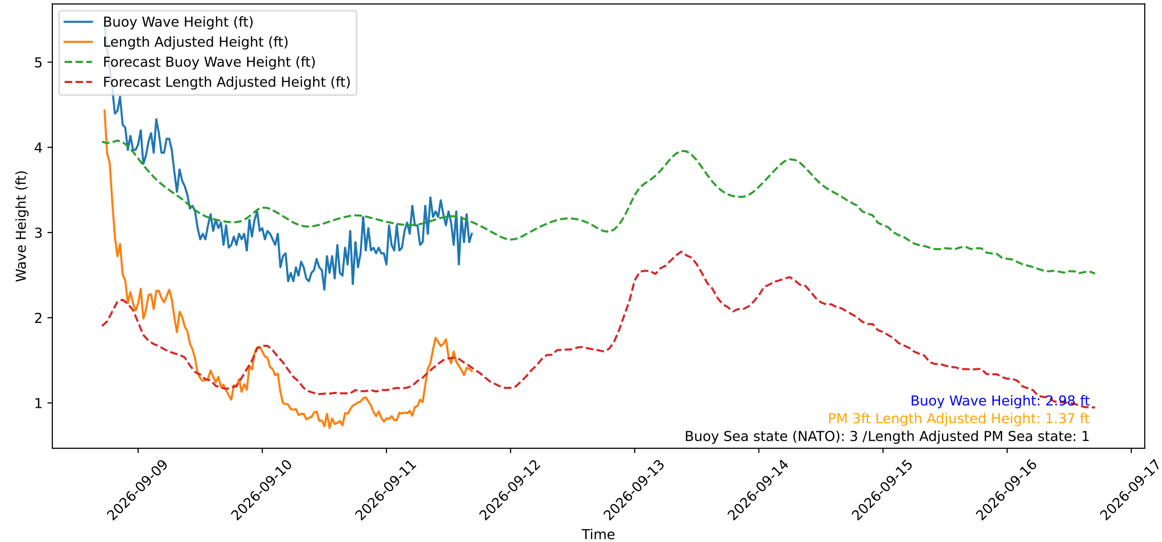
Wave Heights over Time for Red Beach at 2026-09-11 17:20:51
