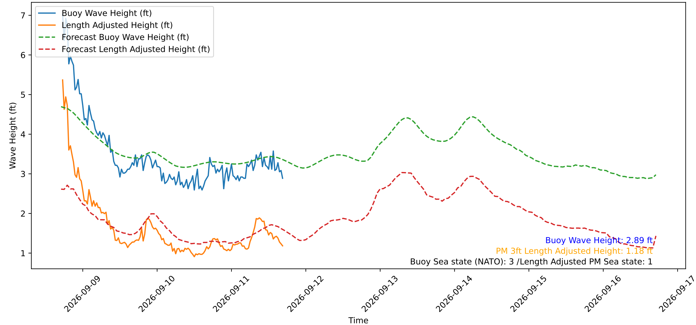
Wave Heights over Time for Green Beach at 2026-09-11 17:21:16
