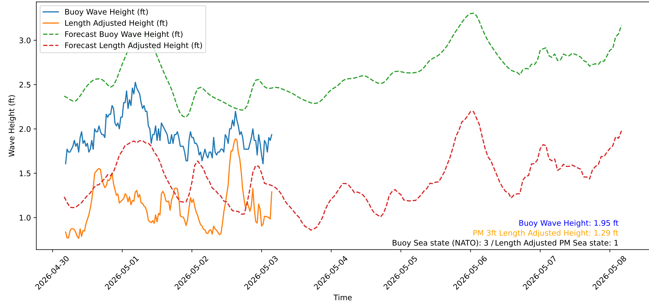
Wave Heights over Time for Red Beach at 2026-05-03 04:10:52
