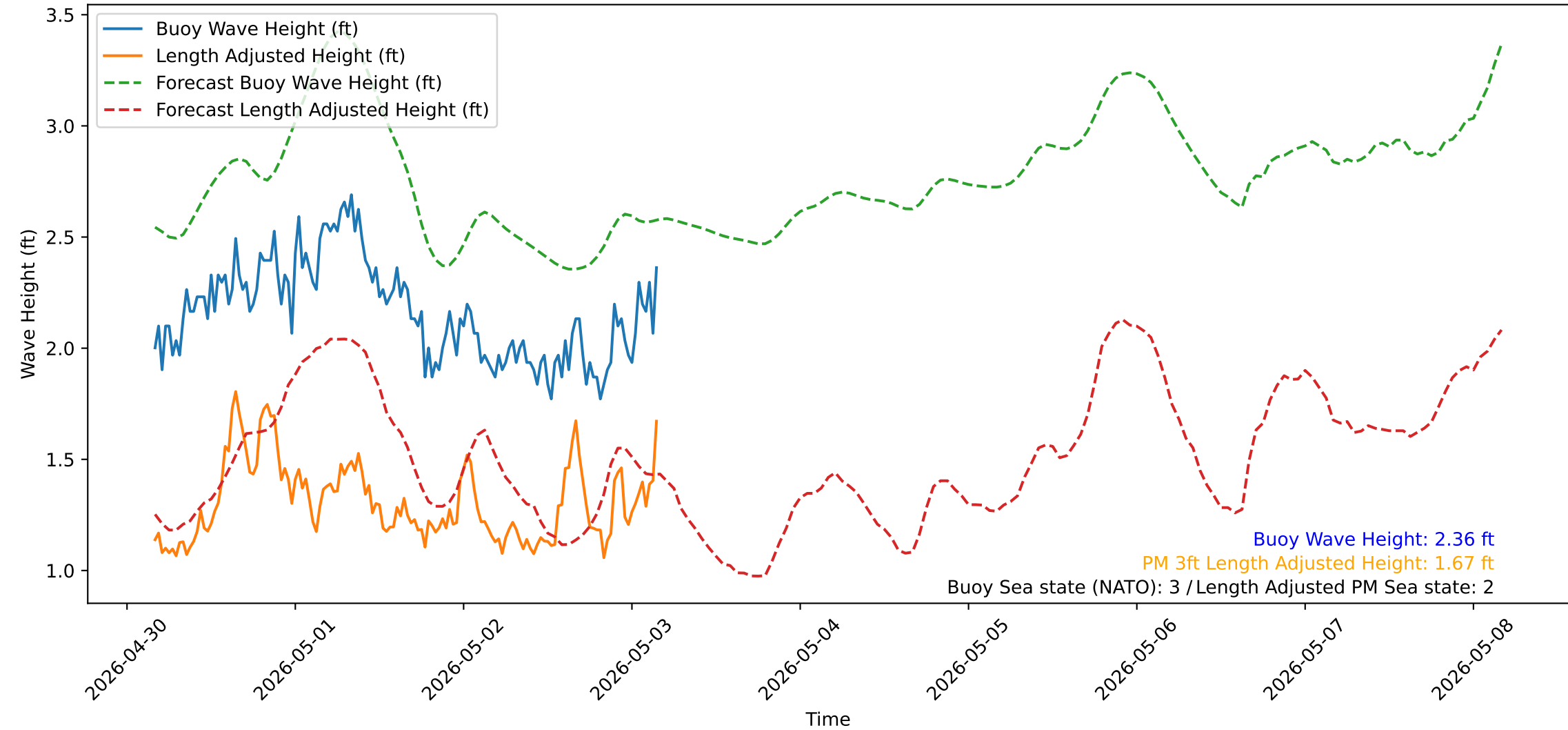
Wave Heights over Time for Oceanside Harbor at 2026-05-03 04:10:32
