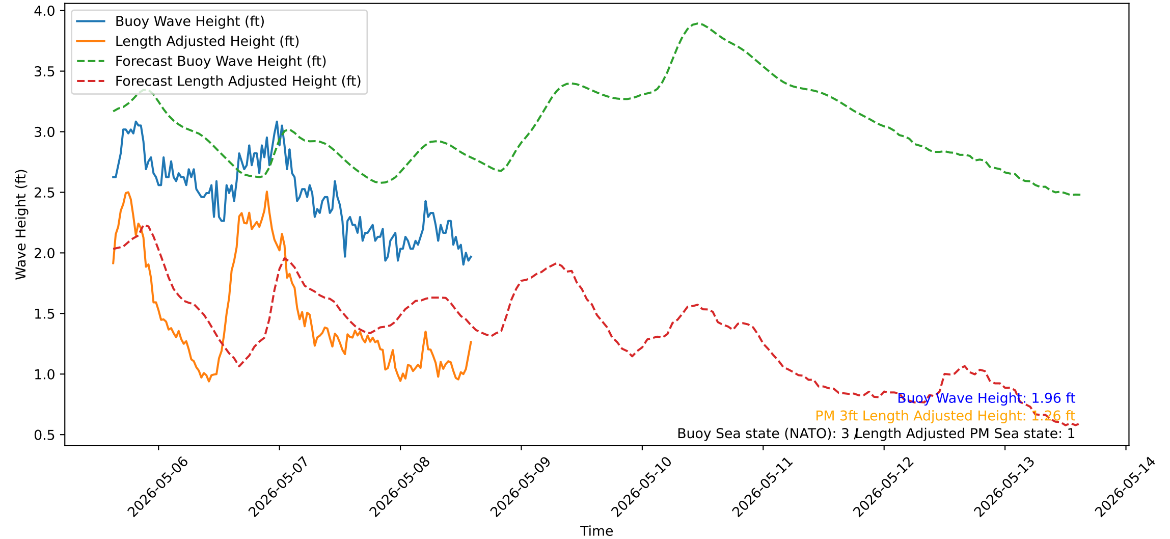
Wave Heights over Time for Red Beach at 2026-05-08 14:50:52
