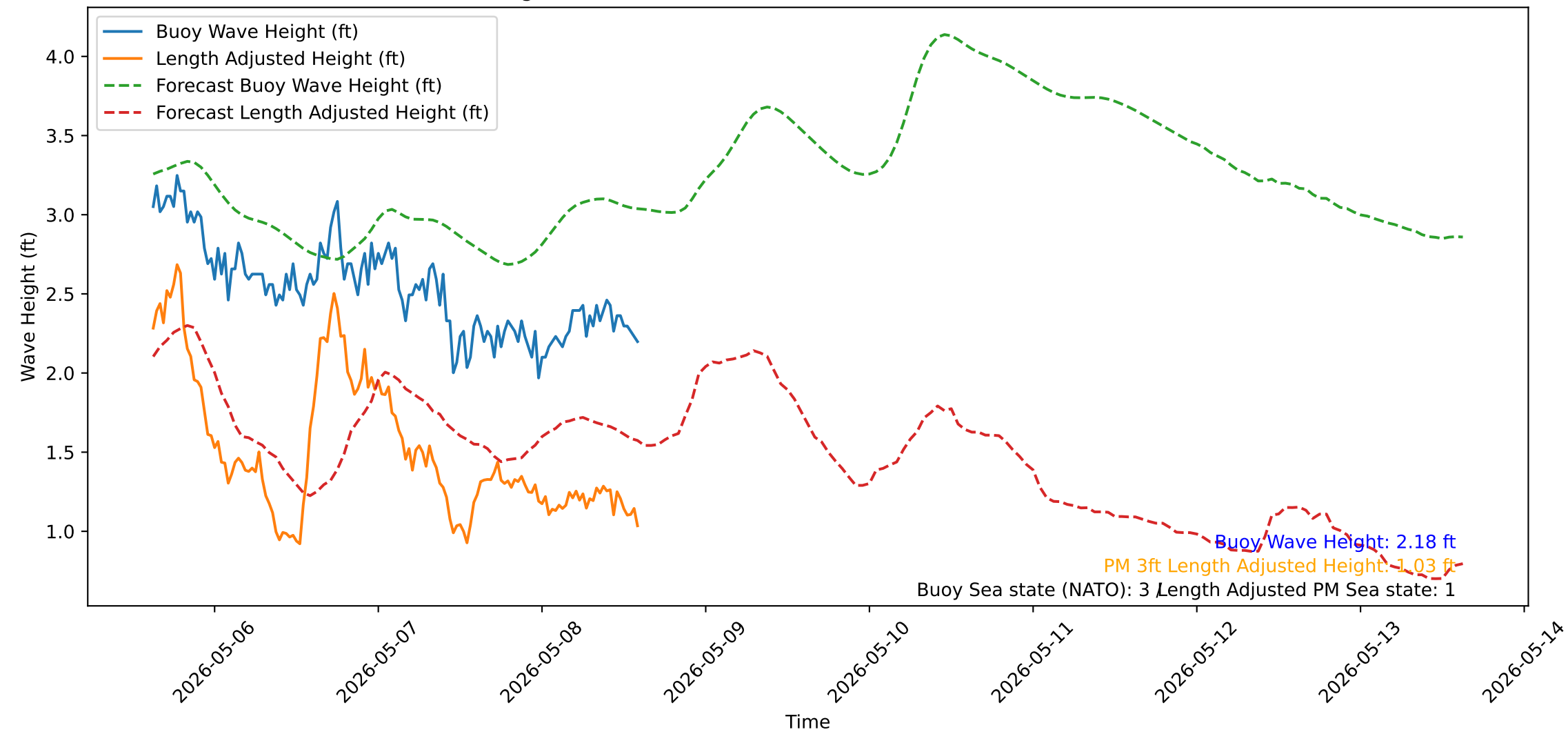
Wave Heights over Time for Oceanside Harbor at 2026-05-08 14:50:31
