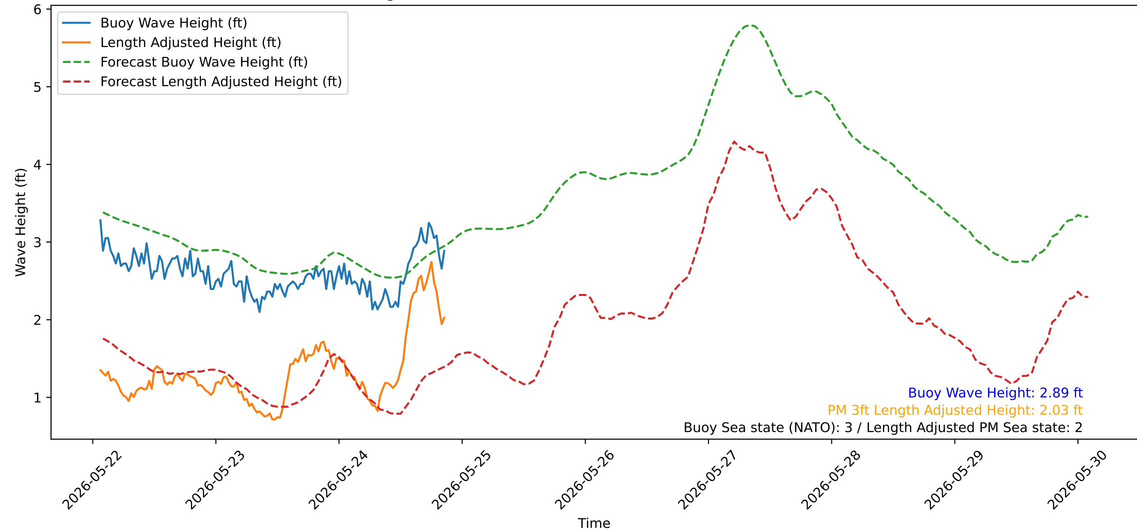
Wave Heights over Time for Oceanside Harbor at 2026-05-25 01:30:31
