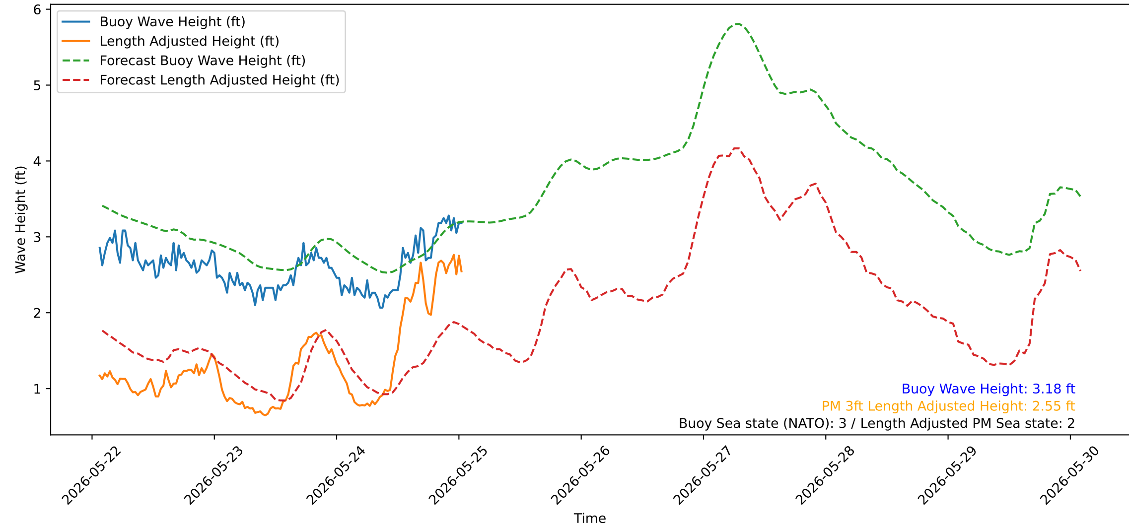
Wave Heights over Time for Green Beach at 2026-05-25 01:31:14
