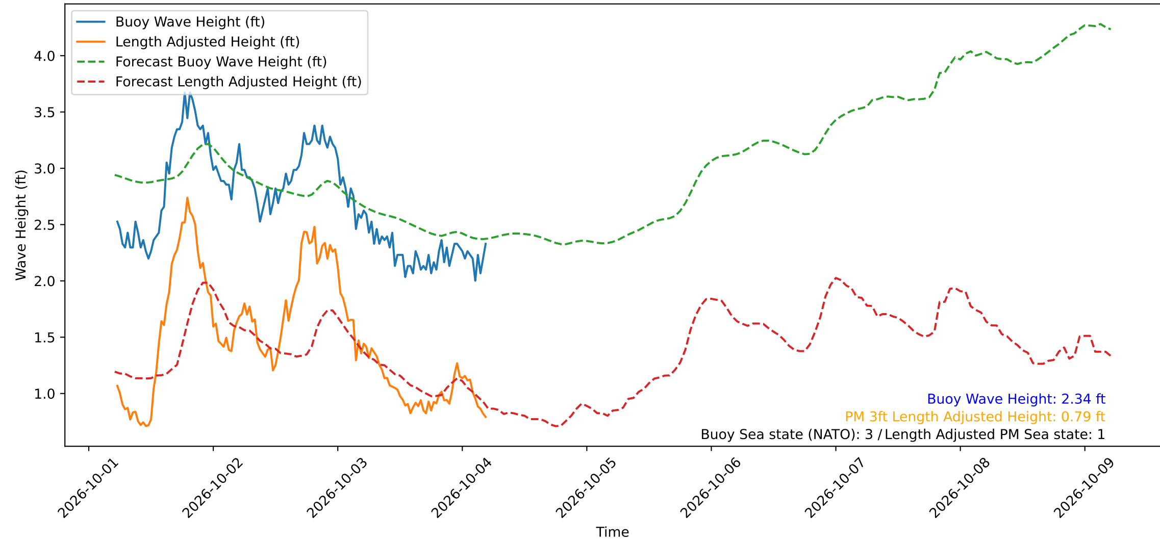
Wave Heights over Time for Green Beach at 2026-10-04 05:21:14
