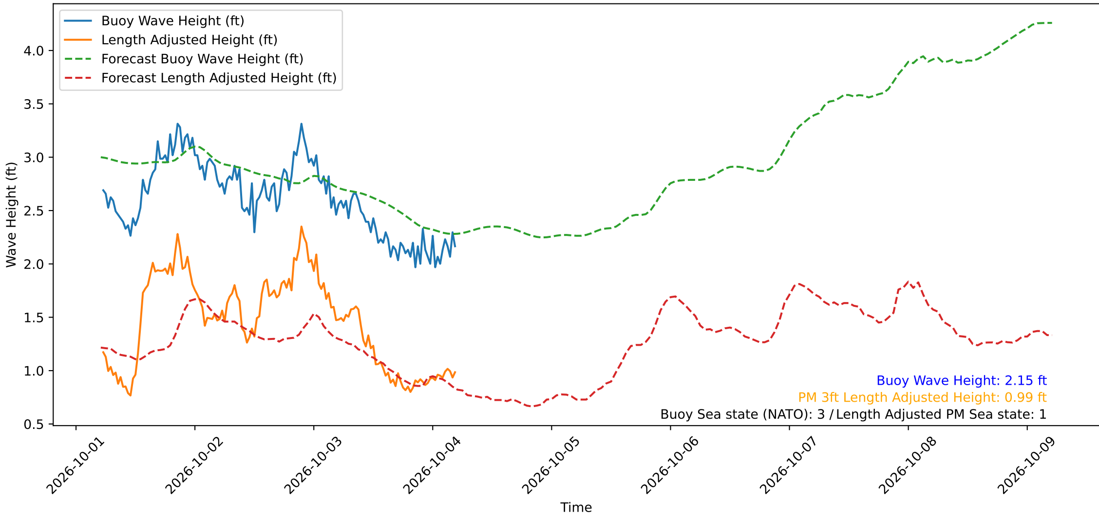
Wave Heights over Time for Oceanside Harbor at 2026-10-04 05:20:29
