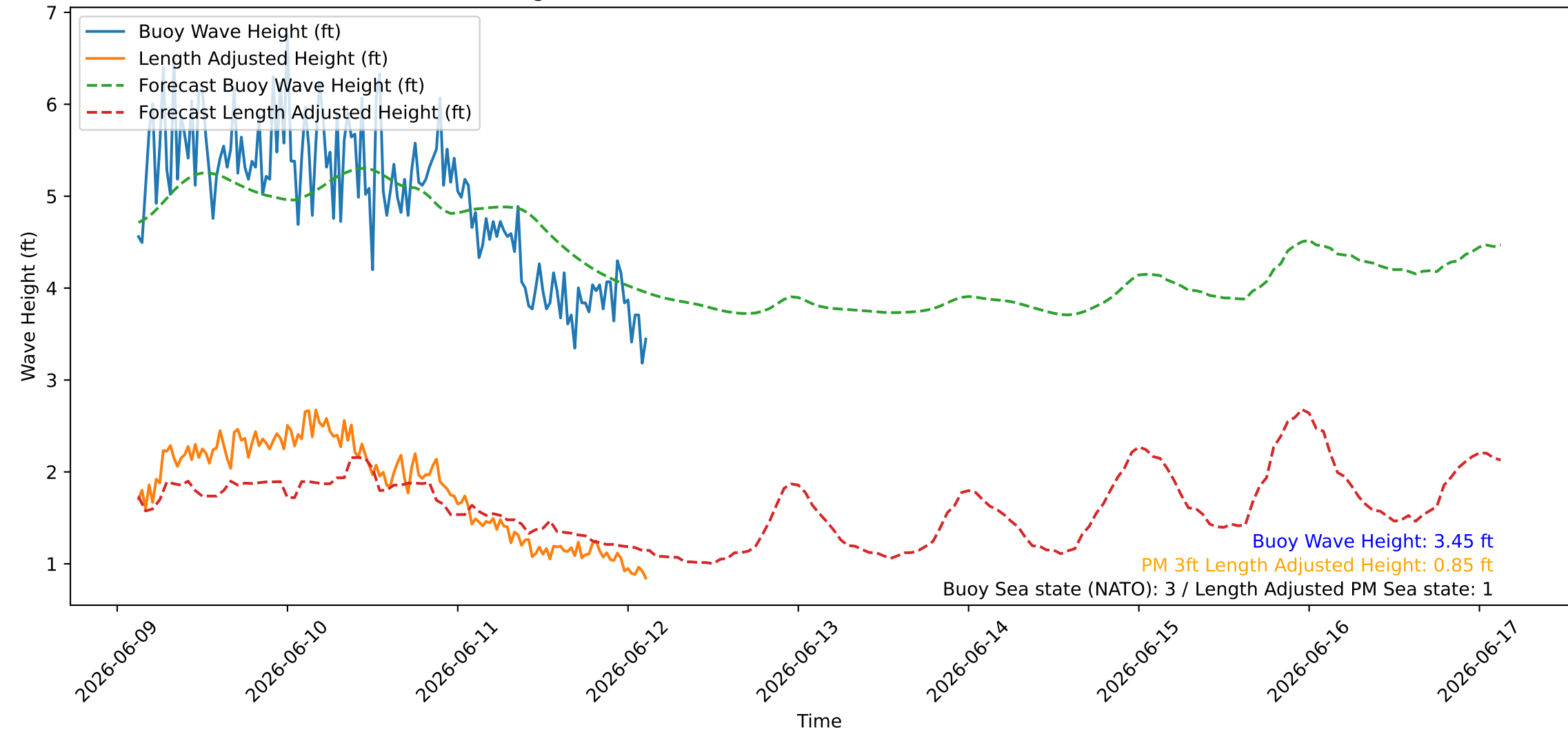
Wave Heights over Time for Oceanside Harbor at 2026-06-12 03:10:27
