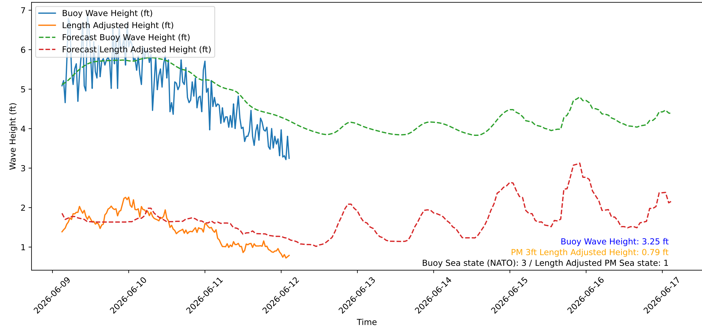
Wave Heights over Time for Green Beach at 2026-06-12 03:11:09
