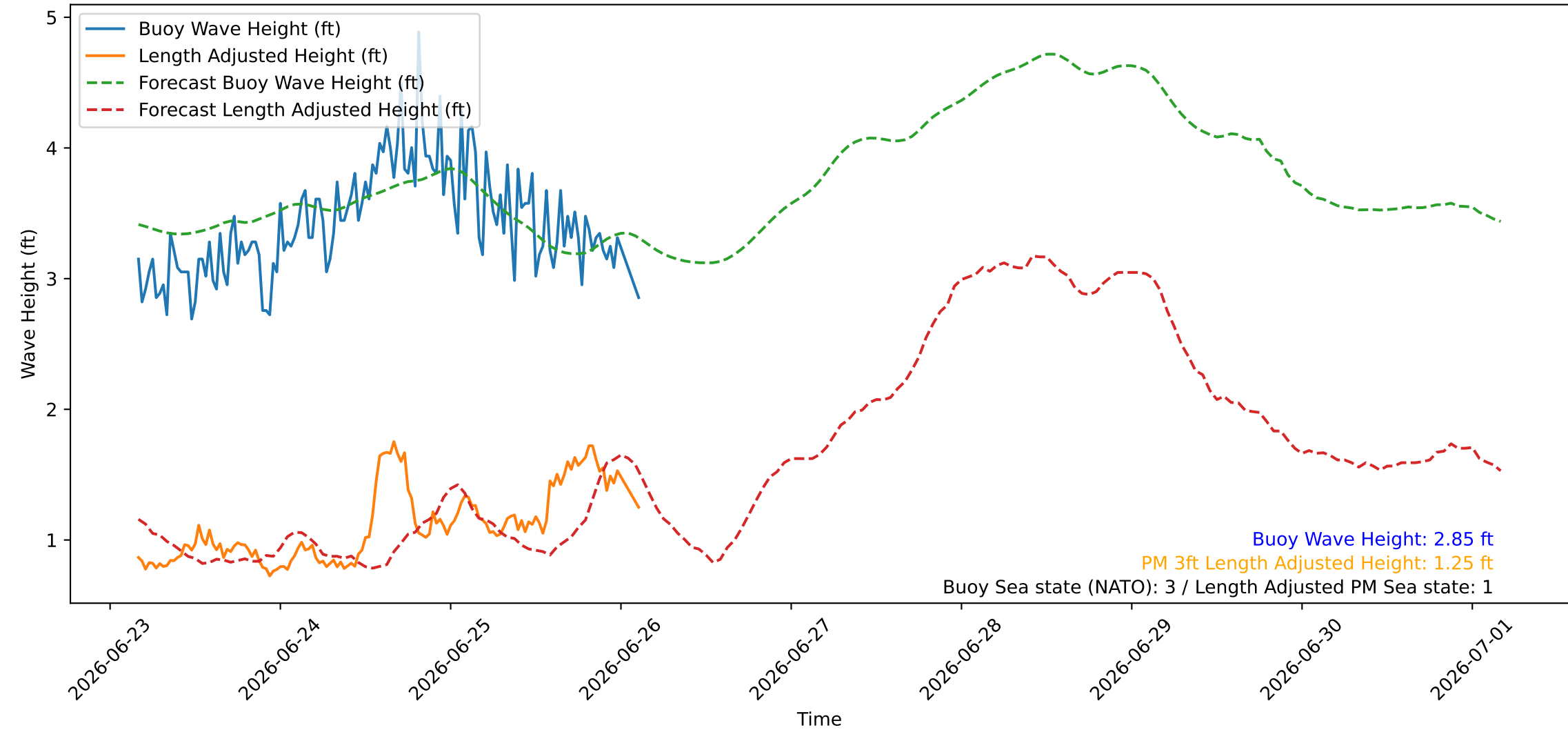
Wave Heights over Time for Oceanside Harbor at 2026-06-26 03:50:25
