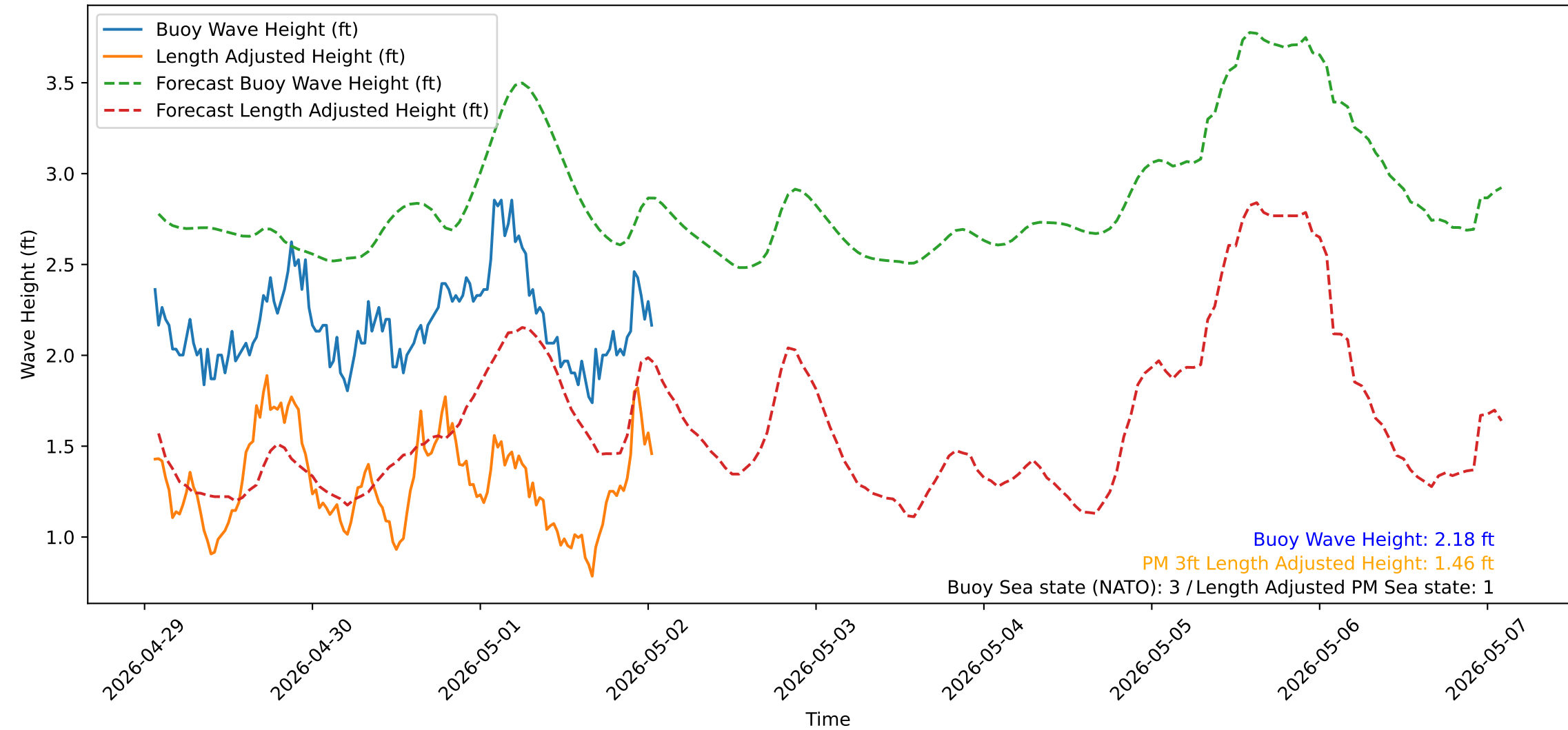
Wave Heights over Time for Green Beach at 2026-05-02 01:31:13
