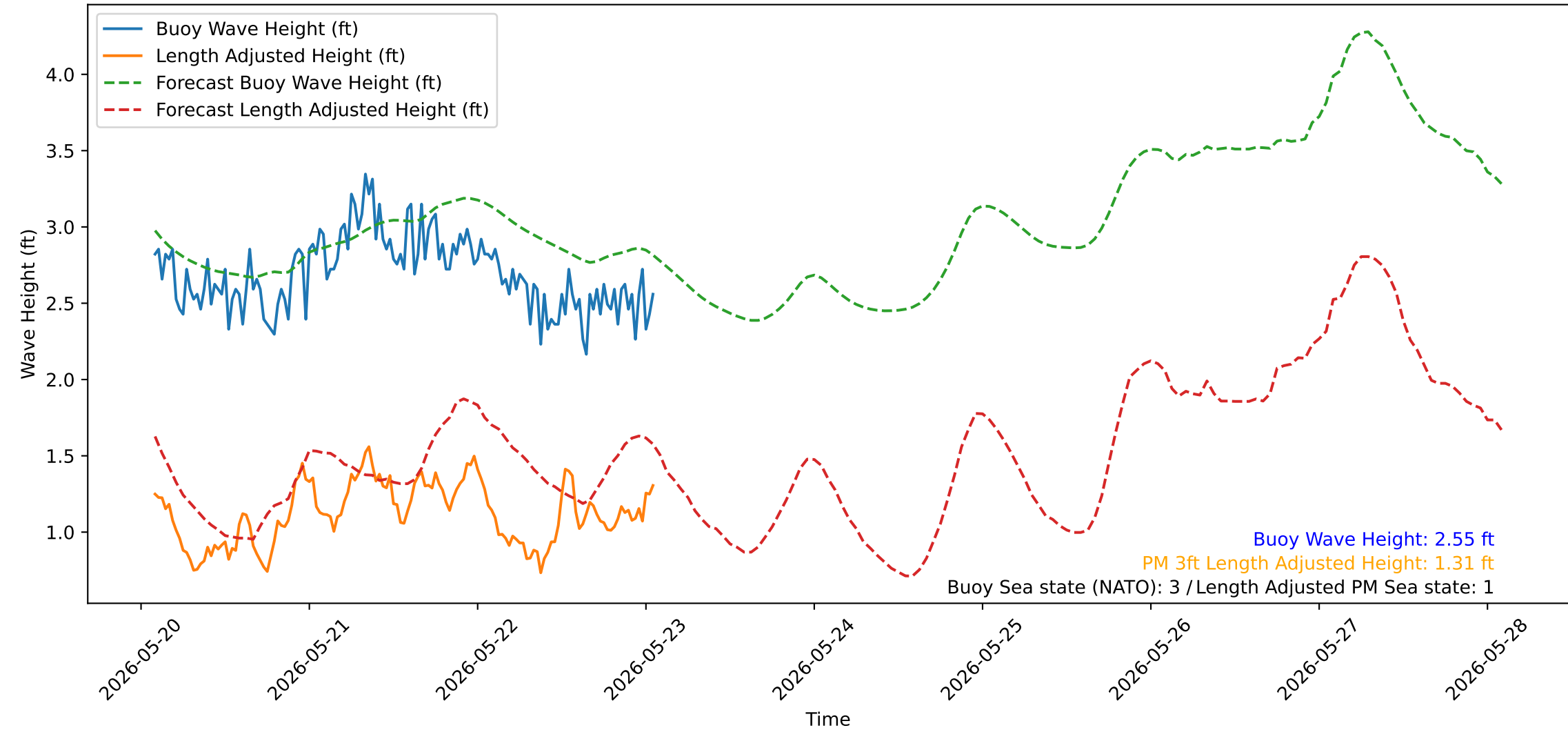
Wave Heights over Time for Red Beach at 2026-05-23 01:50:53
